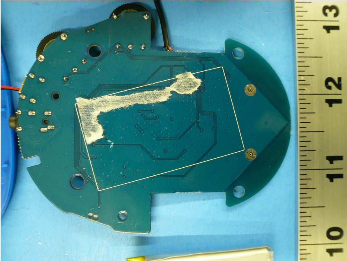
Figure 3: Internal Photo of Ear Force Stealth 520 RX without battery- Bottom
