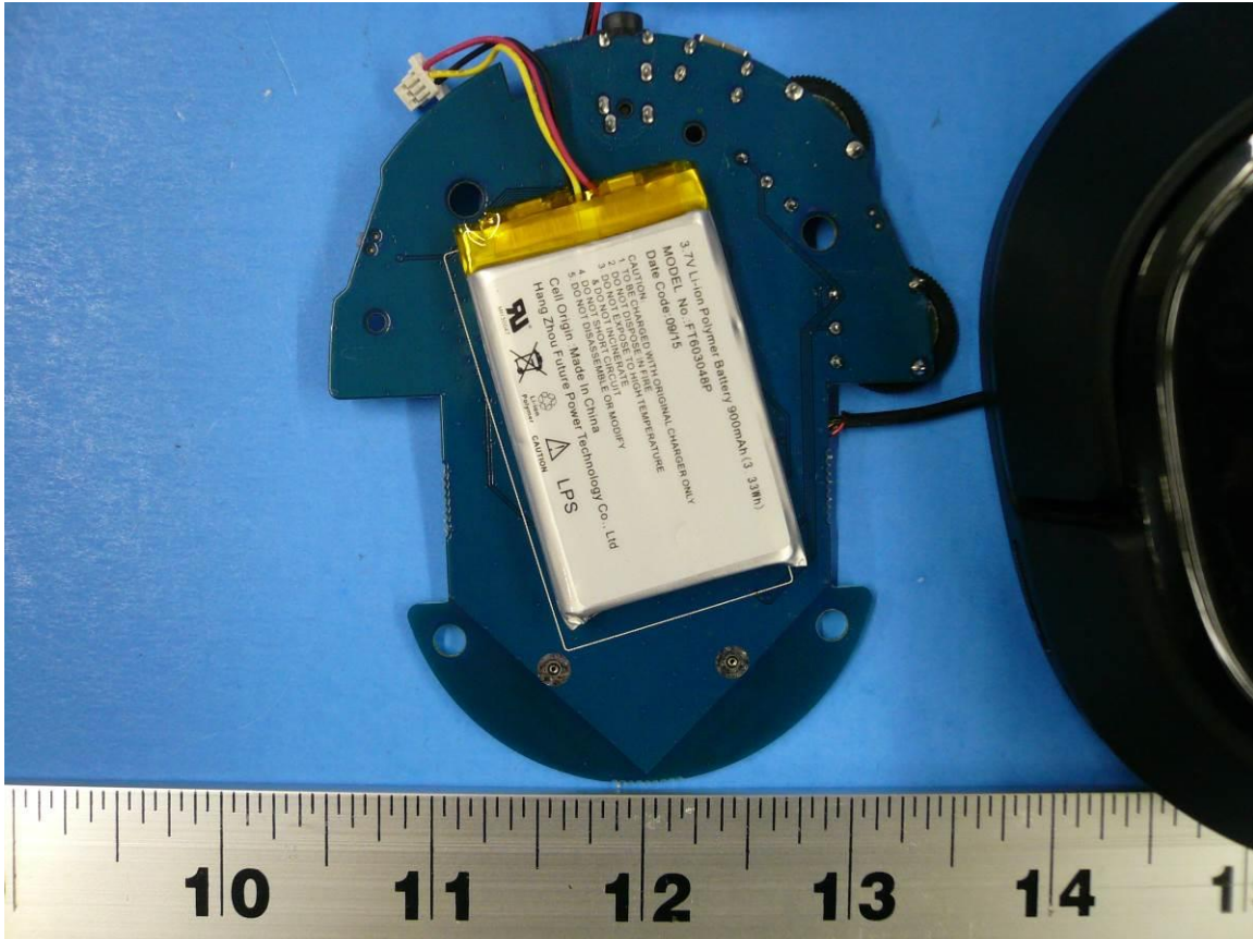
Figure 2: Internal Photo of Ear Force Stealth 520 RX - Bottom
