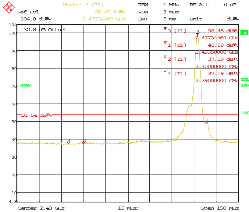
Figure 24: Bandedge-2477.35 MHz-H-Ave
