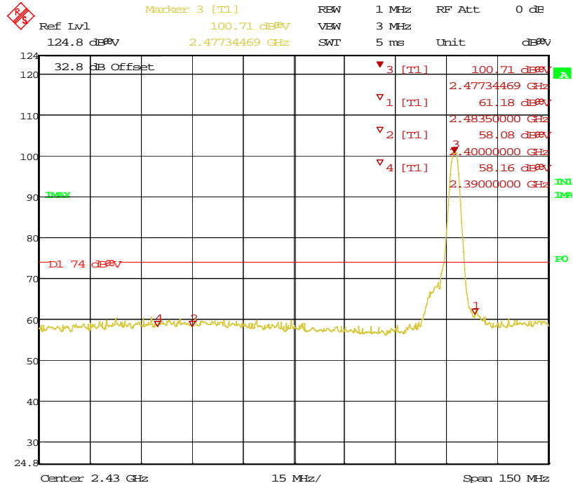
Figure 23: Bandedge-2477.35 MHz-H-Pk
