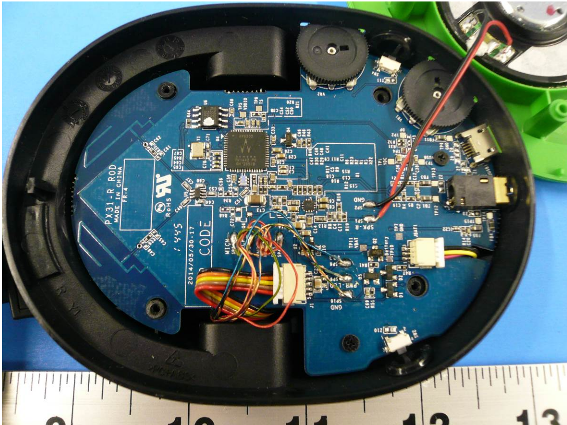
Figure 1: Internal Photo of Ear Force Stealth 420X RX - Top
