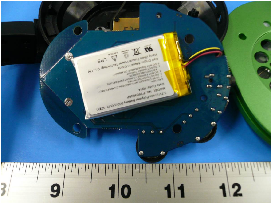
Figure 2: Internal Photo of Ear Force Stealth 420X RX - Bottom
