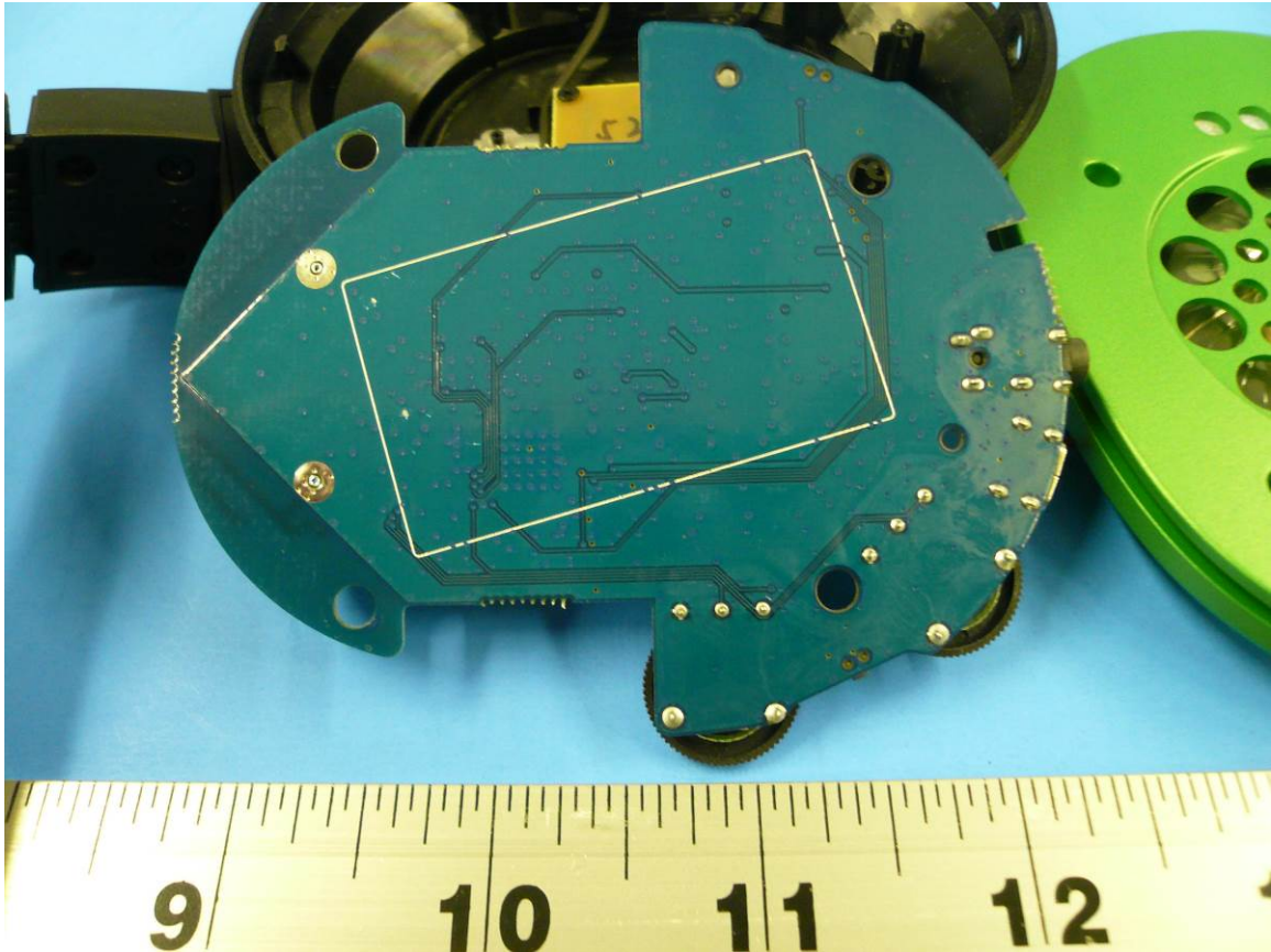
Figure 3: Internal Photo of Ear Force Stealth 420X RX without battery- Bottom
