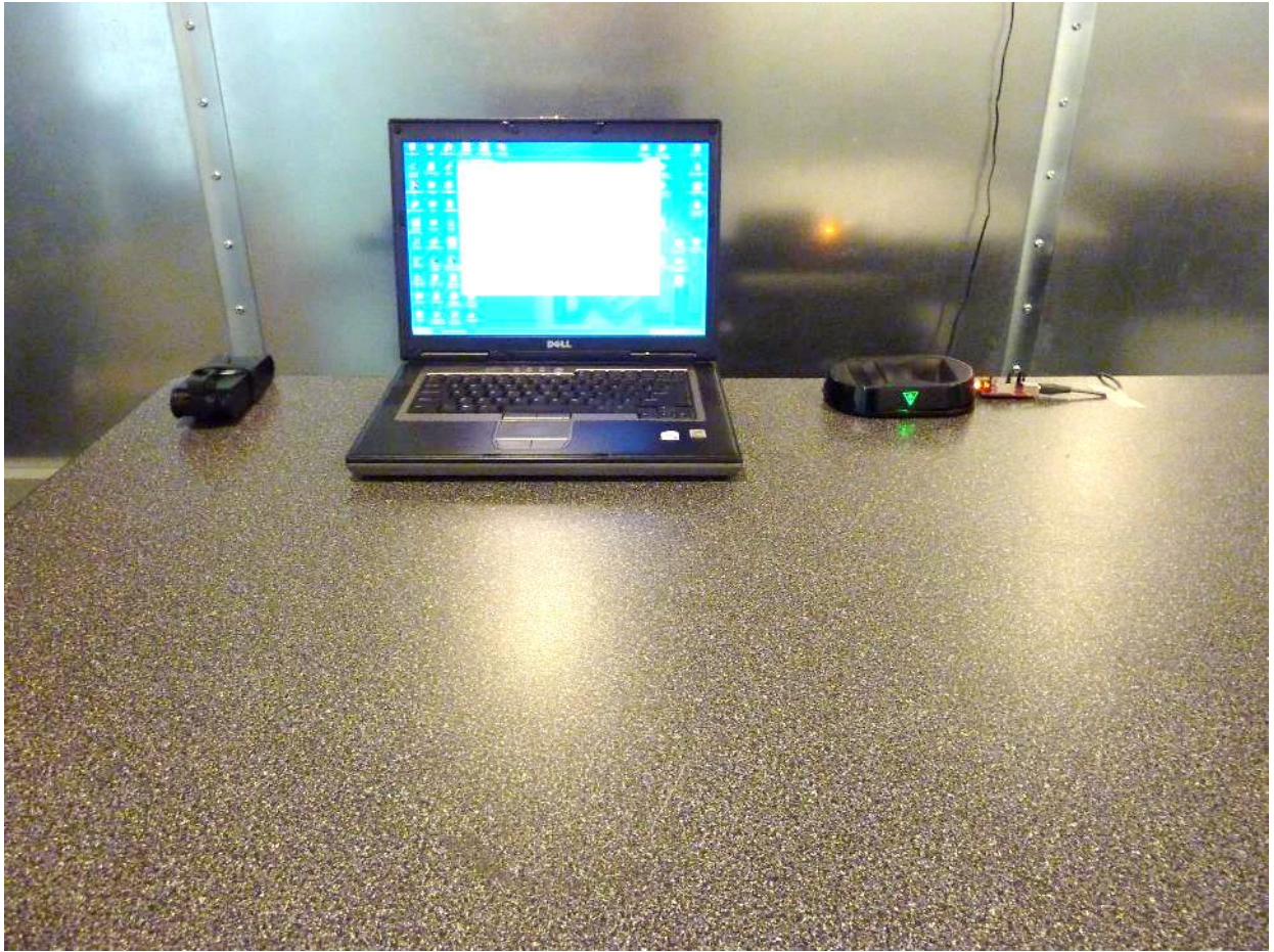
Figure 11: Conducted Emissions Test Setup (Front View)
