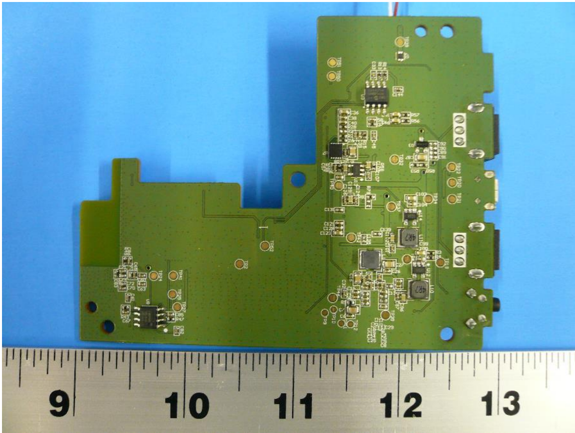
Figure 2: Internal Photo of Elite 800X TX - Bottom
