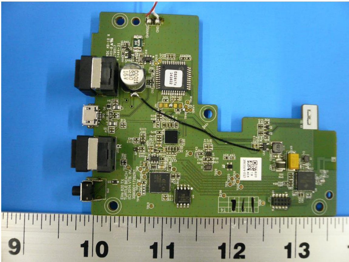
Figure 1: Internal Photo of Elite 800X TX – Top
