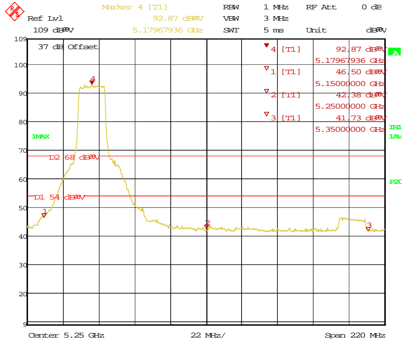
Figure 11: Bandedge-5180 MHz-11a-H-Ave
