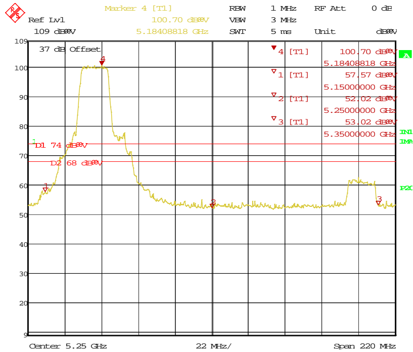
Figure 10: Bandedge-5180 MHz-11a-H-Pk
