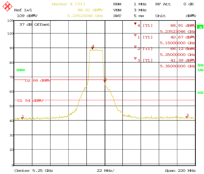
Figure 17: Bandedge-5240 MHz-V-Ave
