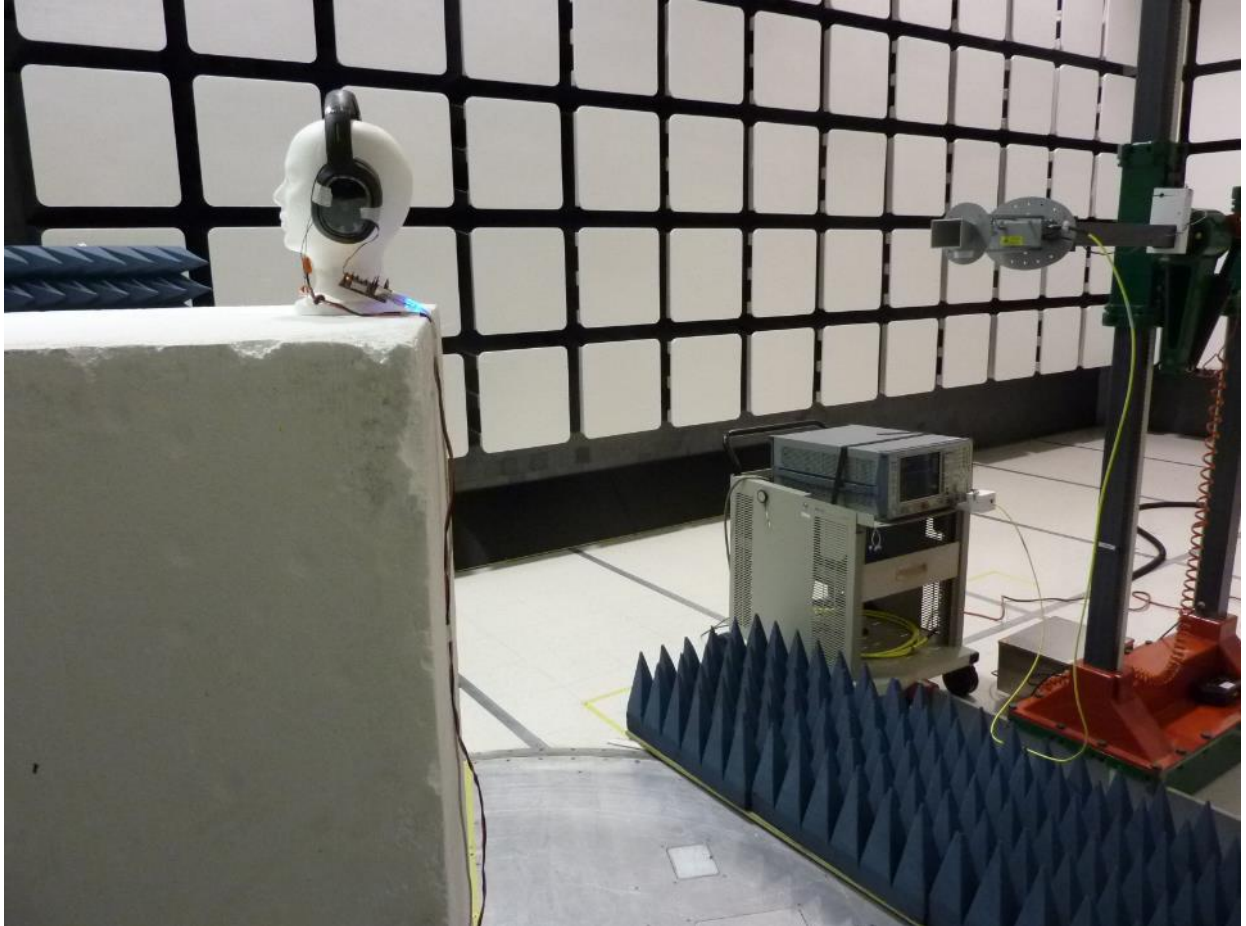
Figure 6: Test Setup for 18 GHz to 40GHz (Rear View)
