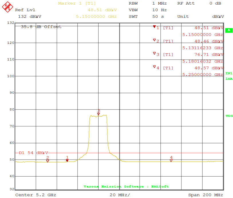
Figure 20: Radiated Emission 5150 MHz Edge for 11a 5180 MHz – Horz. (Avg)
