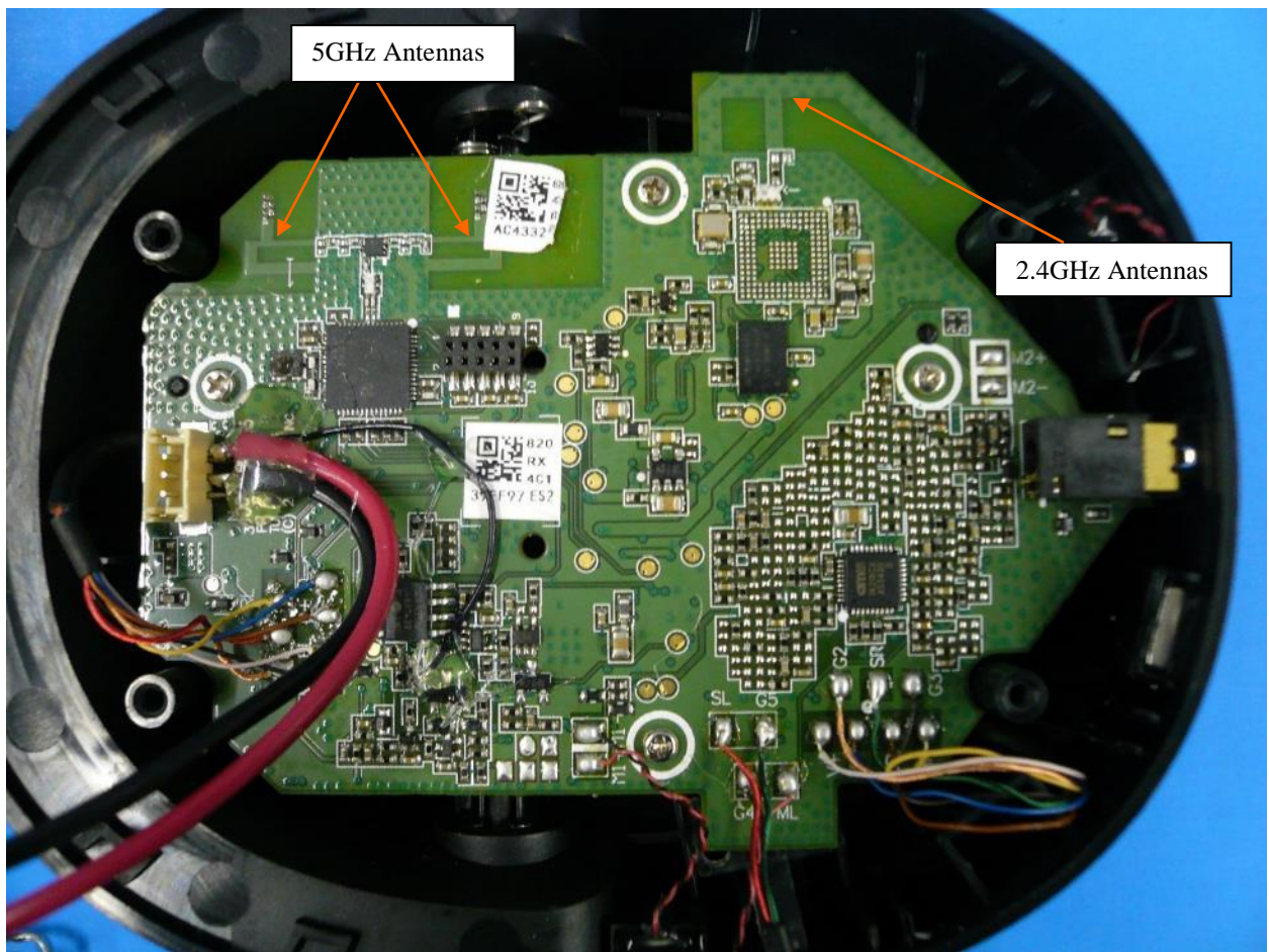
Figure 3: Internal Photo of Elite 800X RX – Antenna Location
