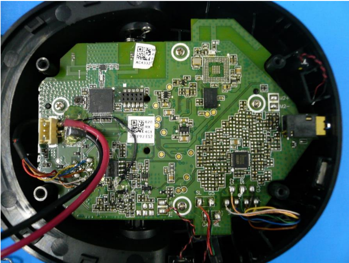
Figure 1: Internal Photo of Elite 800X RX – Top
