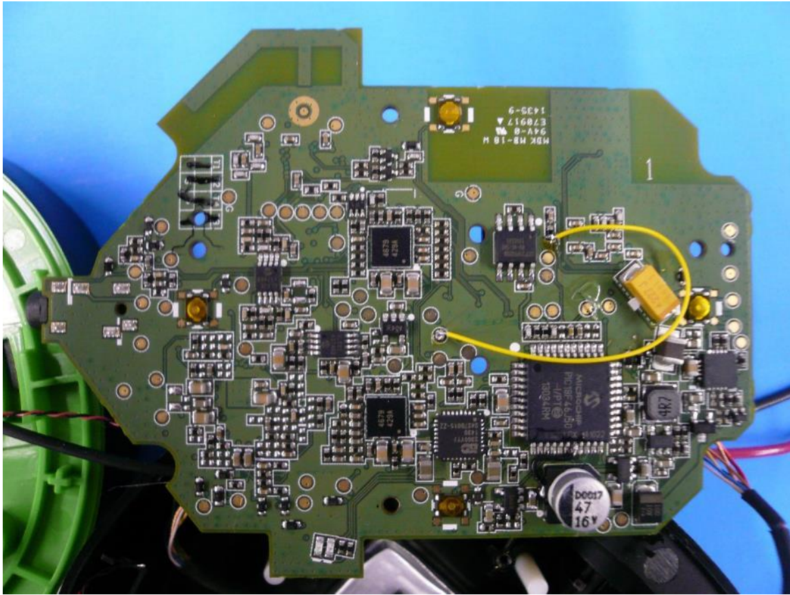
Figure 2: Internal Photo of Elite 800X RX - Bottom
