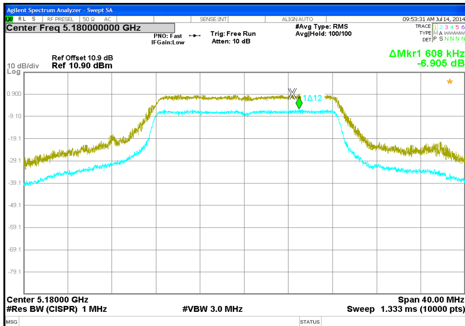
Figure 8: Peak Excursion-5180 MHz-11a-9Mbps
