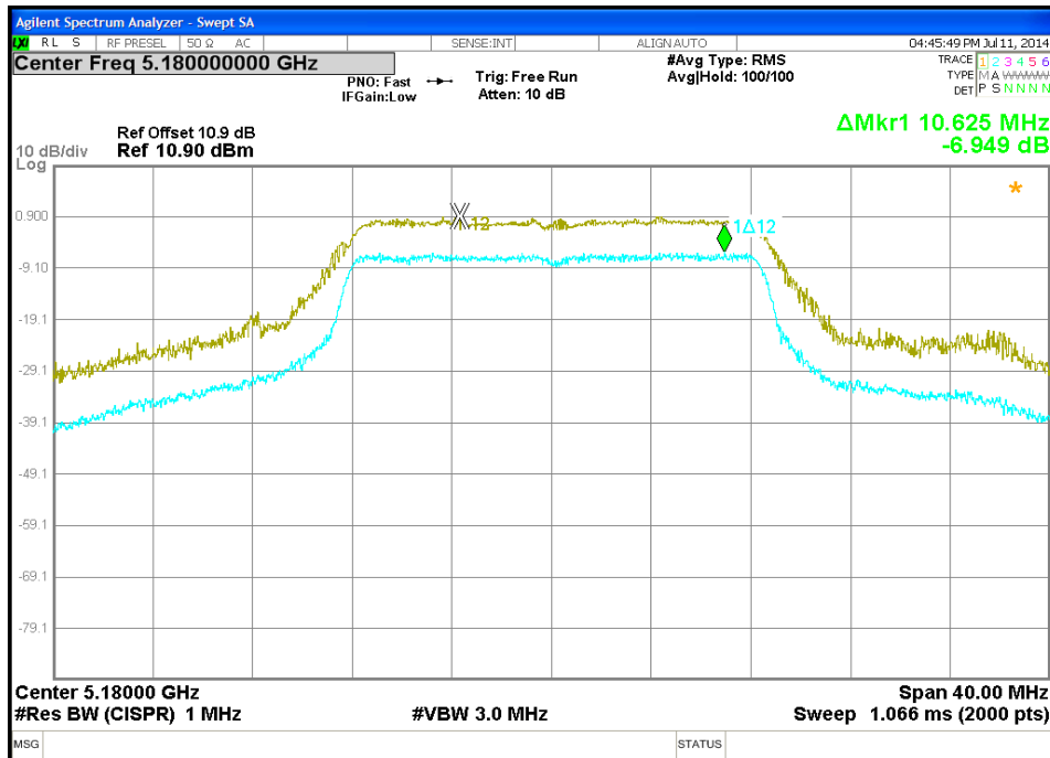
Figure 7: Peak Excursion-5180 MHz-11a-6Mbps
