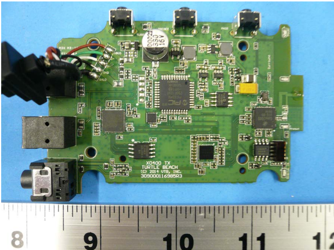
Figure 1: Internal Photo of Ear Force Stealth 500X TX - Top
