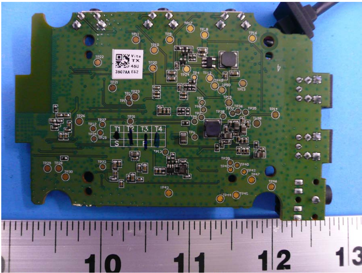
Figure 2: Internal Photo of Ear Force Stealth 500X TX - Bottom
