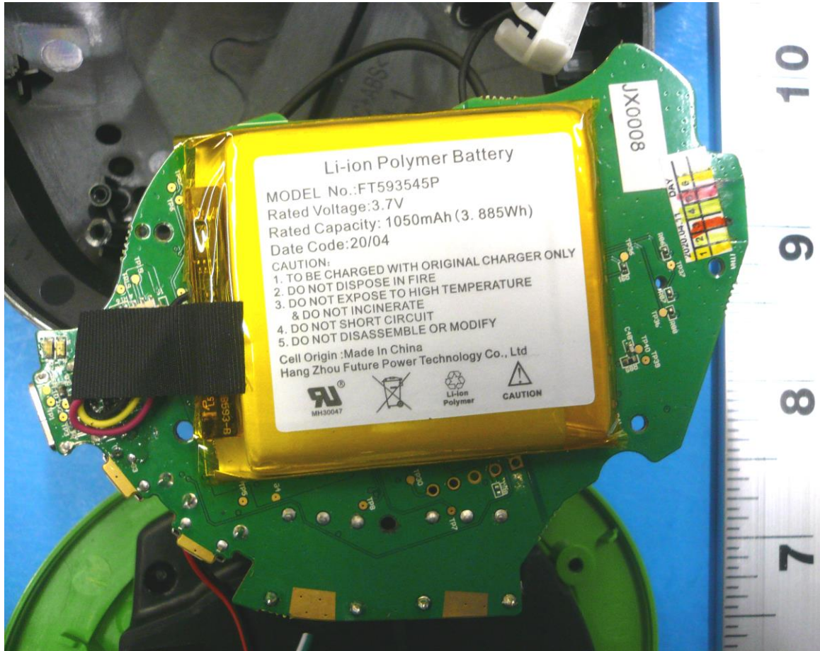
Figure 4: Internal Photo of Stealth 600X Gen 2 PCB (Bottom with Battery), Black & White versions
