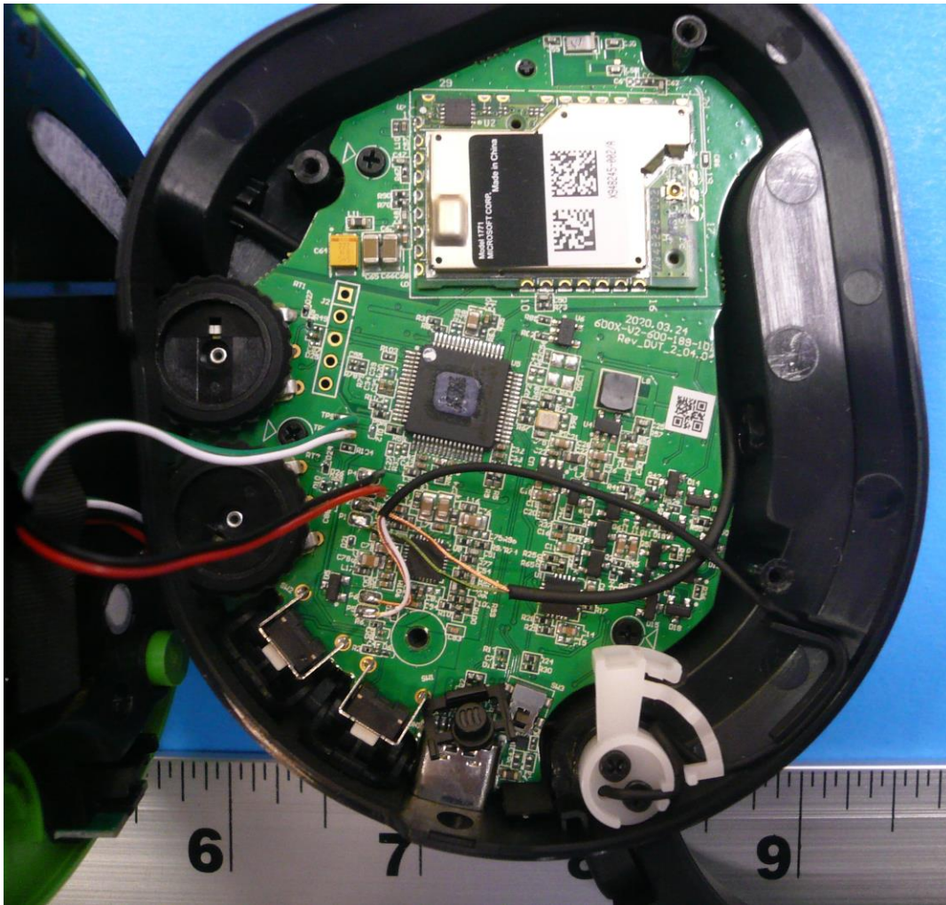
Figure 3: Internal Photo of Stealth 600X Gen 2 PCB, Black & White versions (Top)
