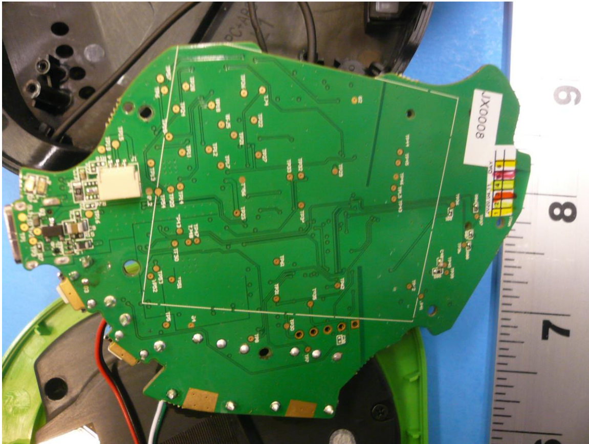
Figure 5: Internal Photo of Stealth 600X Gen 2 PCB (Bottom without Battery), Black & White versions
