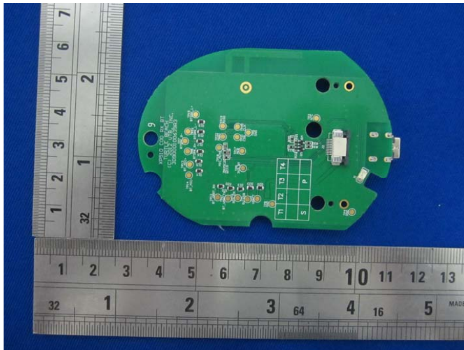
EUT –Bluetooth Board Bottom View
