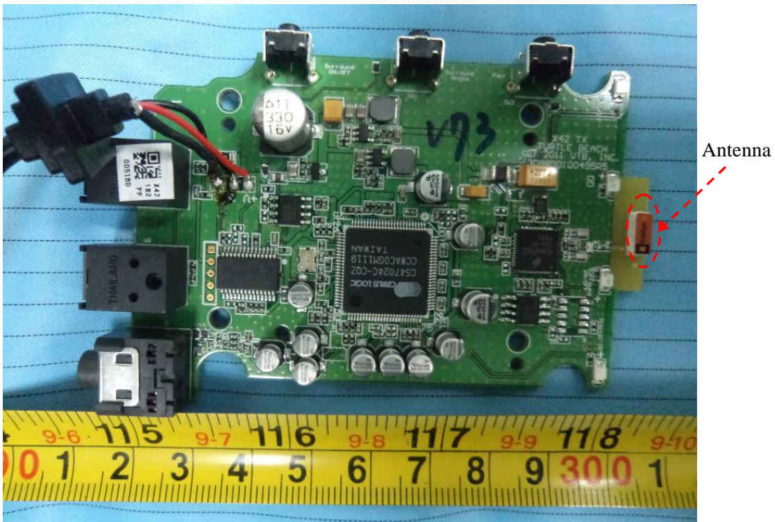
EUT – Main Board Top View
