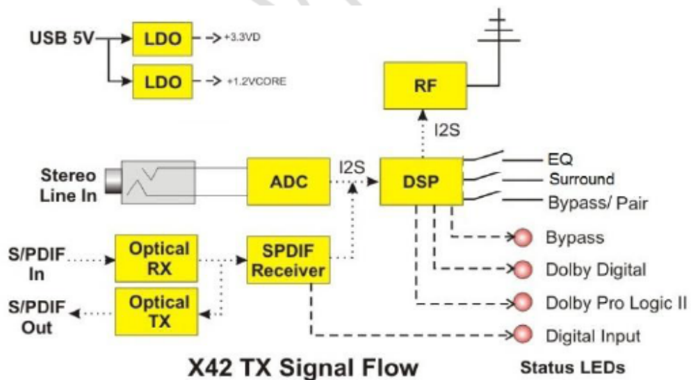
Picture 2 X42 Transmitter Block Diagram
