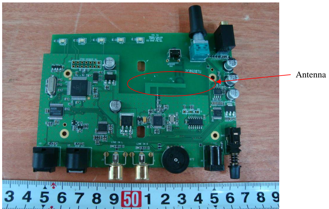
EUT – Main Board Components View
