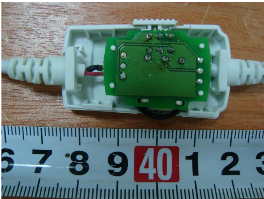
EUT – Control Cable Cover off View
