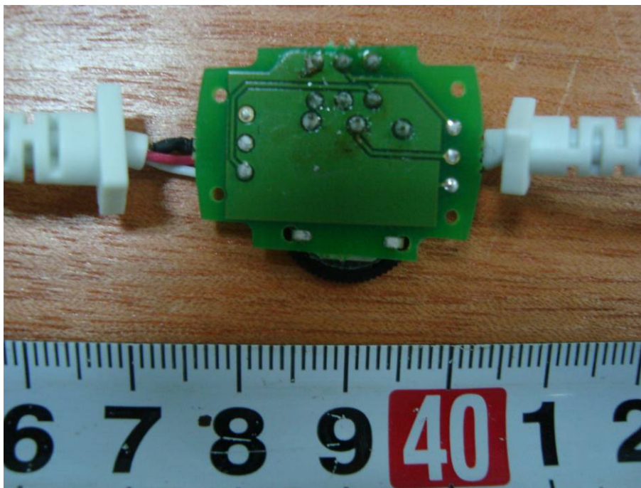
EUT – Control Cable Board Bottom View
