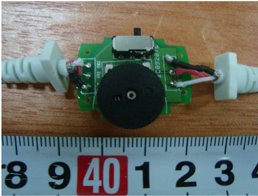
EUT – Control Cable Board Top View
