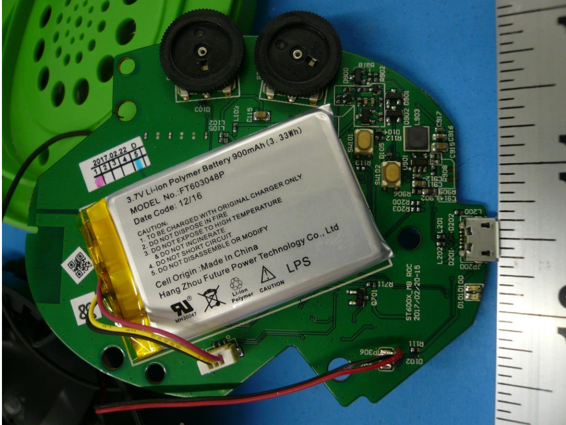
Figure 4: Internal Photo of Ear Force Stealth 600X PCB (Bottom with Battery)
