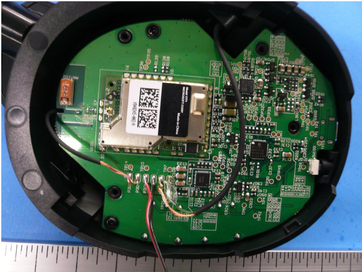
Figure 3: Internal Photo of Ear Force Stealth 600X PCB (Top)
