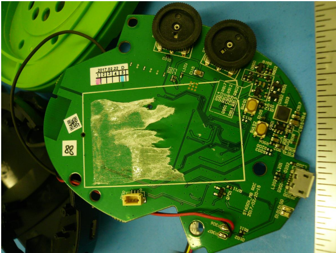
Figure 5: Internal Photo of Ear Force Stealth 600X PCB (Bottom without Battery)
