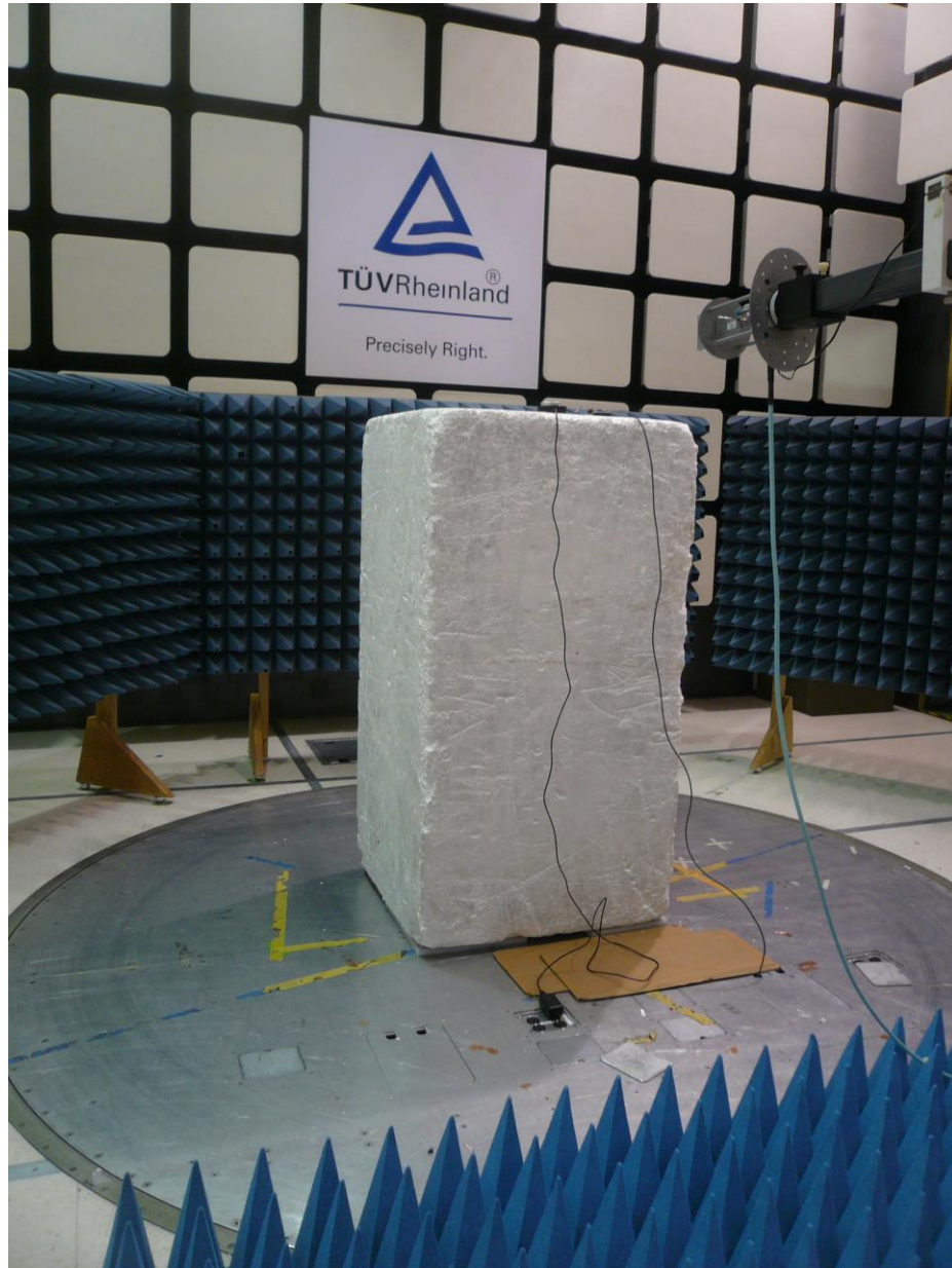
Figure 7: Test Setup for 18 GHz to 26 GHz (Rear View)
