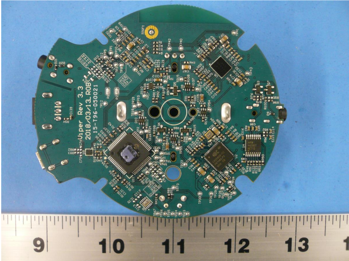
Figure 3: Internal Photo of Elite SuperAmp P - Bottom
