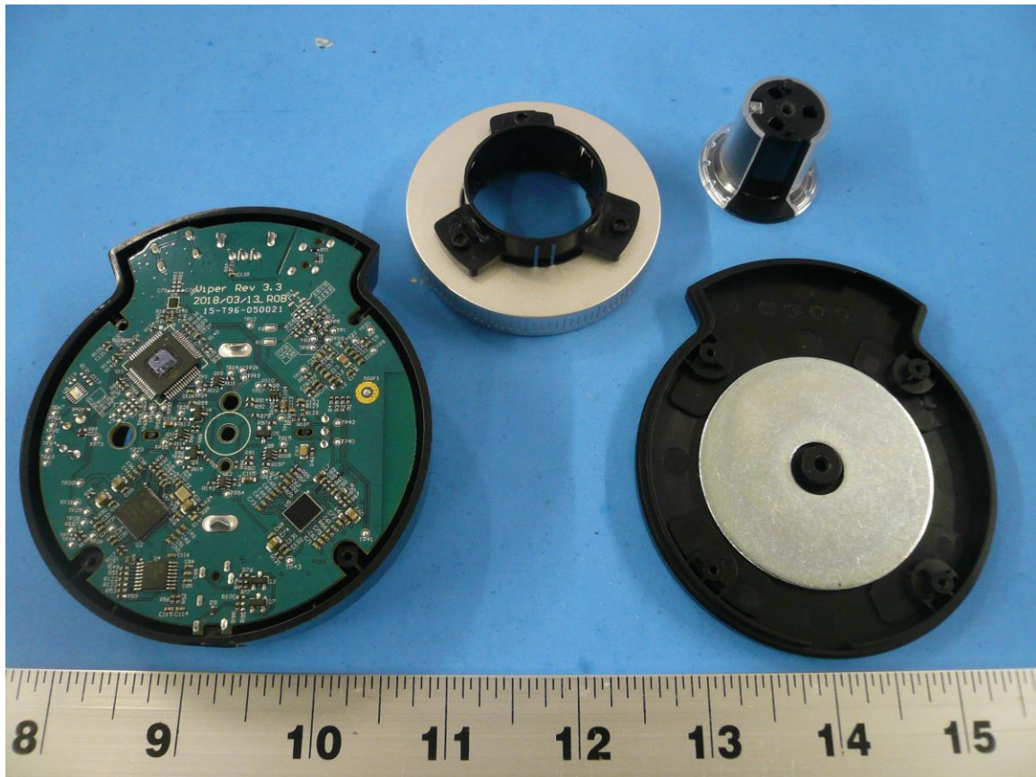
Figure 1: Internal Photo of Elite SuperAmp P - Internal
