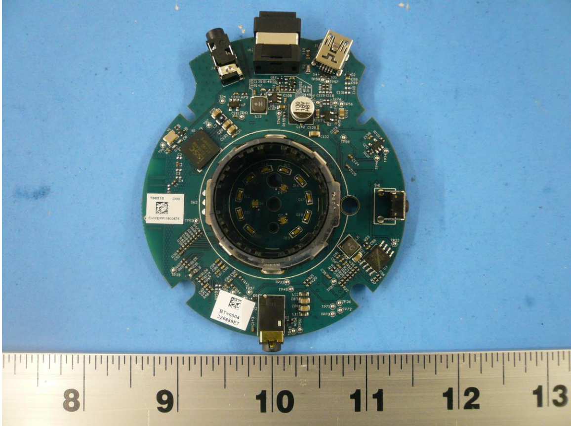
Figure 2: Internal Photo of Elite SuperAmp P - Top
