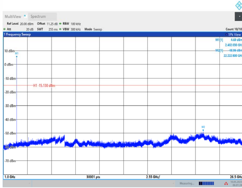
BLE_1M_Ant1_2402_1000~26500
