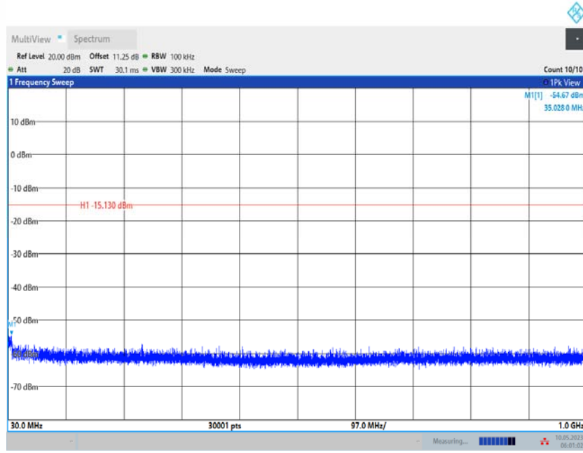
BLE_1M_Ant1_2402_30~1000
