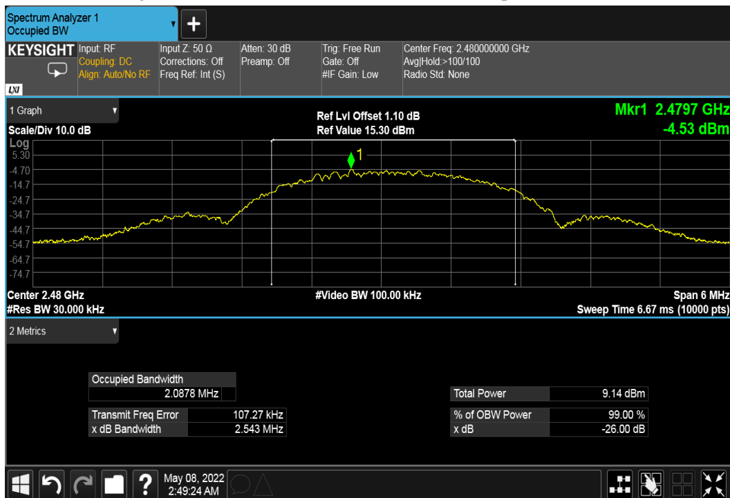
Figure 20: 99% Bandwidth 2480 MHz at 2 Mbps
