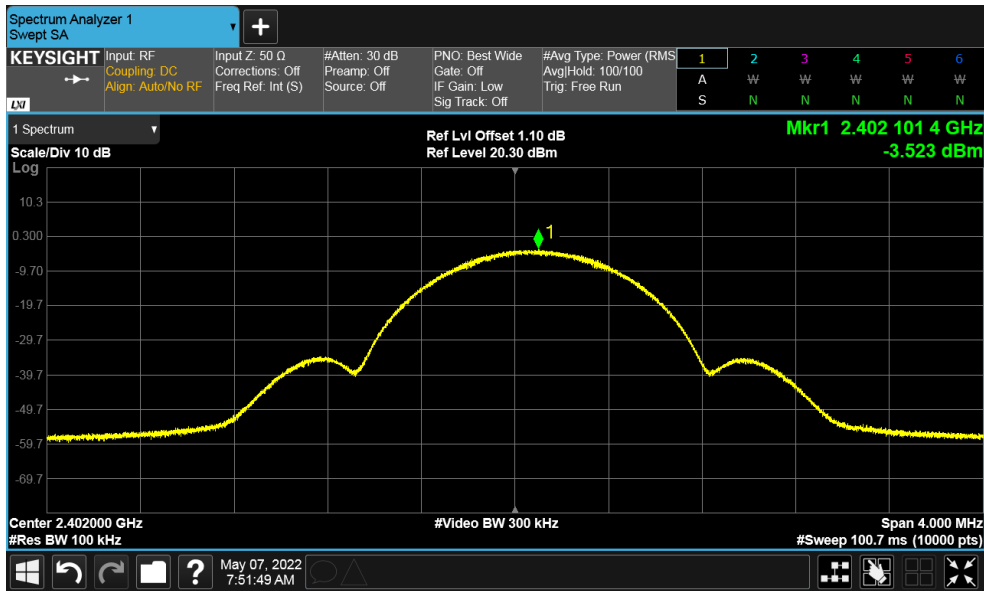
Figure 21: Maximum Power Spectral Density-2402 MHz at 1 Mbps
