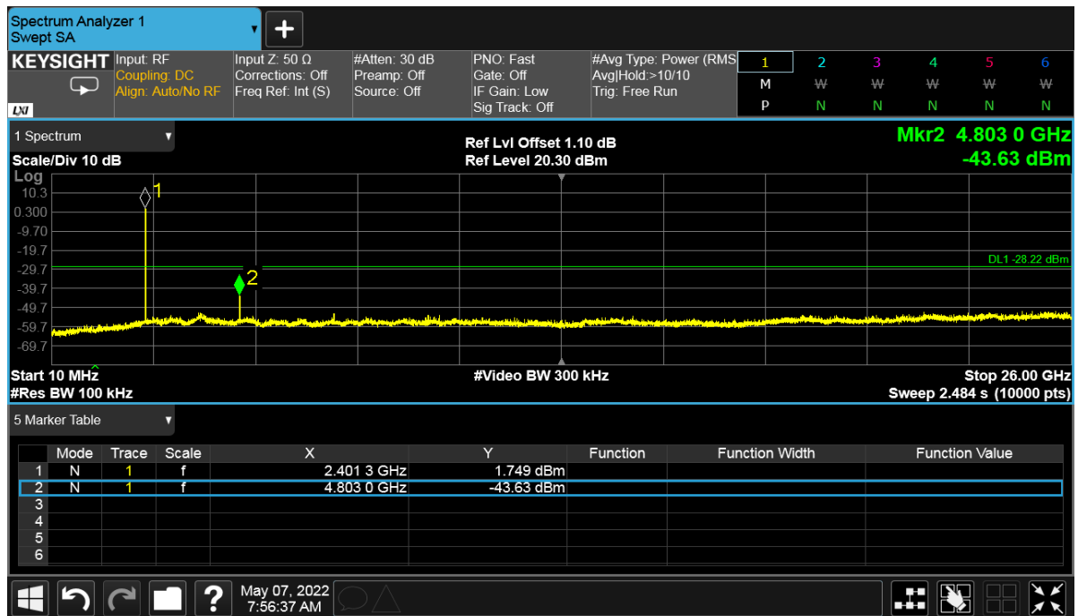
Figure 28: Out of band Emission - 2402 MHz at 1 Mbps
