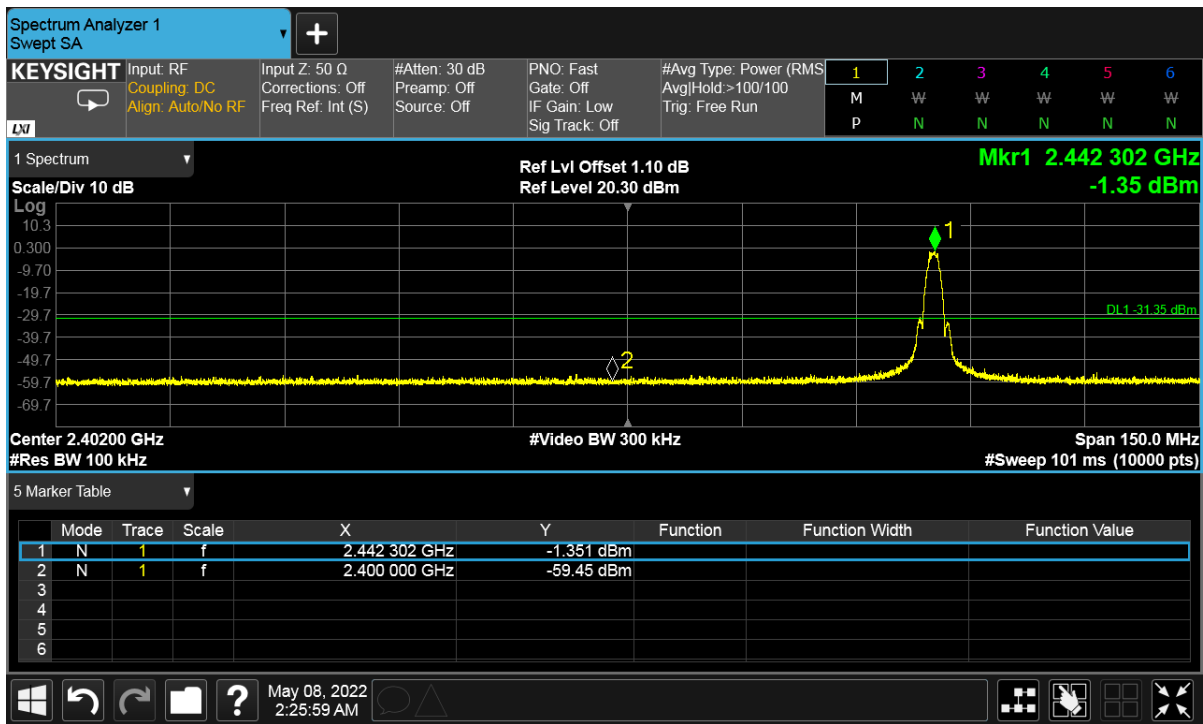
Figure 35: Conducted Band Edge - 2442 MHz at 2 Mbps
