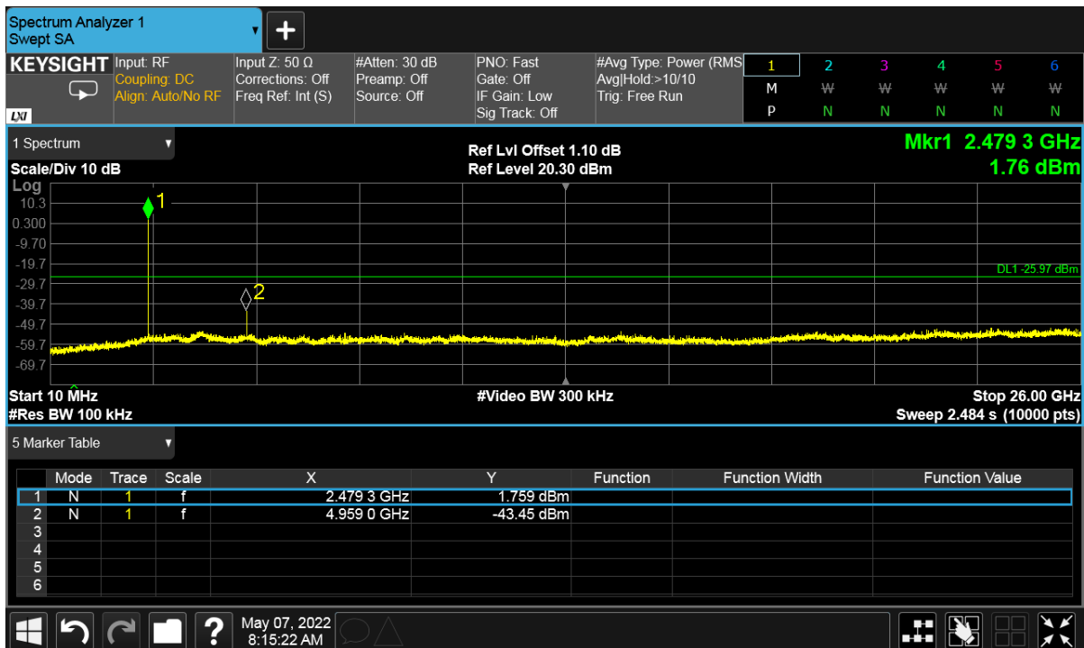
Figure 32: Out of band Emission - 2480 MHz at 1 Mbps
