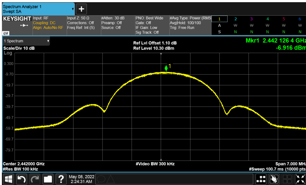
Figure 25: Maximum Power Spectral Density-2442 MHz at 2 Mbps
