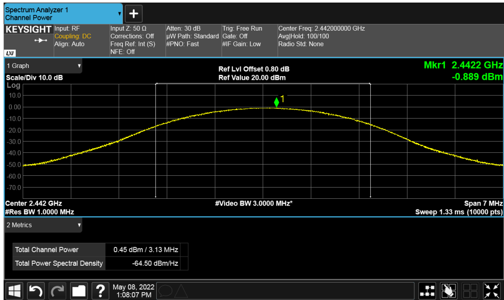
Figure 7: Maximum Conducted Output Power, 2442 MHz at 2 Mbps
