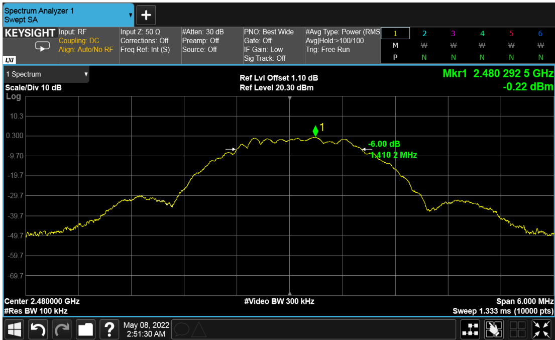
Figure 17: DTS Bandwidth 2480 MHz at 2 Mbps
