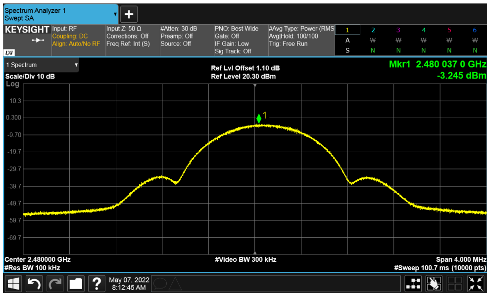
Figure 23: Maximum Power Spectral Density-2480 MHz at 1 Mbps
