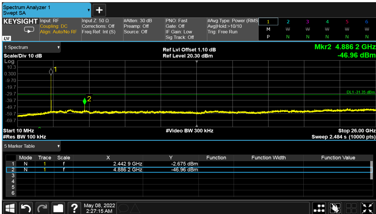
Figure 36: Out of band Emission - 2442 MHz at 2 Mbps
