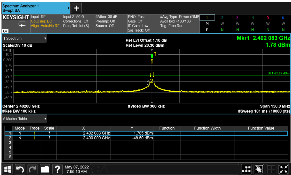
Figure 27: Conducted Band Edge - 2402 MHz at 1 Mbps
