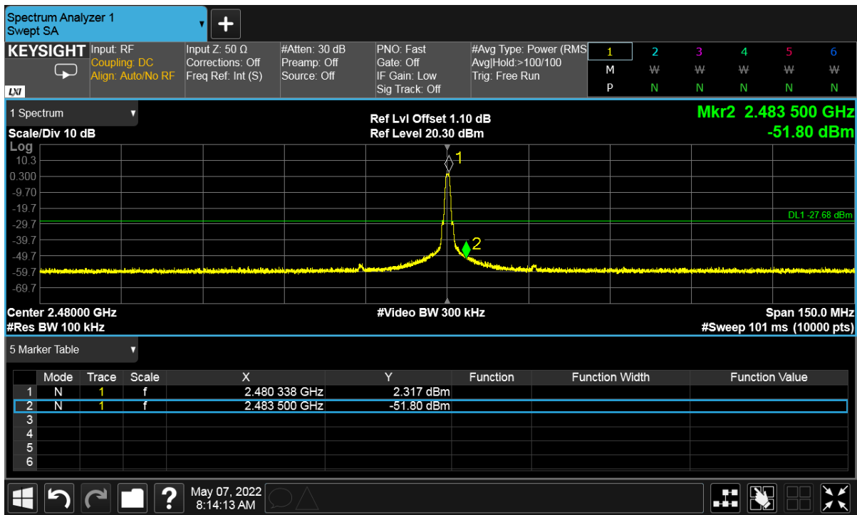
Figure 31: Conducted Band Edge - 2480 MHz at 1 Mbps
