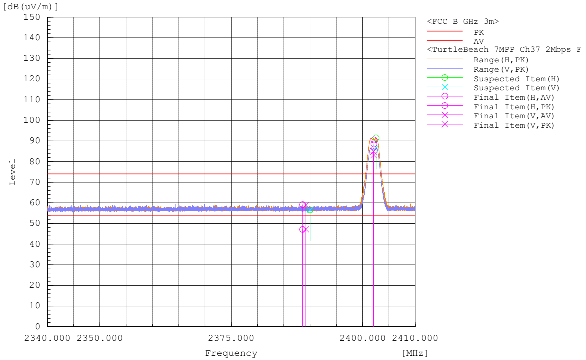
Figure 39: Band-edge-2402 MHz
