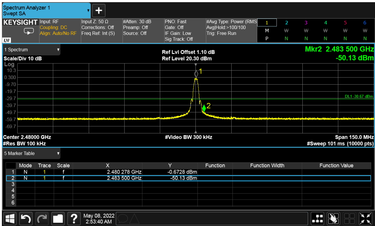
Figure 37: Conducted Band Edge - 2480 MHz at 2 Mbps
