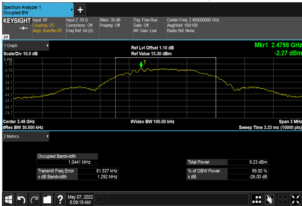
Figure 14: 99% Bandwidth 2480 MHz at 1 Mbps
