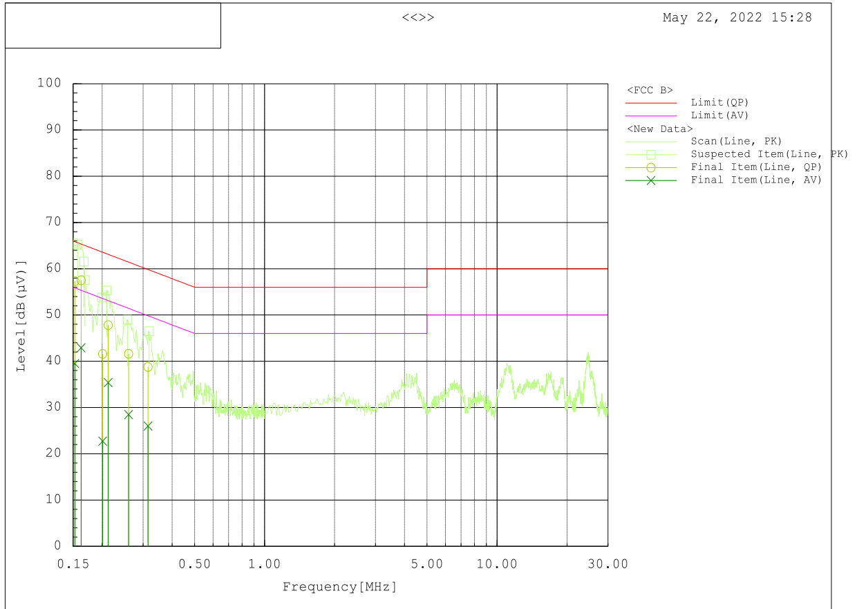
150 kHz to 30 MHz Plot for Line 1 (Hot)
