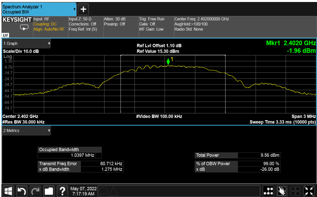
Figure 12: 99% Bandwidth 2402 MHz at 1 Mbps
