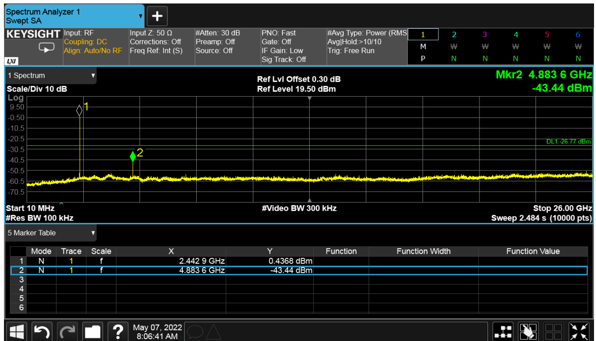
Figure 30: Out of band Emission - 2442 MHz at 1 Mbps
