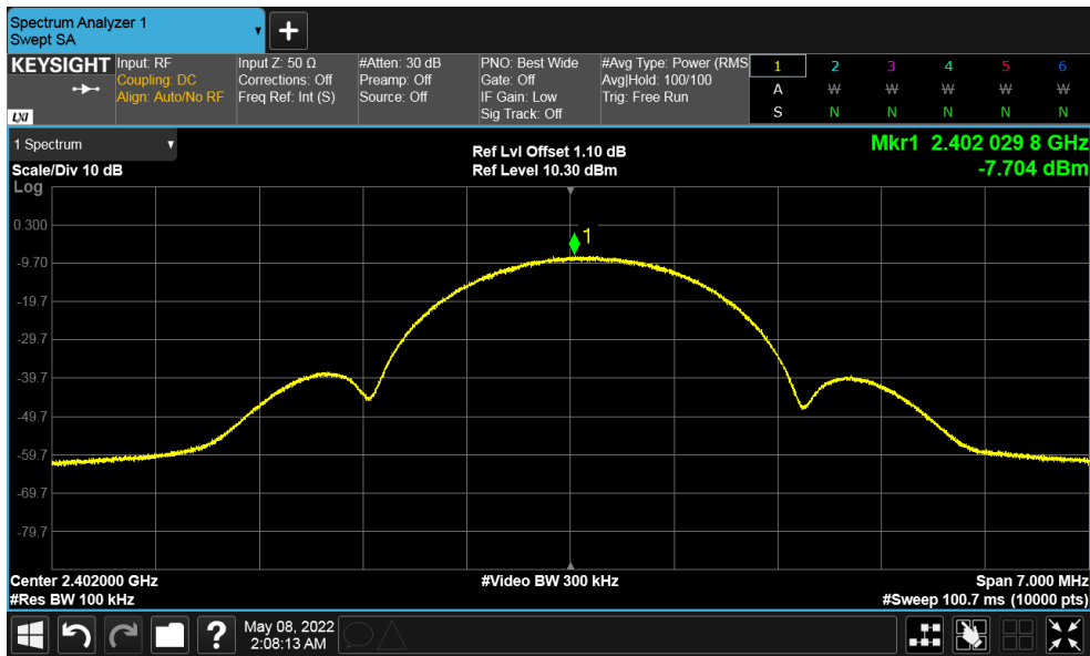
Figure 24: Maximum Power Spectral Density-2402 MHz at 2 Mbps
