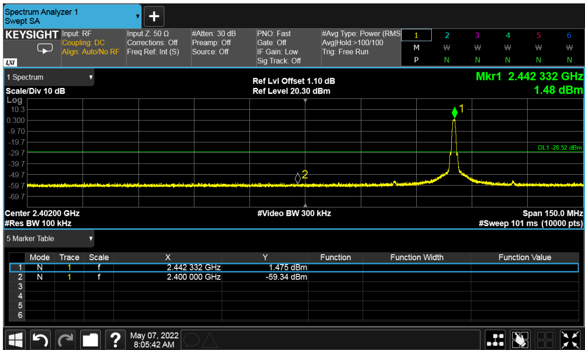
Figure 29: Conducted Band Edge - 2442 MHz at 1 Mbps
