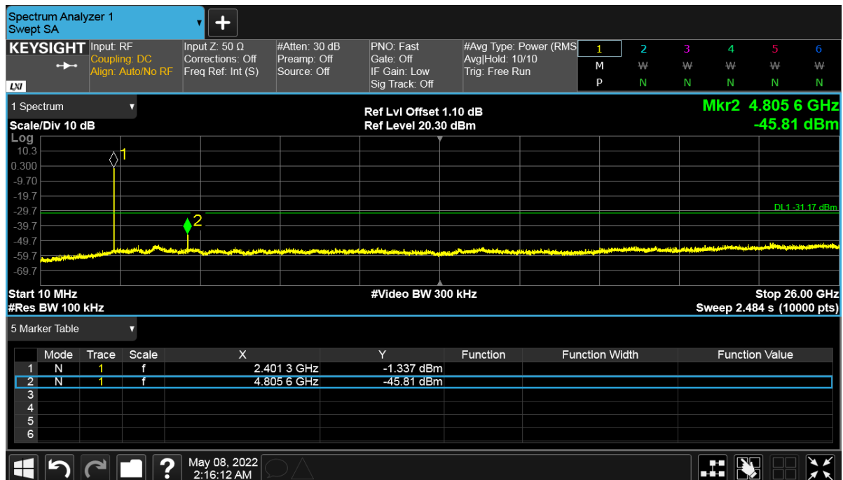
Figure 34: Out of band Emission - 2402 MHz at 2 Mbps
