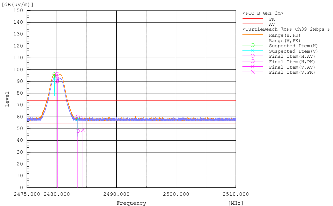
Figure 40: Band-edge-2480 MHz
