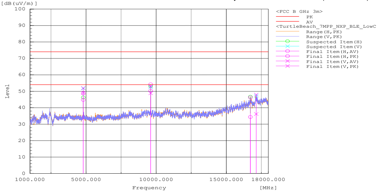
Above 1 GHz Plots for Co-location of NXP at 2402 MHz and Skyworks BT at 2402 MHz (Worst Case)
