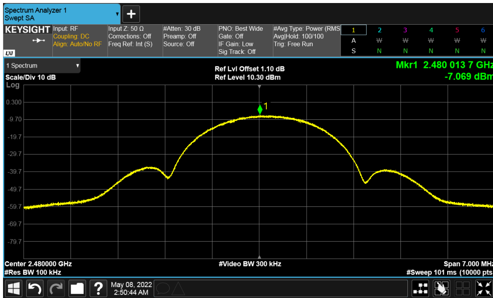
Figure 26: Maximum Power Spectral Density-2480 MHz at 2 Mbps
