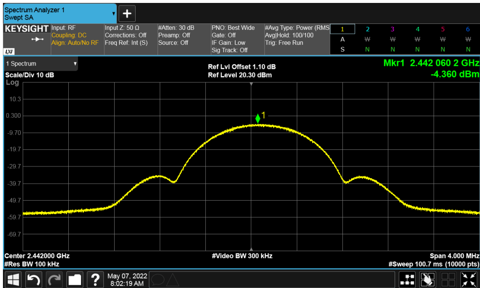
Figure 22: Maximum Power Spectral Density-2442 MHz at 1 Mbps
