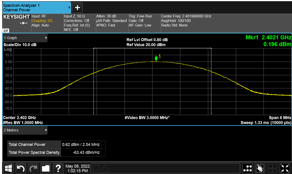
Figure 3: Maximum Conducted Output Power, 2402 MHz at 1 Mbps
