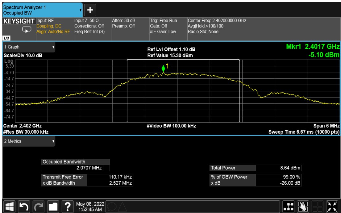
Figure 18: 99% Bandwidth 2402 MHz at 2 Mbps
