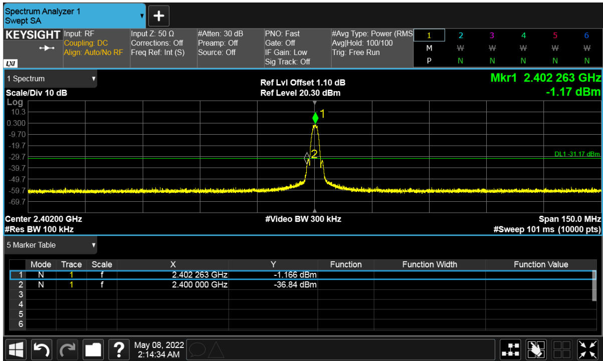
Figure 33: Conducted Band Edge - 2402 MHz at 2 Mbps
