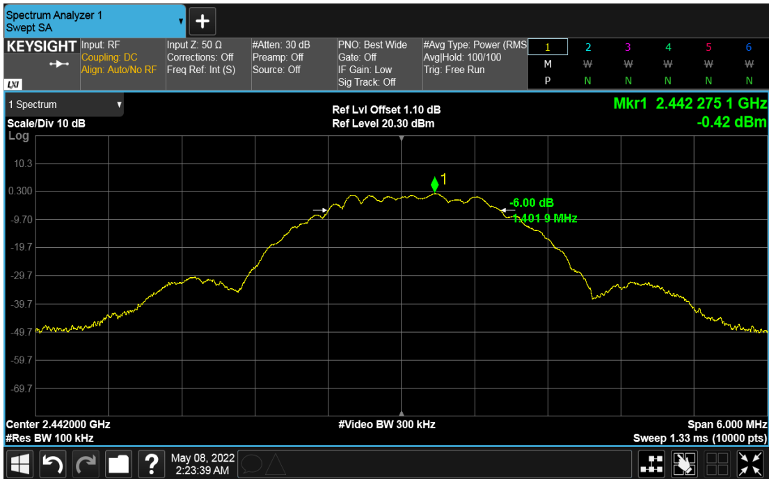
Figure 16: DTS Bandwidth 2442 MHz at 2 Mbps
