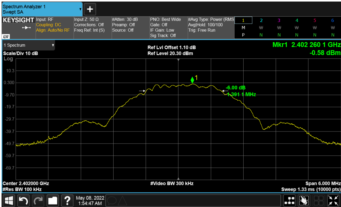
Figure 15: DTS Bandwidth 2402 MHz at 2 Mbps
