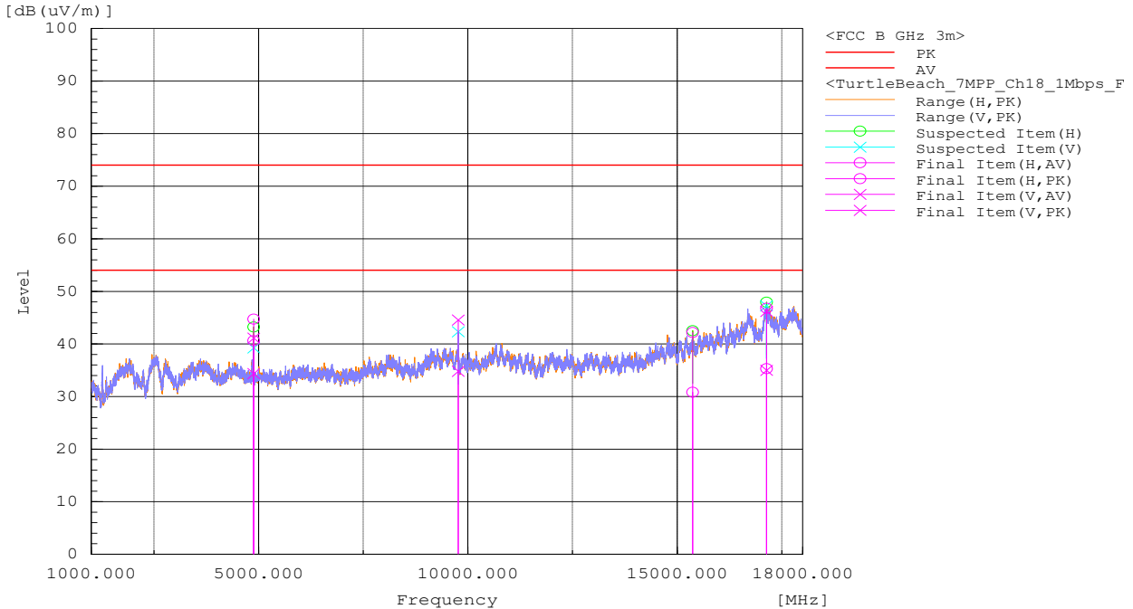
Above 1 GHz Plots for Transmit Mode at 2442 MHz
