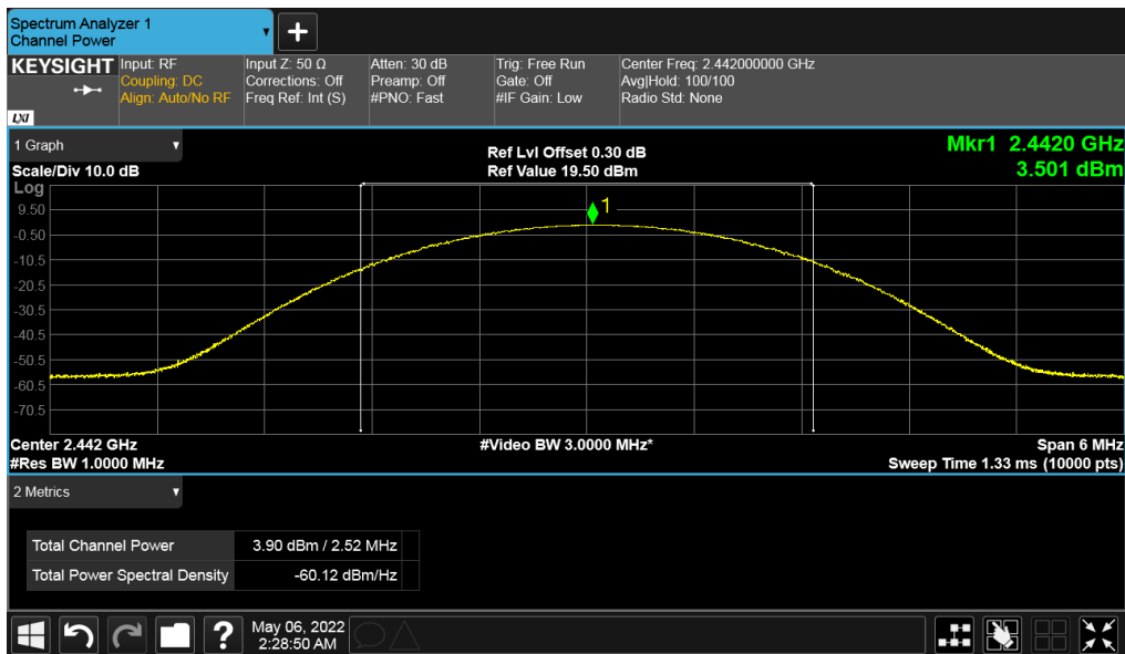
Figure 3: Maximum Conducted Output Power at 2442 MHz
