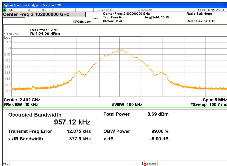
Figure 8: 99% Bandwidth-Headset -2402 MHz
