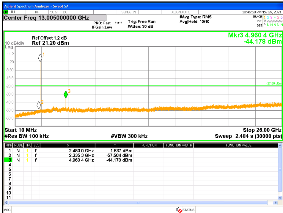
Figure 19: Out of band Emissions at 2480 MHz-Headset
