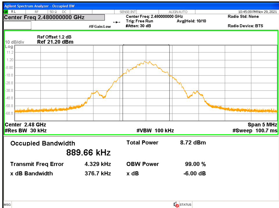
Figure 10: 99% Bandwidth-Headset -2480 MHz
