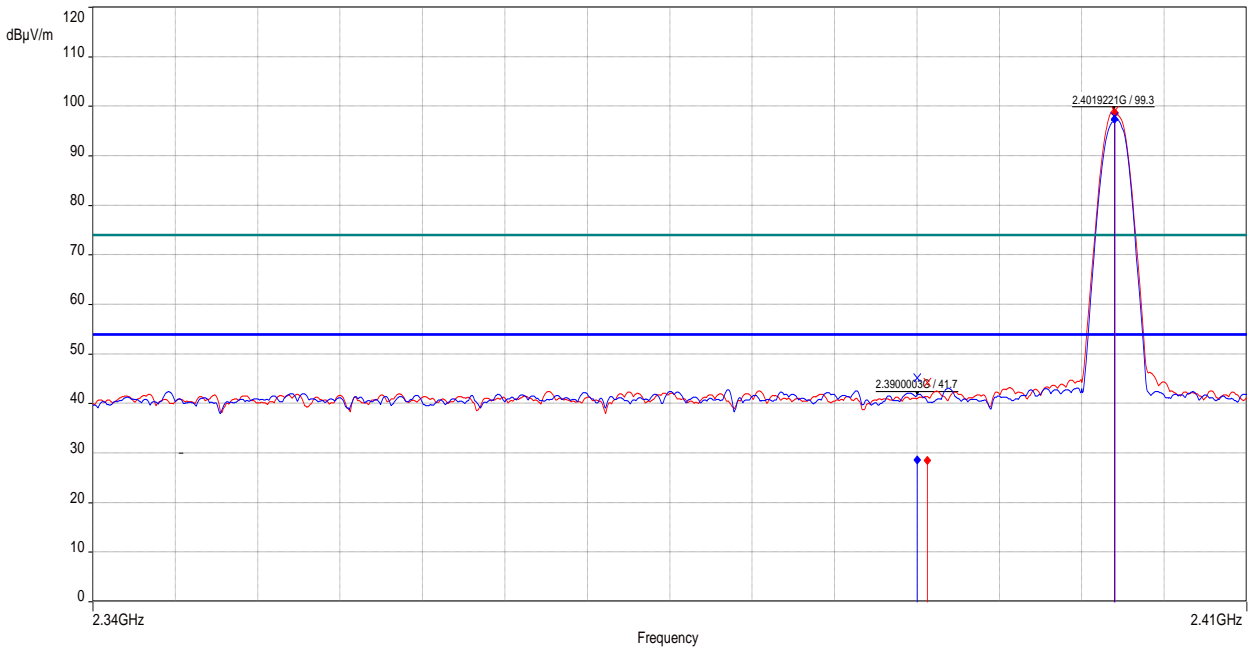
Figure 20: Band-edge-2402 MHz
