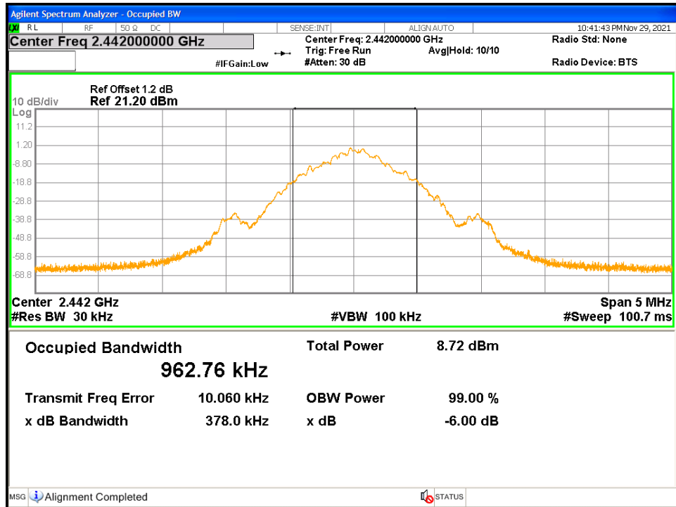
Figure 9: 99% Bandwidth-Headset -2442 MHz
