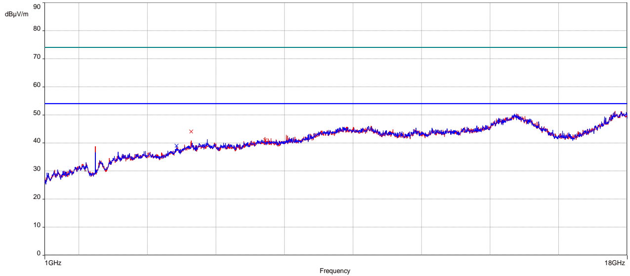
Above 1 GHz Plots for Transmit Mode at 2480 MHz
