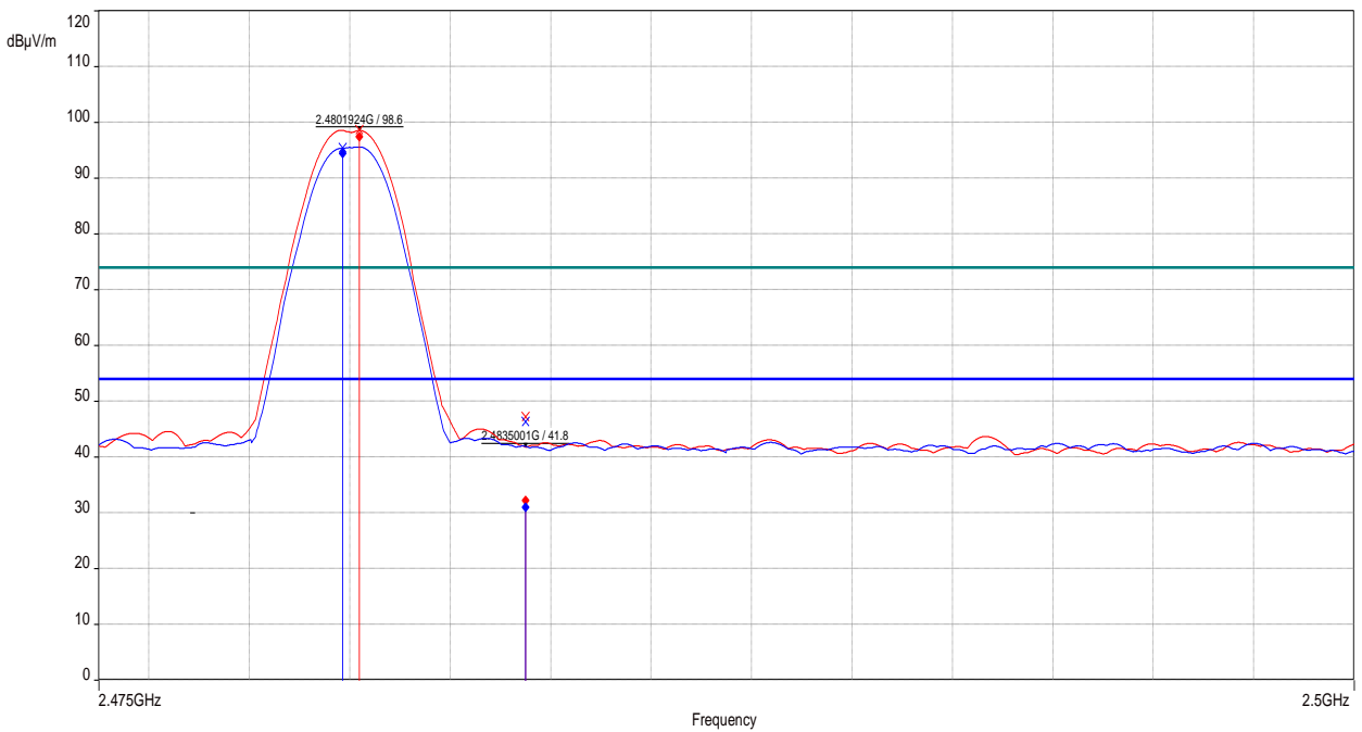
Figure 21: Band-edge-2480 MHz
