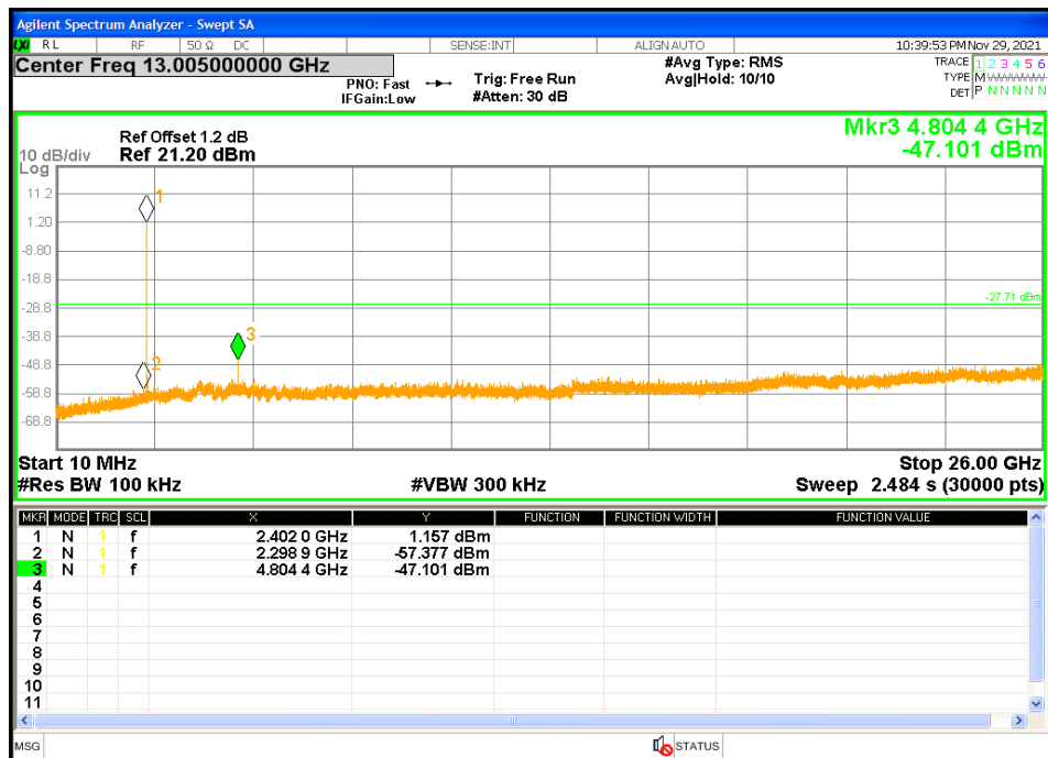
Figure 15: Out of band Emissions at 2402 MHz-Headset
