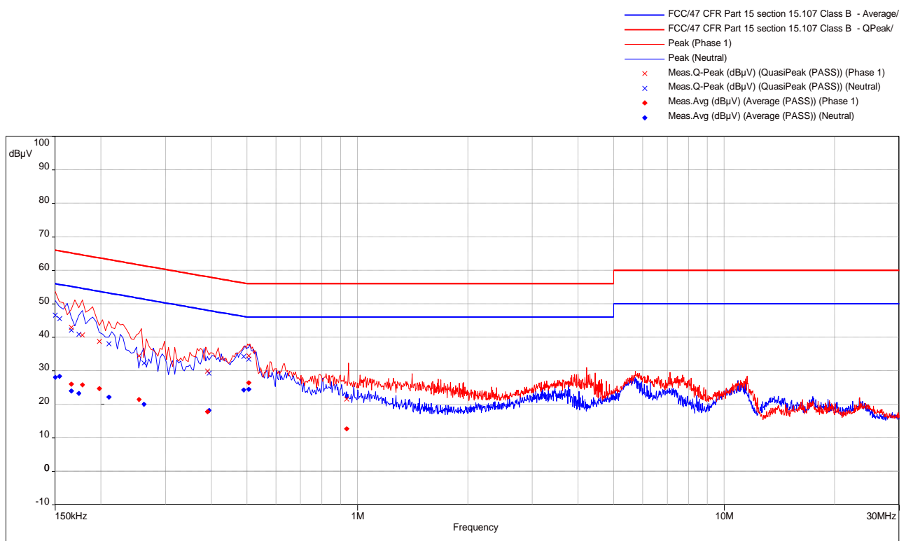
150 kHz to 30 MHz Plot for Live and Neutral
