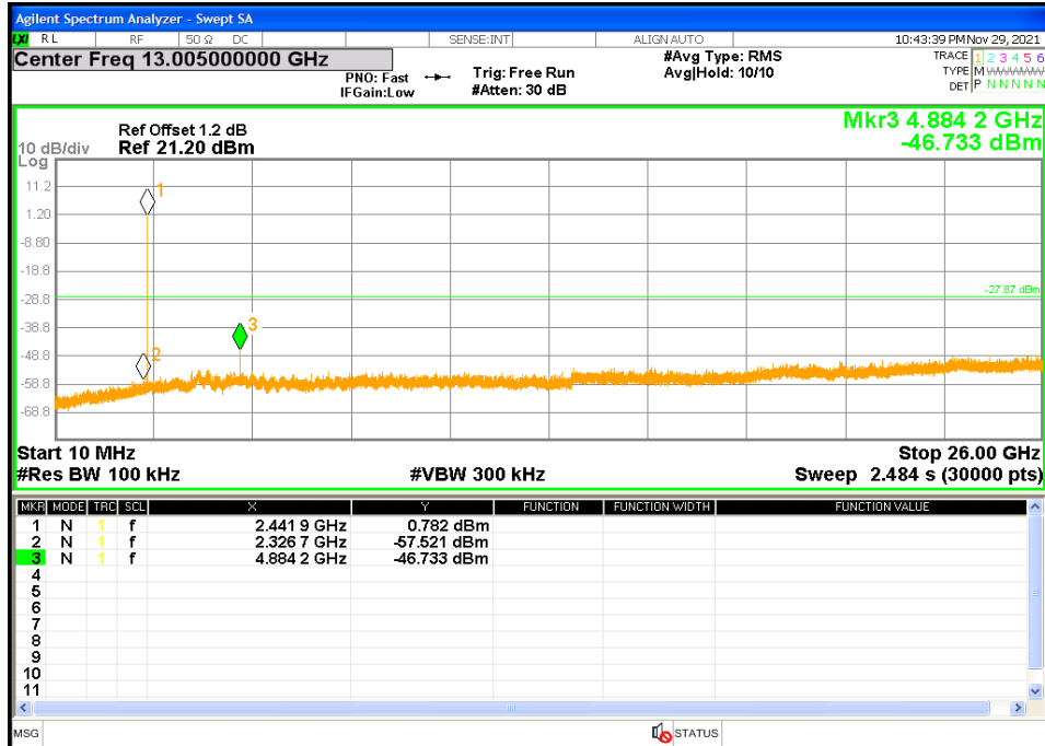
Figure 17: Out of band Emissions at 2442 MHz-Headset
