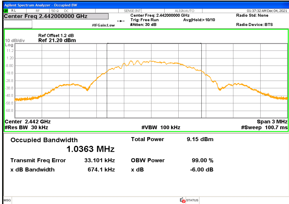
Figure 9: 99% Bandwidth-Headset -2442 MHz
