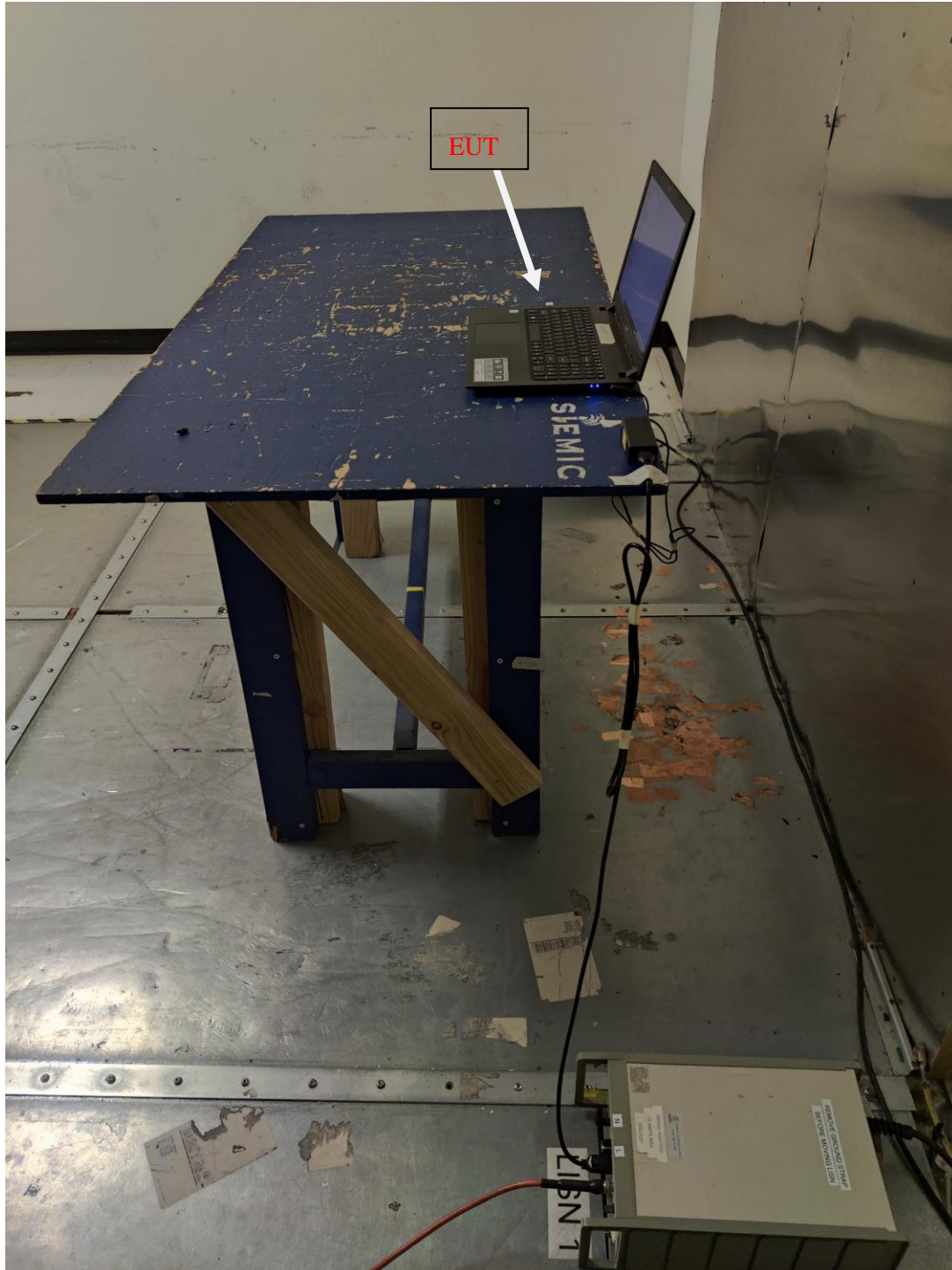
Figure 11: AC Conducted Emission Test Setup (Side)
