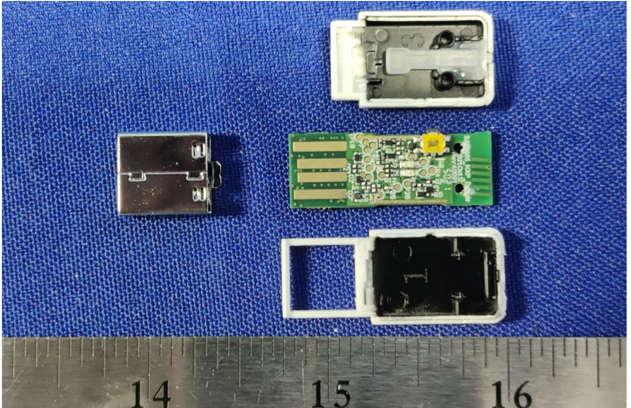
Figure 1: Internal Photo of Stealth600P-USB-TX with Plastic Cover Removed
