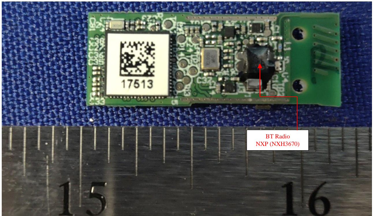
Figure 2: Internal Photo of Stealth600P-USB-TX – Top PCB
