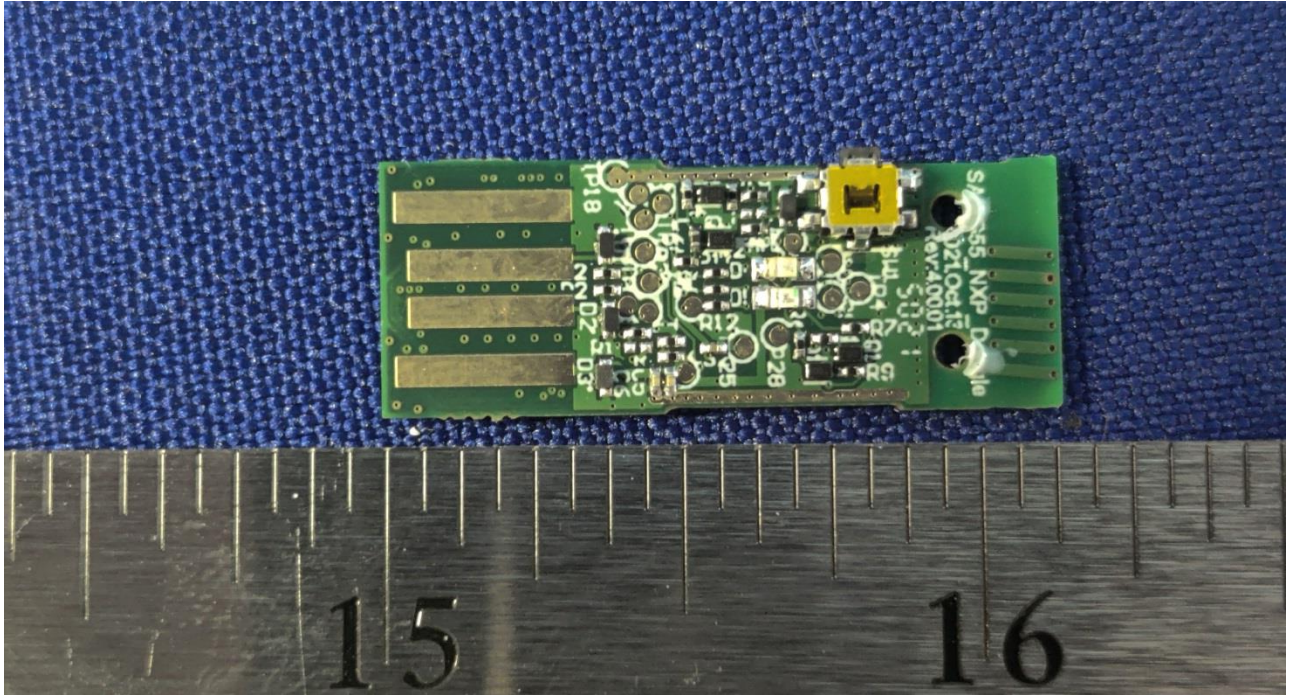
Figure 3: Internal Photo of Stealth600P-USB-TX – Bottom PCB
