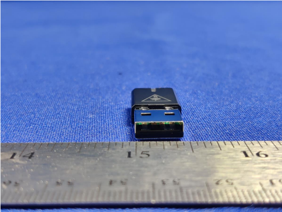
Figure 3: External Photo of Stealth600P-USB-TX – Rear (Black Version)
