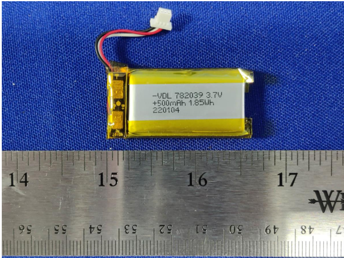
Figure 5: Internal Photo of Stealth600P-USB-RX – Battery
