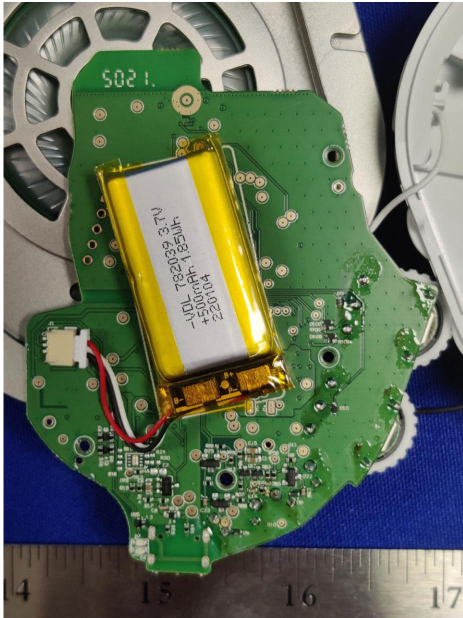
Figure 3: Internal Photo of Stealth600P-USB-RX – Bottom PCB with Battery
