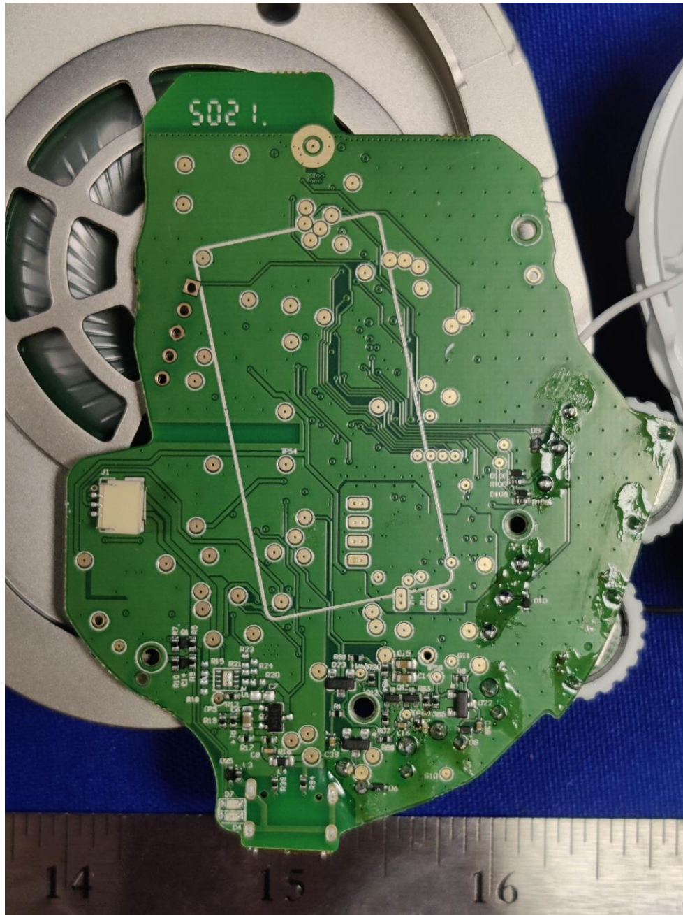
Figure 4: Internal Photo of Stealth600P-USB-RX – Bottom PCB
