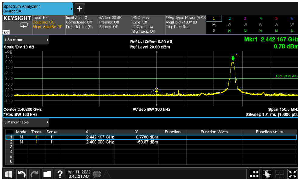
Figure 35: Conducted Band Edge - 2442 MHz at 2 Mbps
