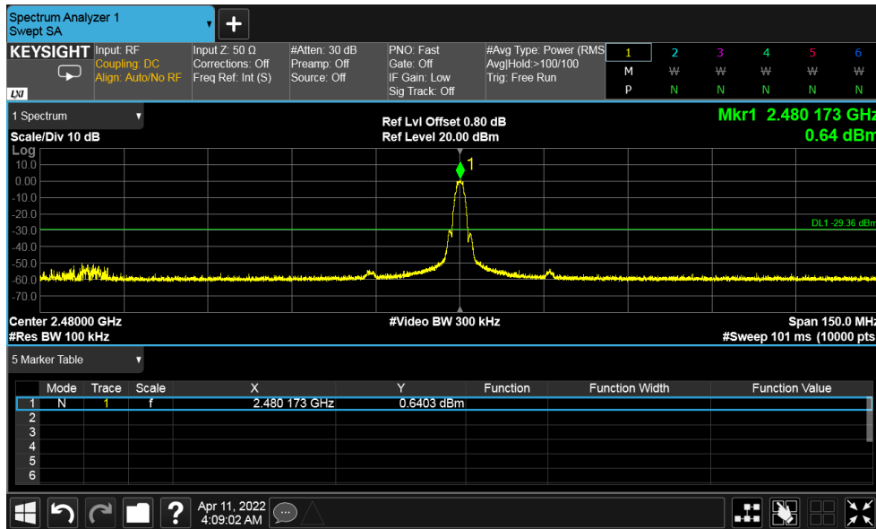
Figure 37: Conducted Band Edge - 2480 MHz at 2 Mbps
