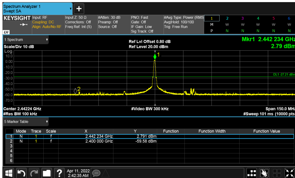
Figure 29: Conducted Band Edge - 2442 MHz at 1 Mbps
