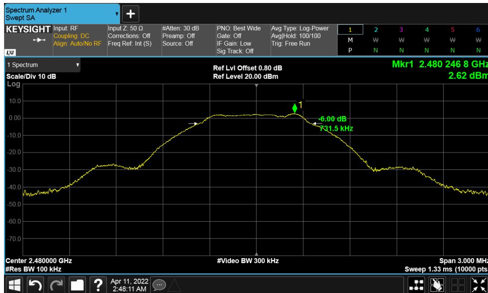
Figure 11: DTS Bandwidth 2480 MHz at 1 Mbps
