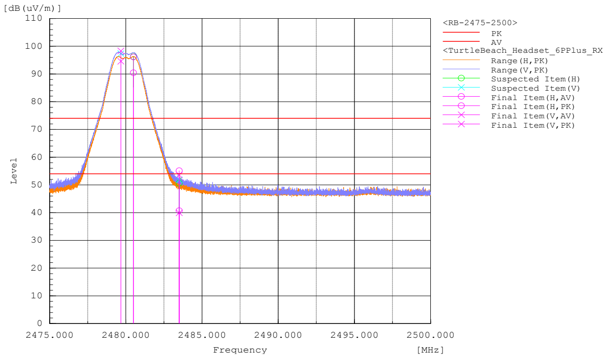
Figure 40: Band-edge-2480 MHz
