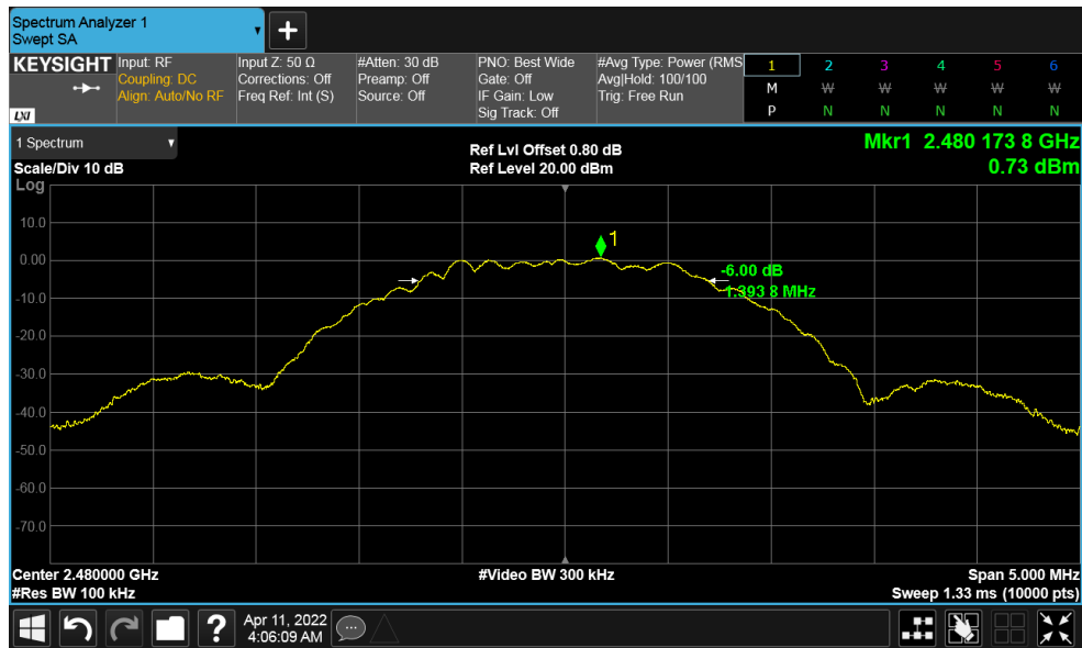
Figure 17: DTS Bandwidth 2480 MHz at 2 Mbps
