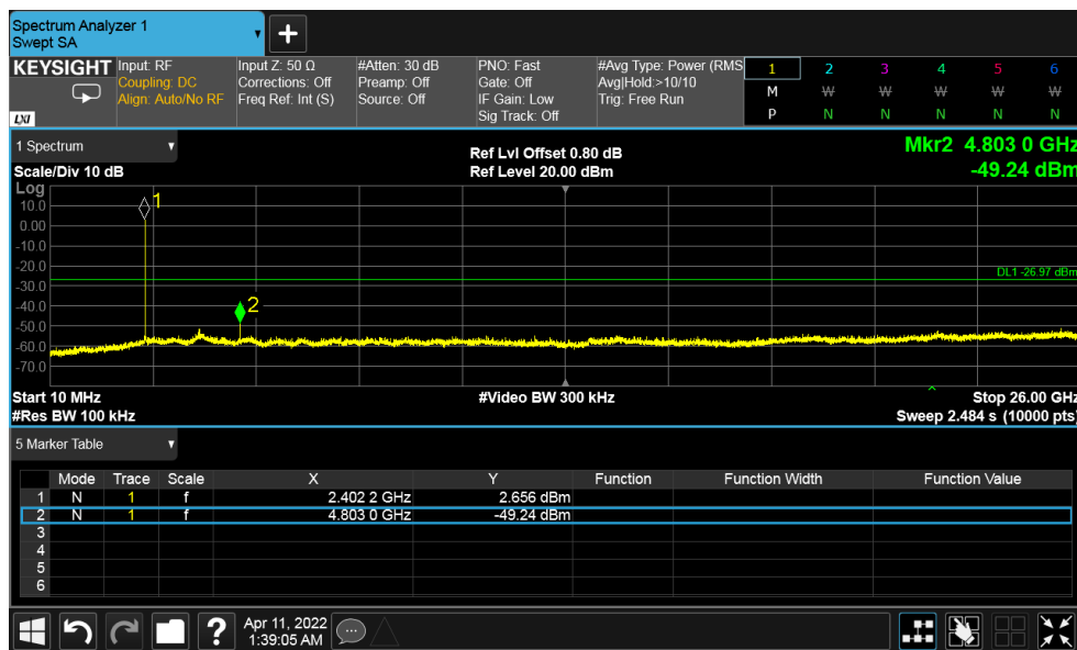
Figure 28: Out of band Emission - 2402 MHz at 1 Mbps
