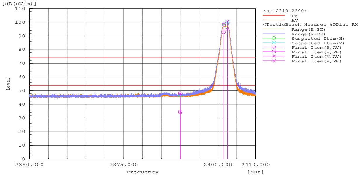
Figure 39: Band-edge-2402 MHz
