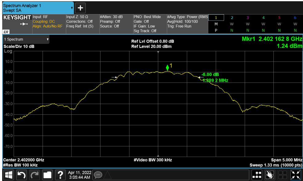
Figure 15: DTS Bandwidth 2402 MHz at 2 Mbps
