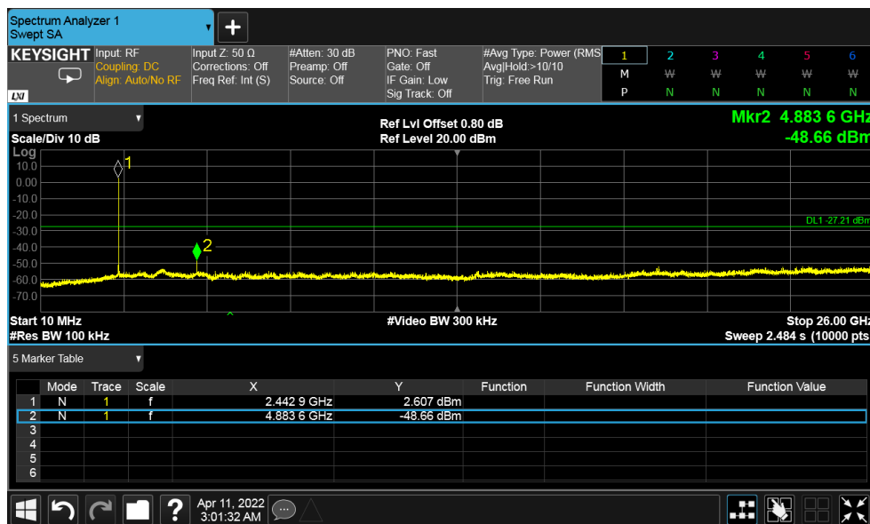
Figure 30: Out of band Emission - 2442 MHz at 1 Mbps
