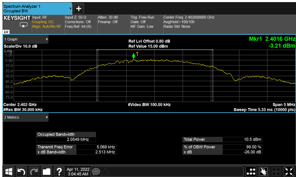
Figure 18: 99% Bandwidth 2402 MHz at 2 Mbps
