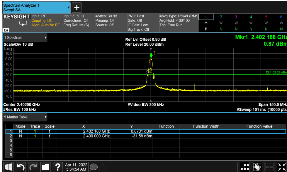
Figure 33: Conducted Band Edge - 2402 MHz at 2 Mbps
