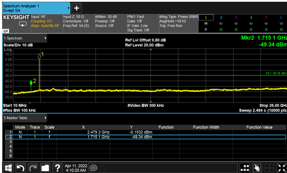
Figure 38: Out of band Emission - 2480 MHz at 2 Mbps
