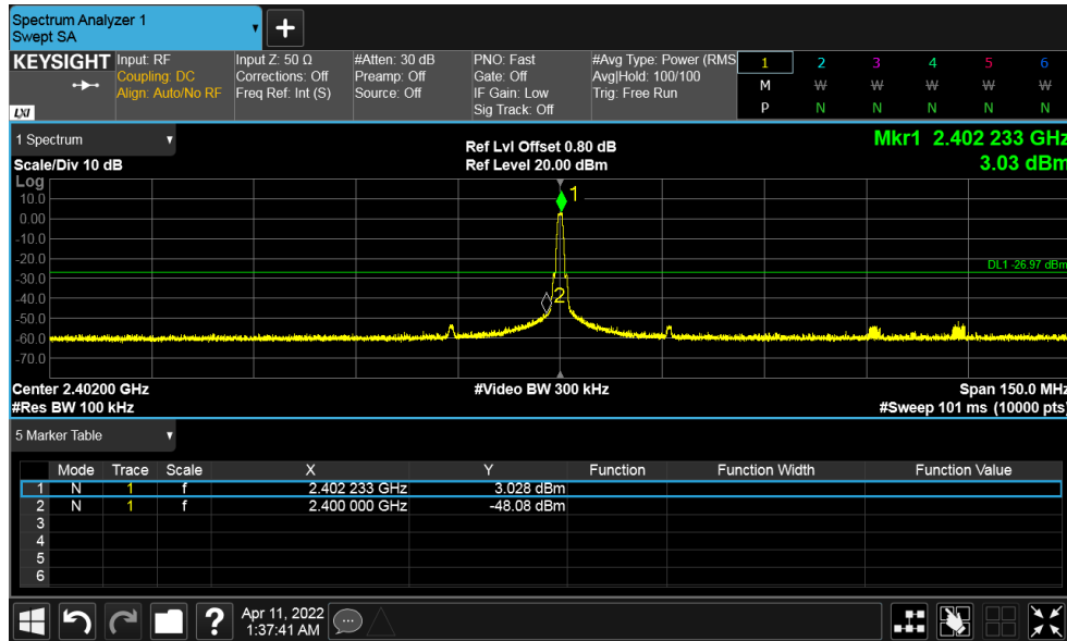
Figure 27: Conducted Band Edge - 2402 MHz at 1 Mbps
