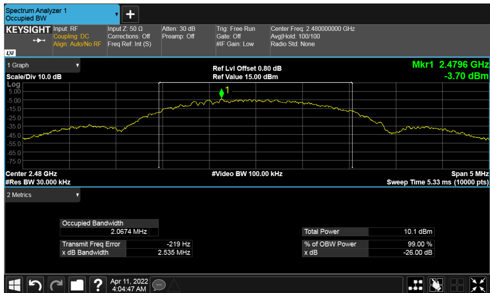
Figure 20: 99% Bandwidth 2480 MHz at 2 Mbps
