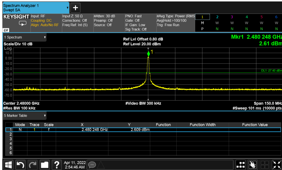
Figure 31: Conducted Band Edge - 2480 MHz at 1 Mbps
