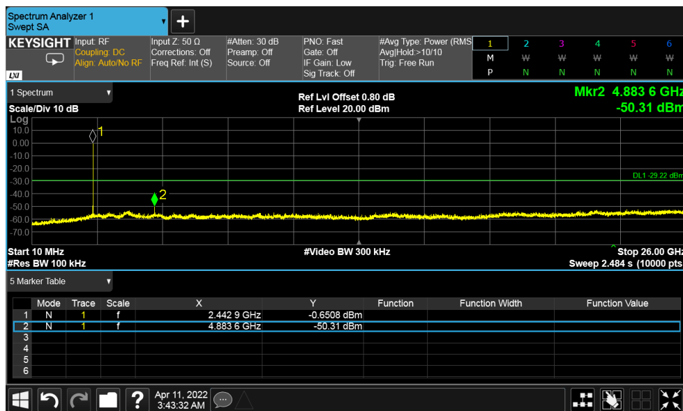
Figure 36: Out of band Emission - 2442 MHz at 2 Mbps
