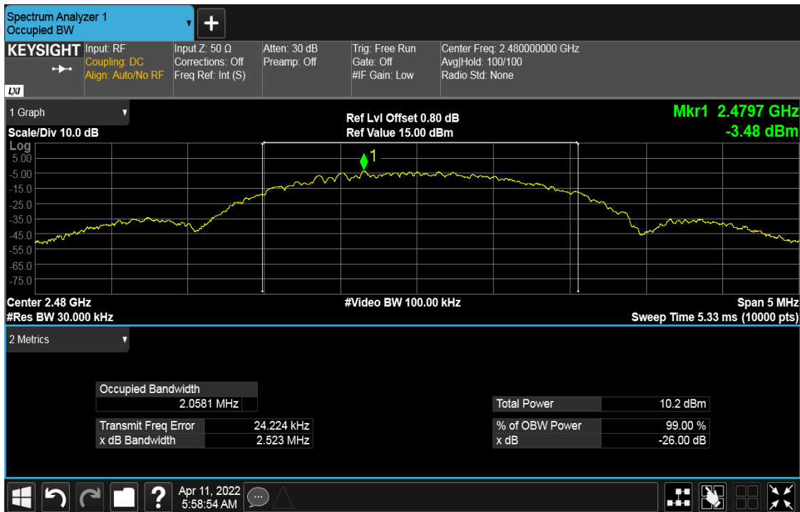
Figure 20: 99% Bandwidth 2480 MHz at 2 Mbps
