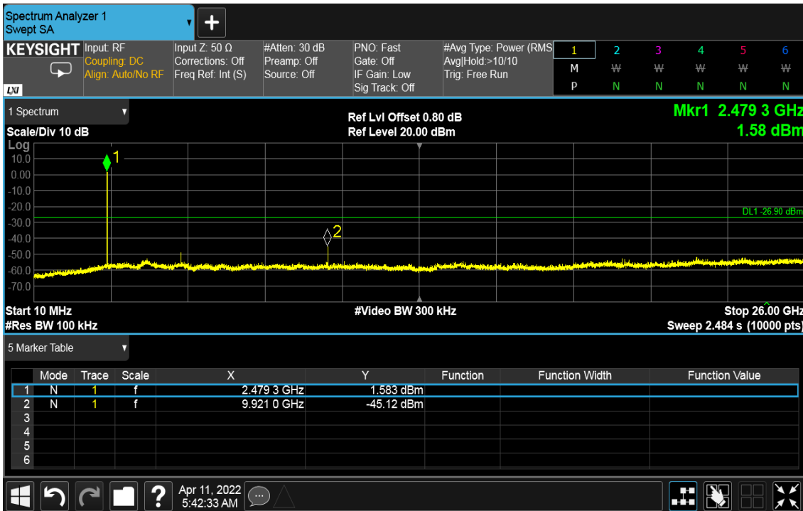
Figure 32: Out of band Emission - 2480 MHz at 1 Mbps
