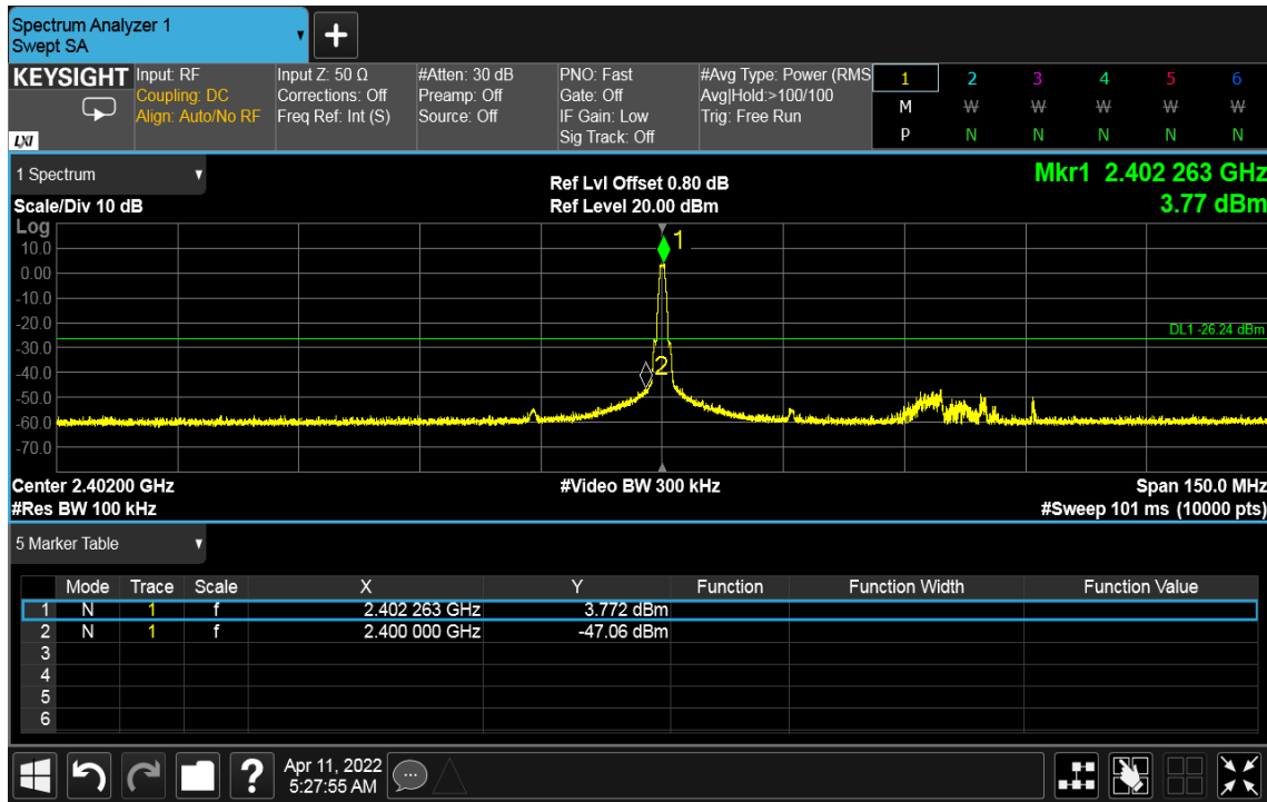
Figure 27: Conducted Band Edge - 2402 MHz at 1 Mbps
