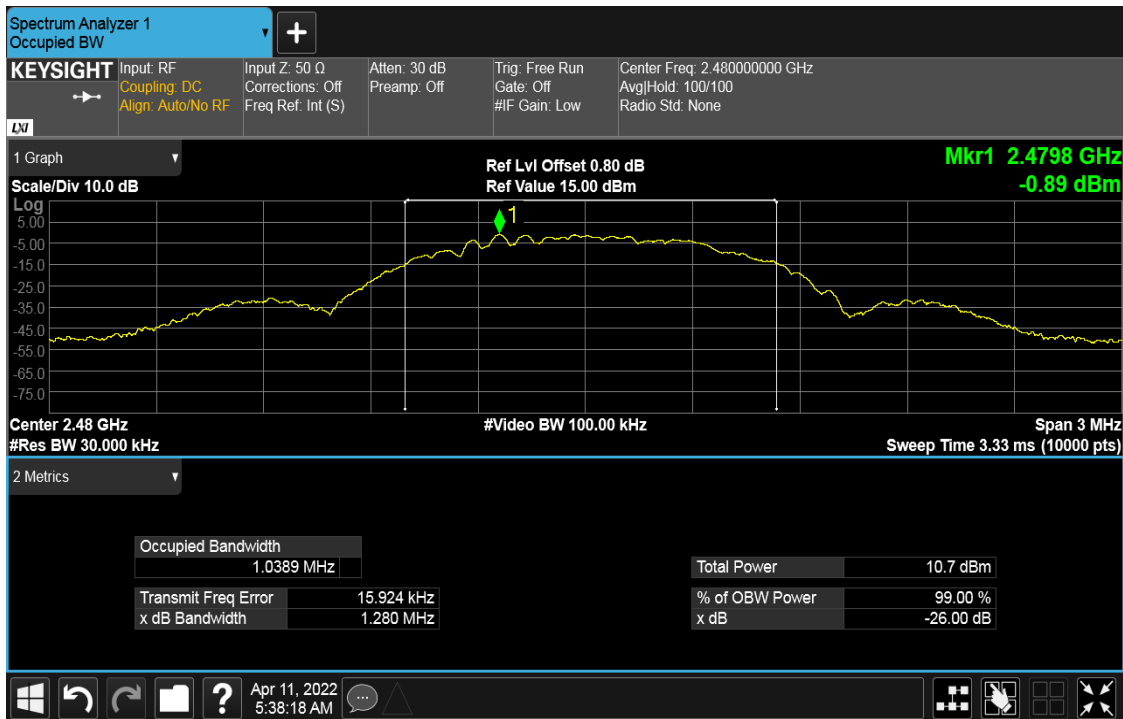
Figure 14: 99% Bandwidth 2480 MHz at 1Mbps
