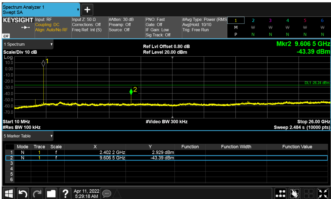
Figure 28: Out of band Emission - 2402 MHz at 1 Mbps
