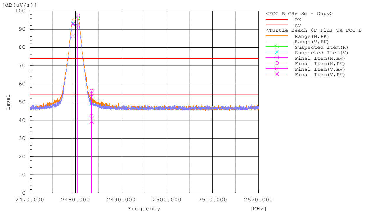
Figure 40: Band-edge-2480 MHz
