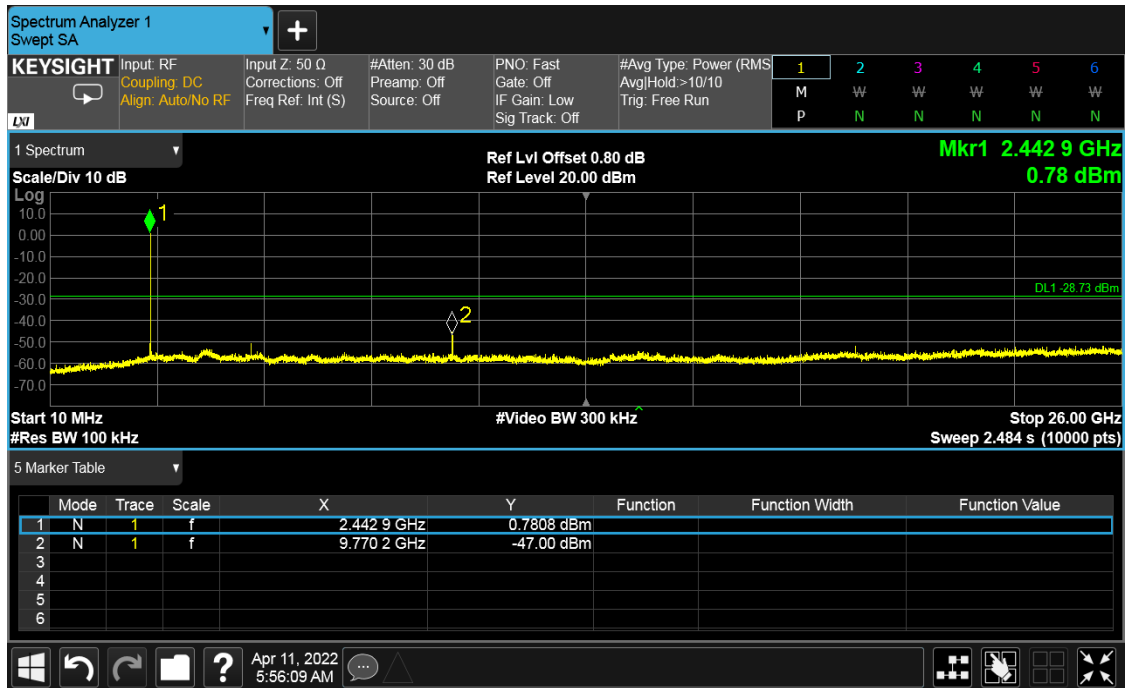
Figure 36: Out of band Emission - 2442 MHz at 2 Mbps
