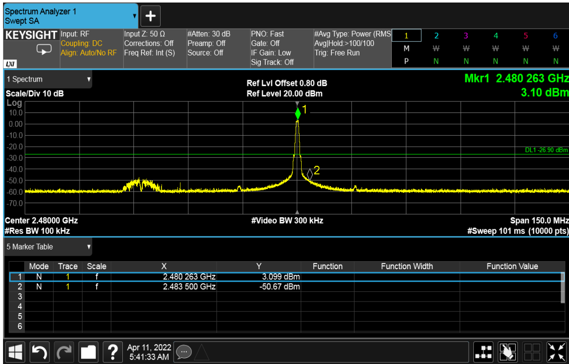
Figure 31: Conducted Band Edge - 2480 MHz at 1 Mbps
