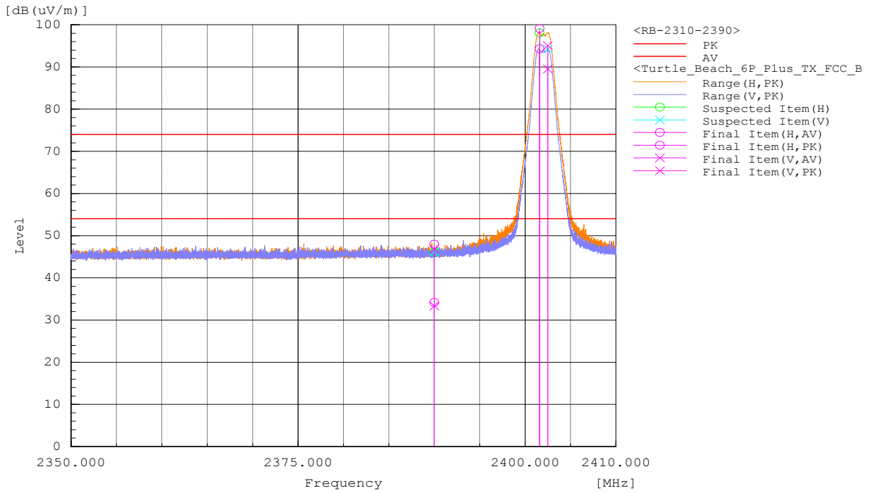
Figure 39: Band-edge-2402 MHz
