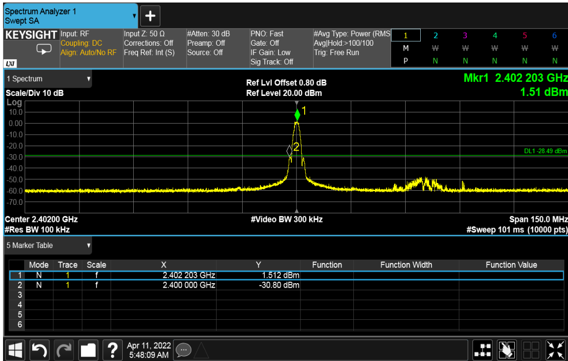
Figure 33: Conducted Band Edge - 2402 MHz at 2 Mbps
