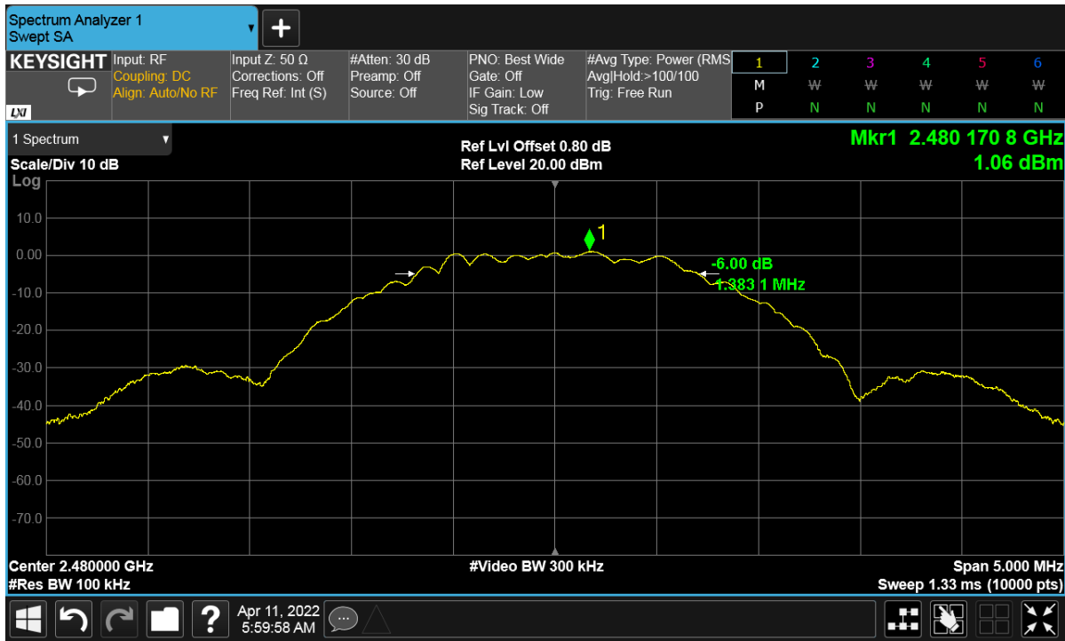
Figure 17: DTS Bandwidth 2480 MHz at 2 Mbps
