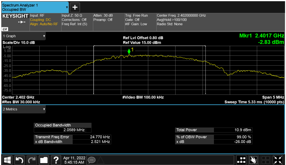
Figure 18: 99% Bandwidth 2402 MHz at 2 Mbps
