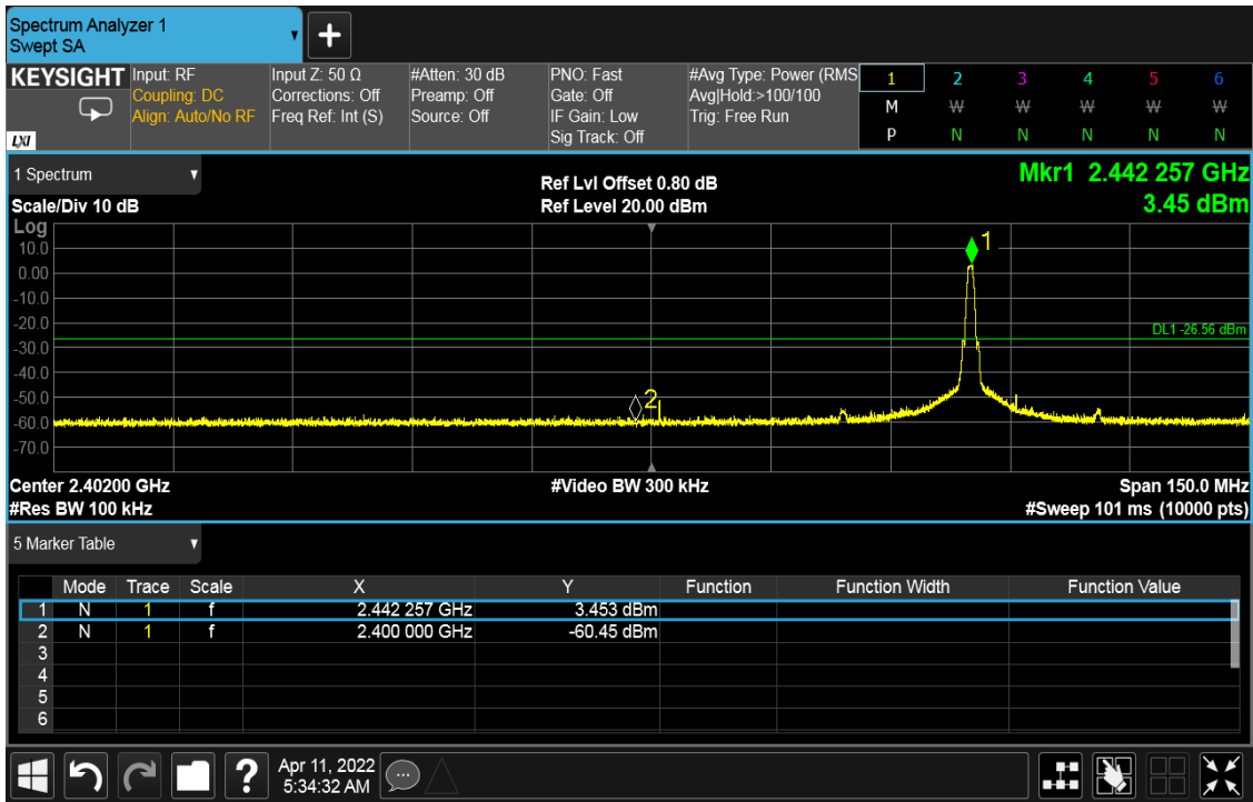
Figure 29: Conducted Band Edge - 2442 MHz at 1 Mbps
