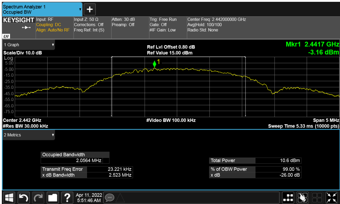
Figure 19: 99% Bandwidth 2442 MHz at 2 Mbps
