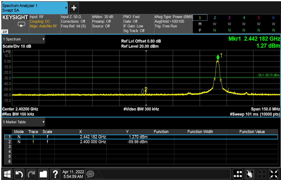
Figure 35: Conducted Band Edge - 2442 MHz at 2 Mbps
