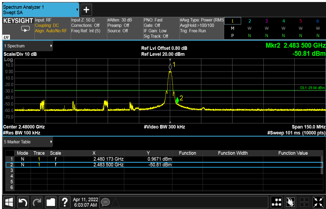
Figure 37: Conducted Band Edge - 2480 MHz at 2 Mbps
