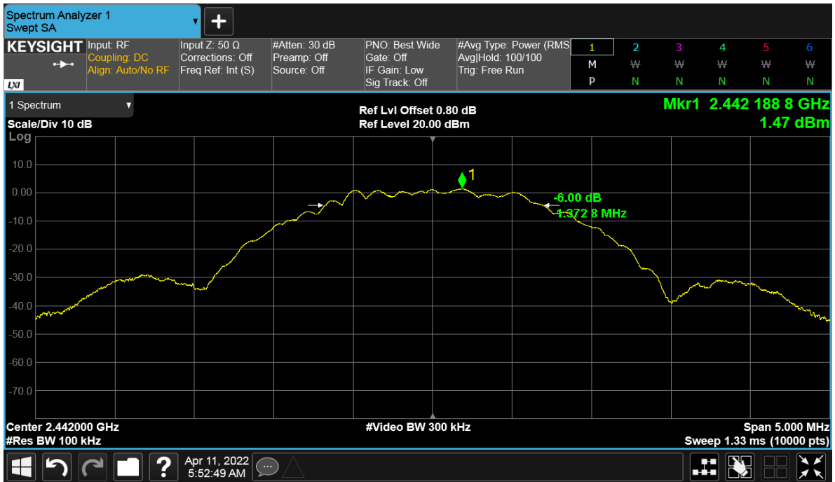
Figure 16: DTS Bandwidth 2442 MHz at 2 Mbps
