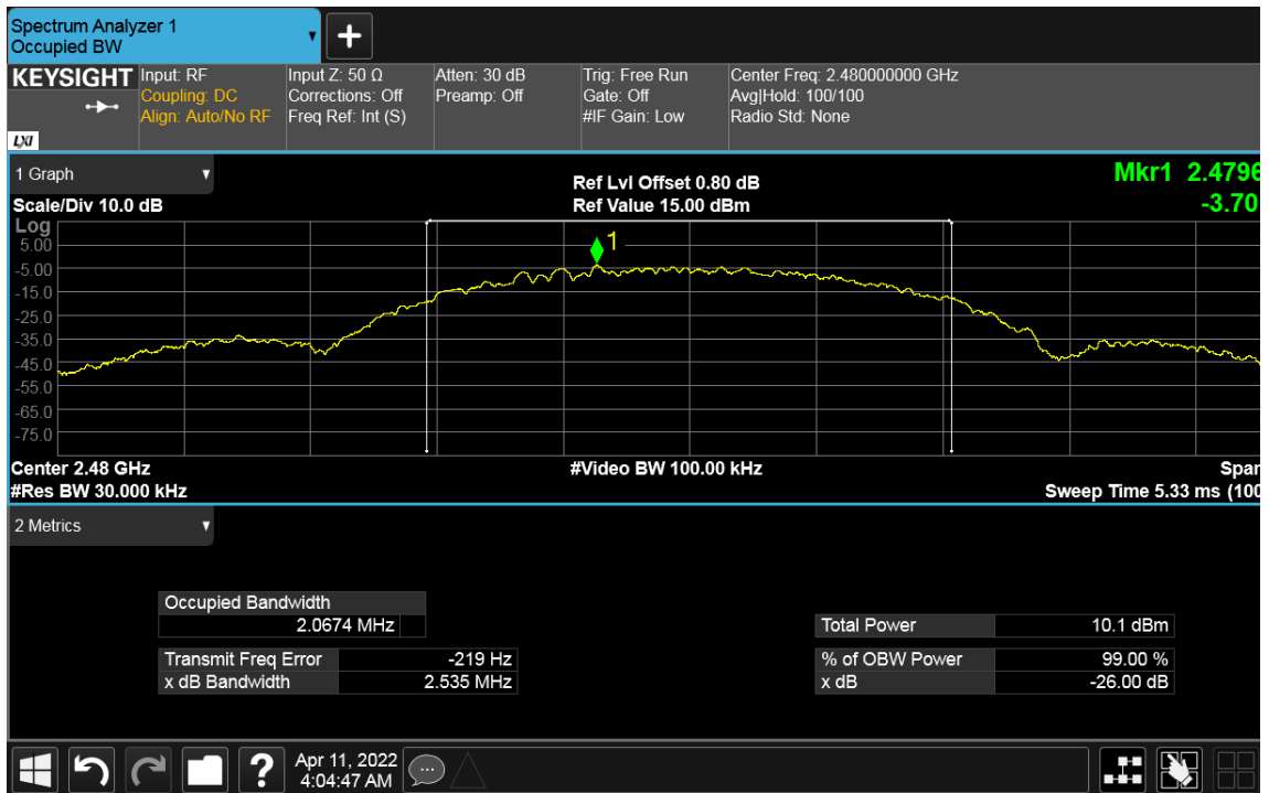
Figure 20: 99% Bandwidth 2480 MHz at 2 Mbps
