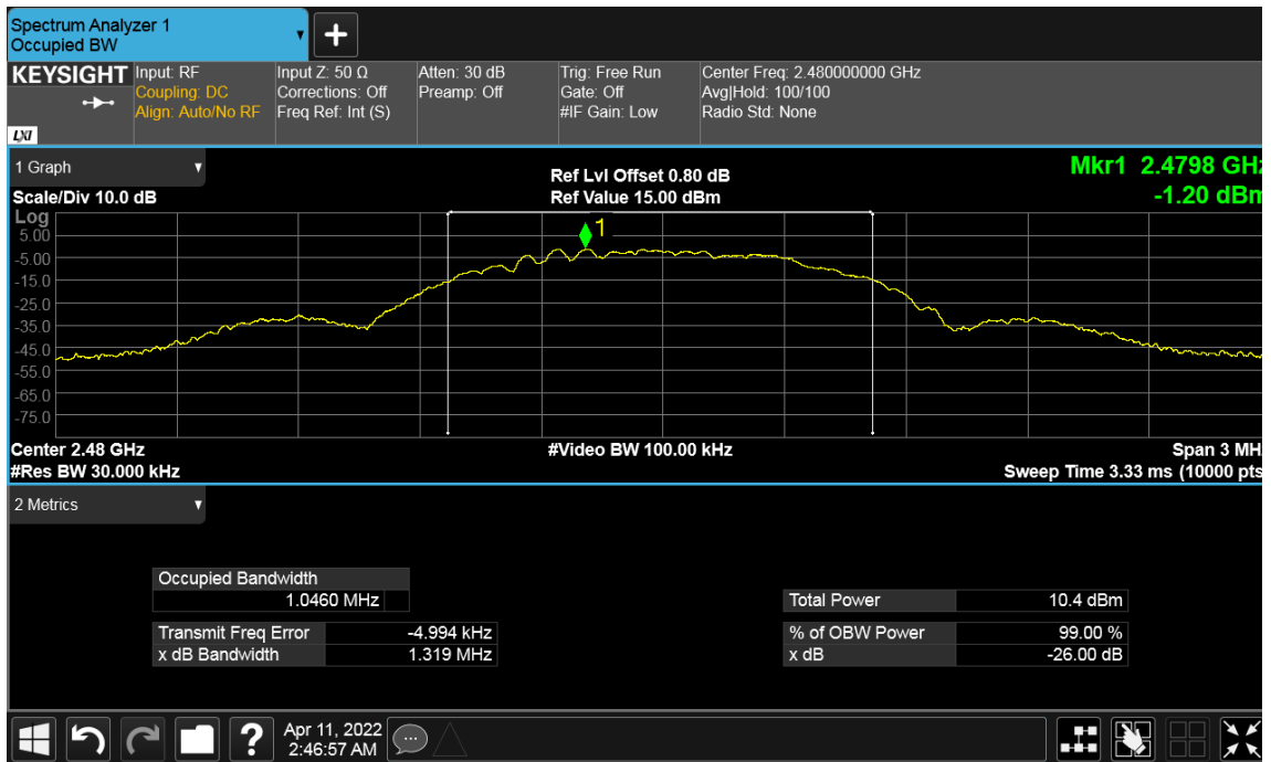
Figure 14: 99% Bandwidth 2480 MHz at 1Mbps
