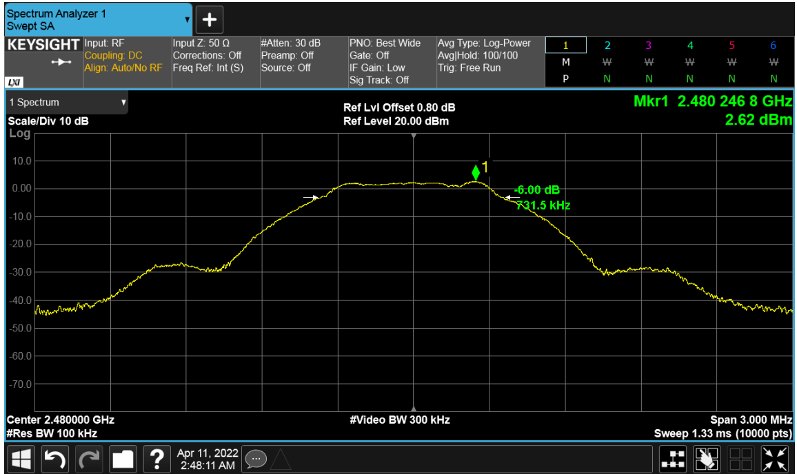
Figure 11: DTS Bandwidth 2480 MHz at 1 Mbps
