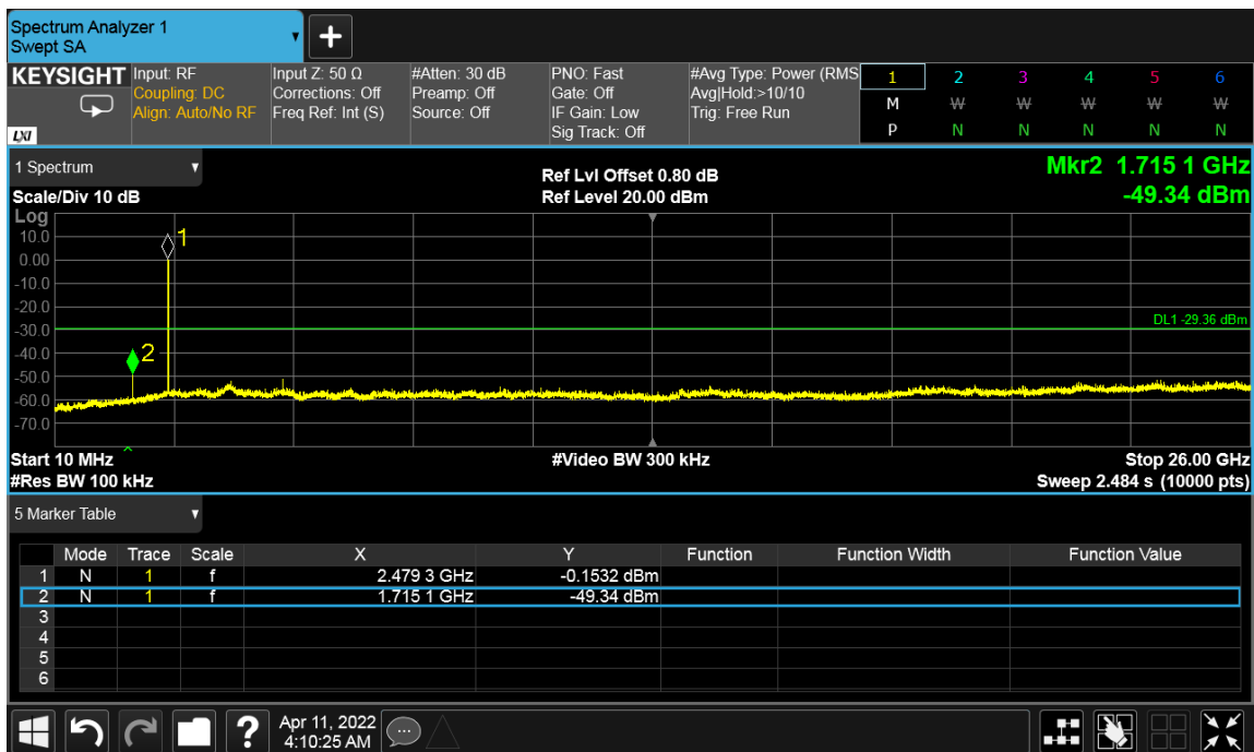
Figure 38: Out of band Emission - 2480 MHz at 2 Mbps
