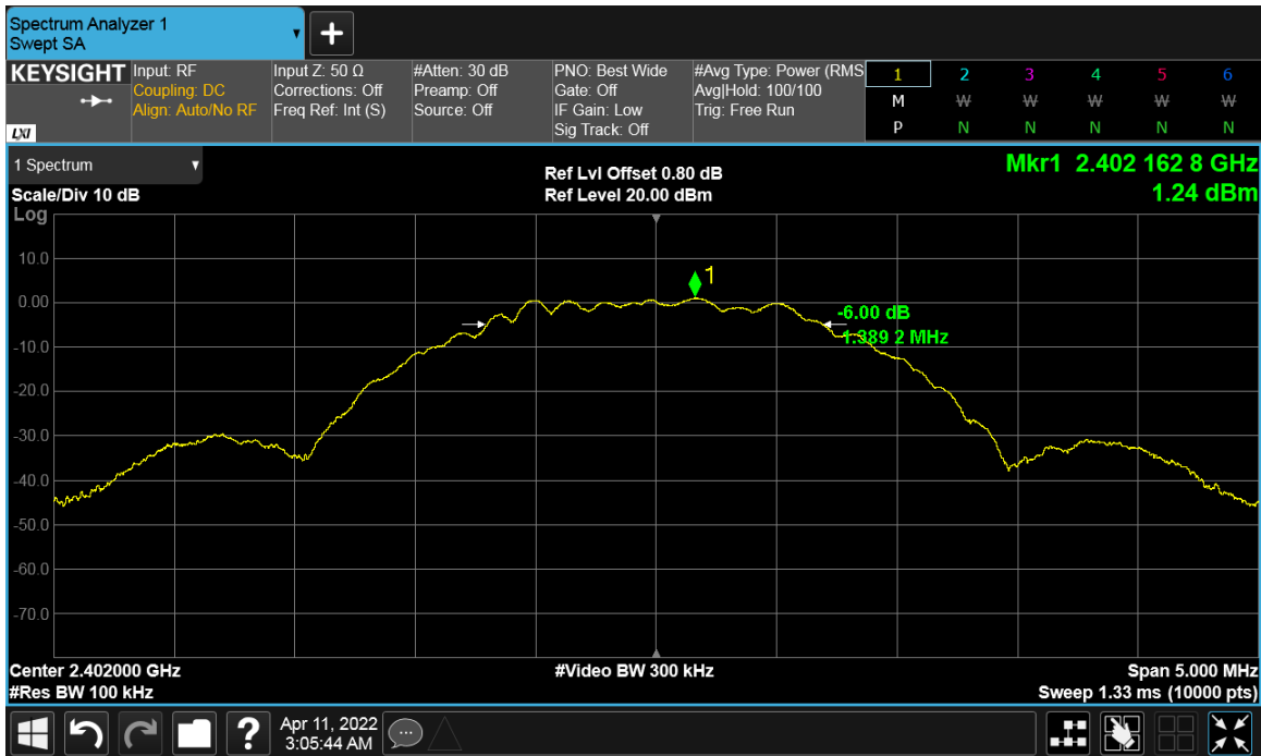
Figure 15: DTS Bandwidth 2402 MHz at 2 Mbps
