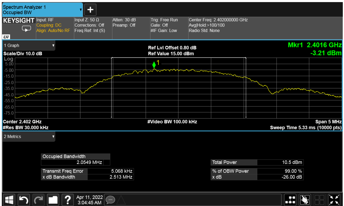
Figure 18: 99% Bandwidth 2402 MHz at 2 Mbps
