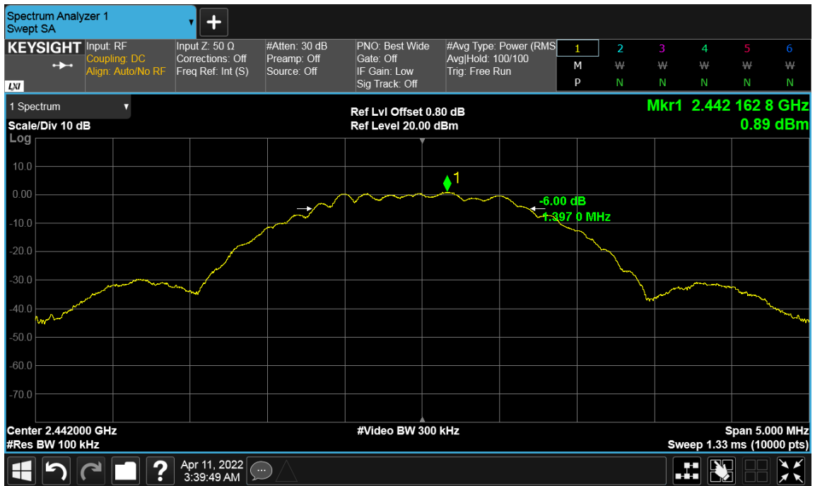
Figure 16: DTS Bandwidth 2442 MHz at 2 Mbps
