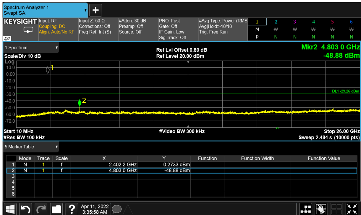
Figure 34: Out of band Emission - 2402 MHz at 2 Mbps
