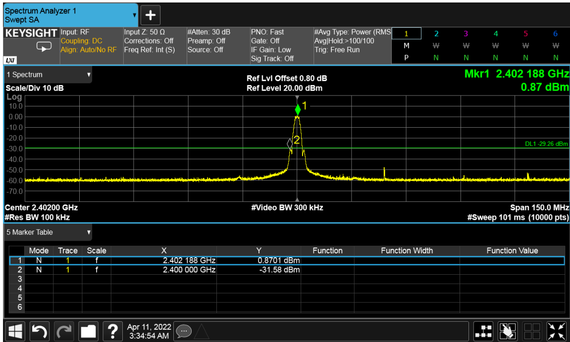
Figure 33: Conducted Band Edge - 2402 MHz at 2 Mbps
