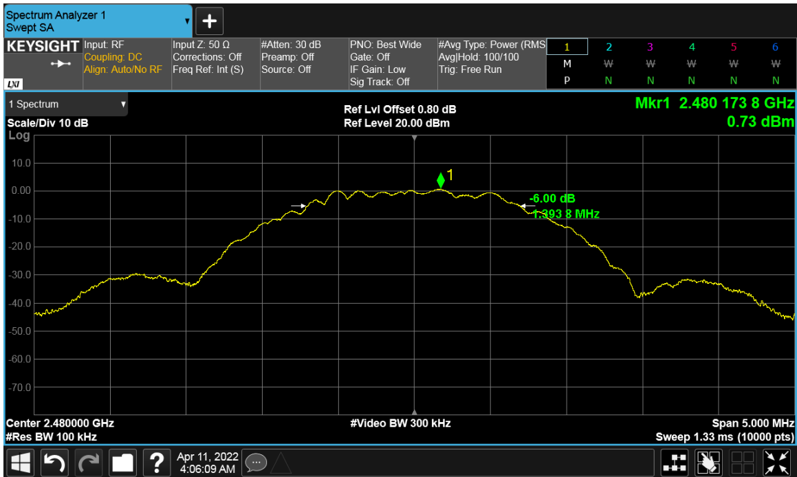
Figure 17: DTS Bandwidth 2480 MHz at 2 Mbps
