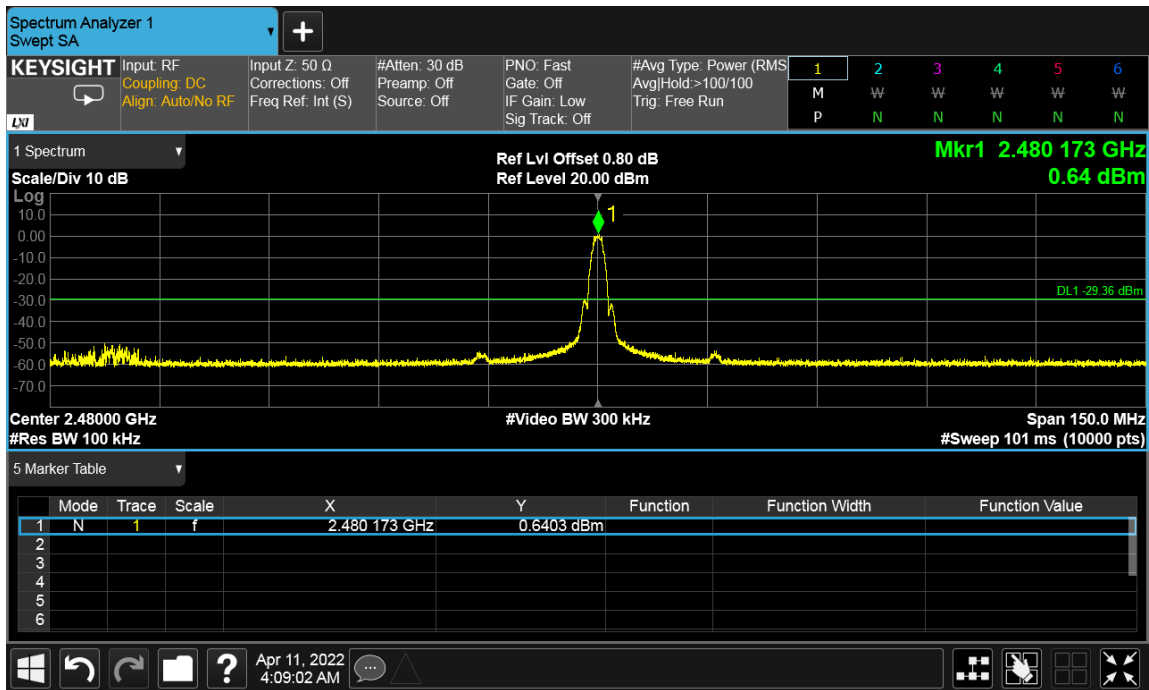
Figure 37: Conducted Band Edge - 2480 MHz at 2 Mbps
