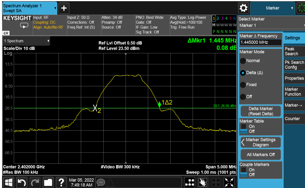
Figure 26: Conducted Band Edge - 2402 MHz at 1 Mbps
