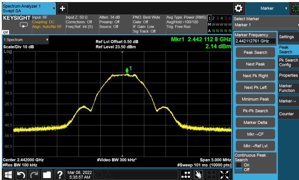
Figure 21: Maximum Power Spectral Density-2442 MHz at 1 Mbps
