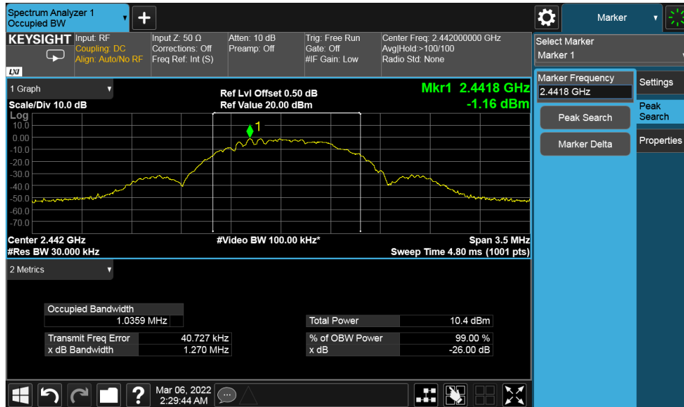
Figure 12: 99% Bandwidth 2442 MHz at 1Mbps
