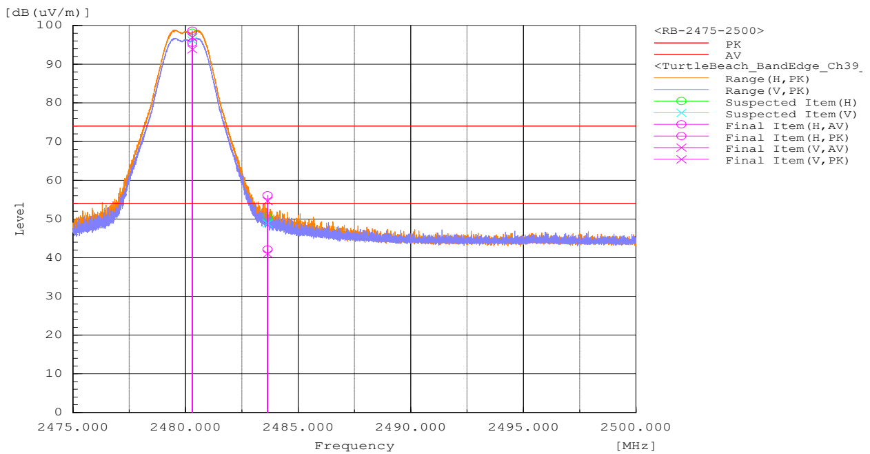
Figure 39: Band-edge-2480 MHz
