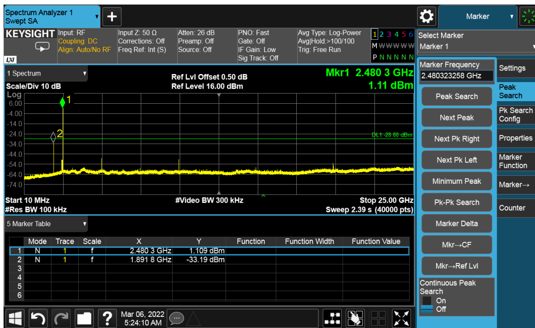
Figure 37: Out of band Emission - 2480 MHz at 2 Mbps
