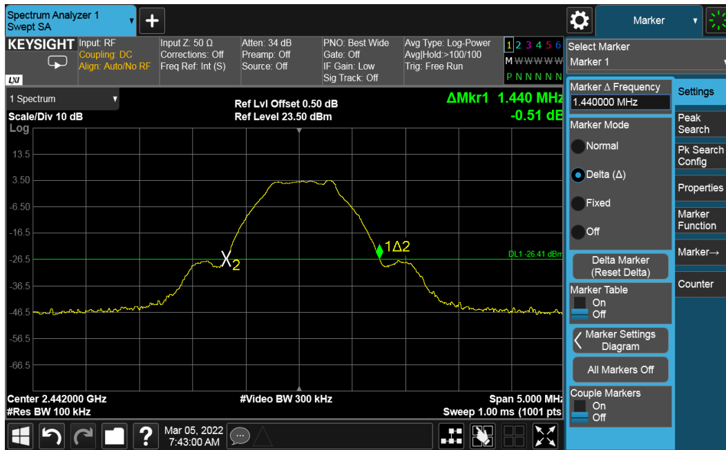
Figure 28: Conducted Band Edge - 2442 MHz at 1 Mbps
