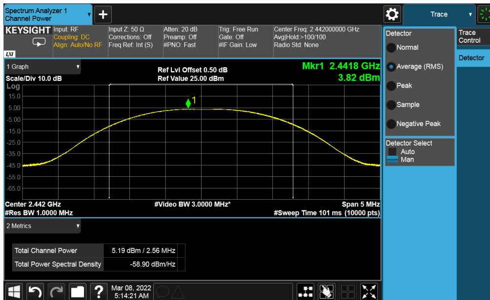
Figure 3: Maximum Conducted Output Power at 2442 MHz at 1Mbps
