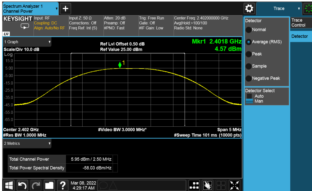
Figure 2: Maximum Transmitted Power, 2402 MHz at 1Mbps
