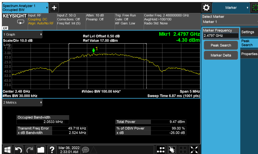
Figure 19: 99% Bandwidth 2480 MHz at 2 Mbps
