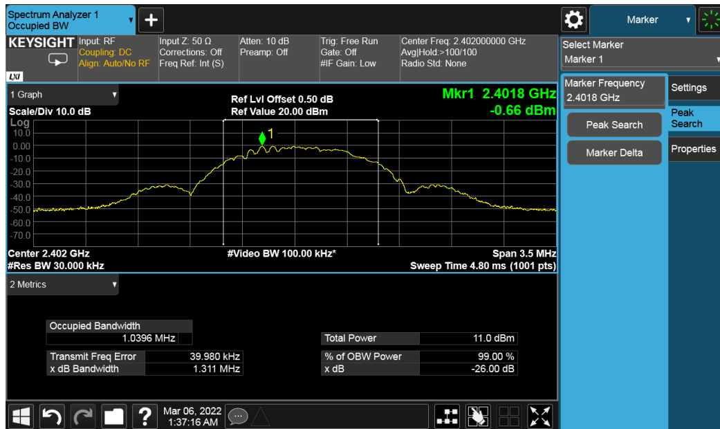
Figure 11: 99% Bandwidth 2402 MHz at 1Mbps
