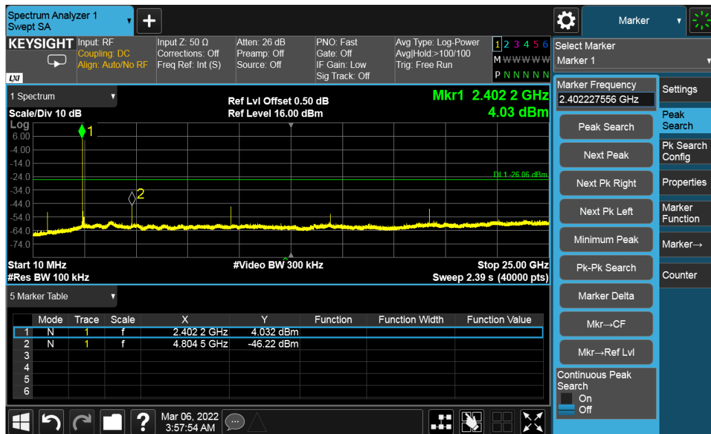
Figure 27: Out of band Emission - 2402 MHz at 1 Mbps
