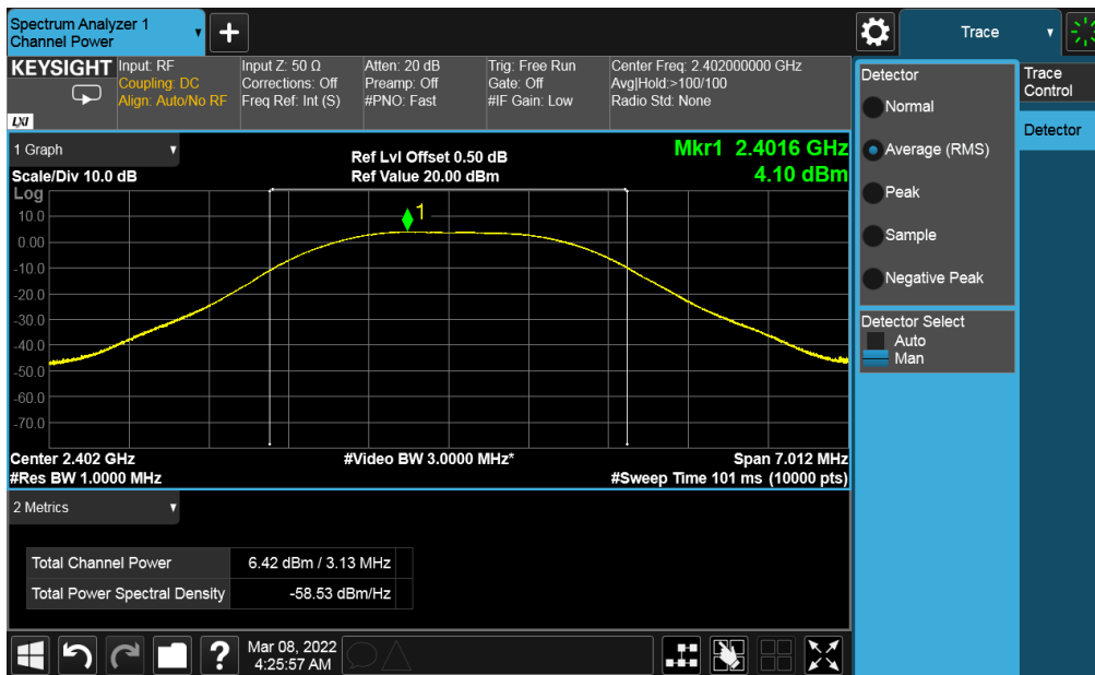
Figure 5: Maximum Conducted Output Power at 2402 MHz at 2Mbps
