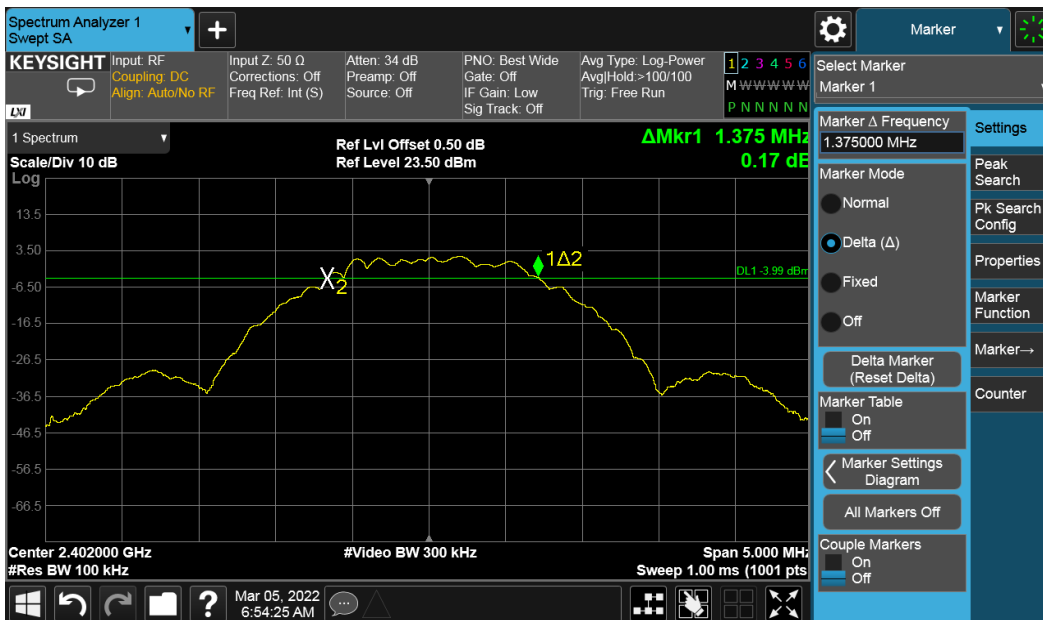
Figure 14: DTS Bandwidth 2402 MHz at 2 Mbps
