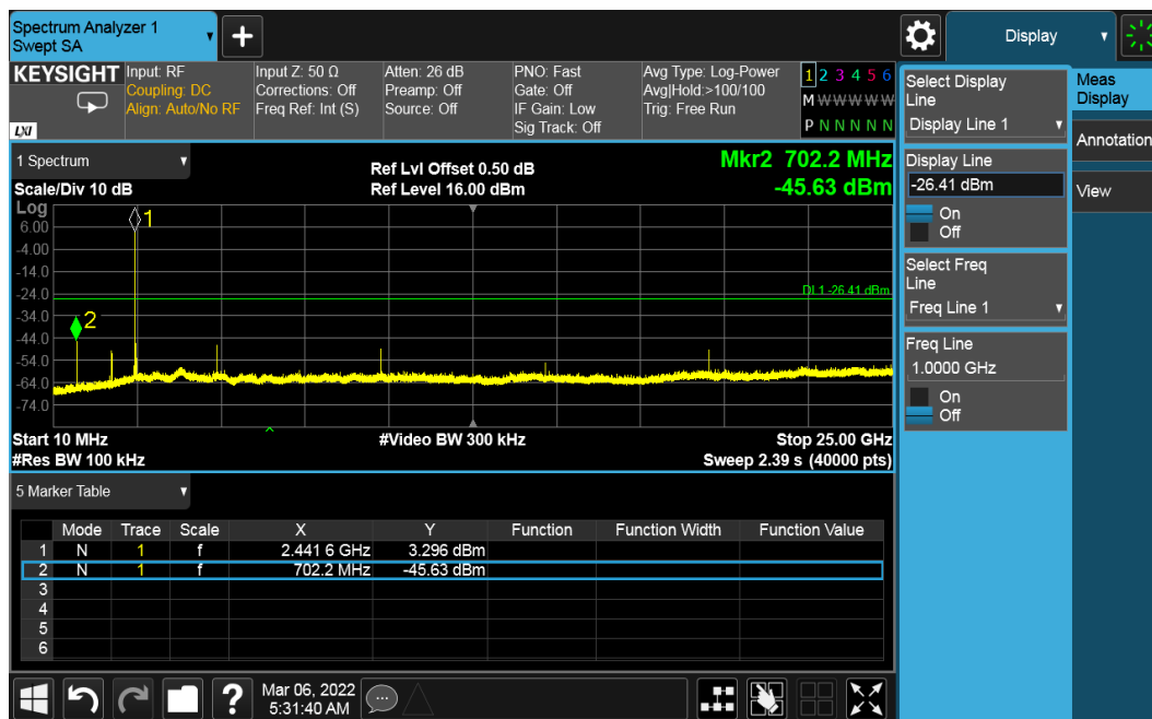
Figure 29: Out of band Emission - 2442 MHz at 1 Mbps
