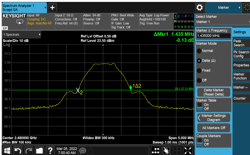
Figure 30: Conducted Band Edge - 2480 MHz at 1 Mbps
