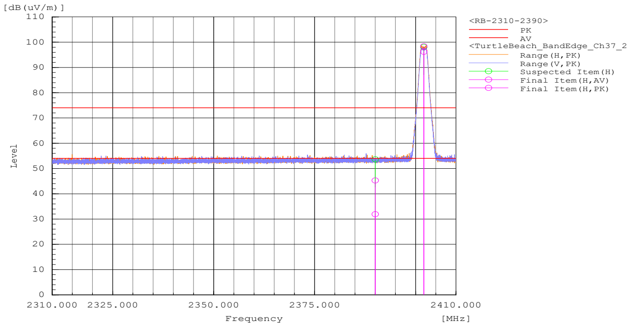
Figure 38: Band-edge-2402 MHz
