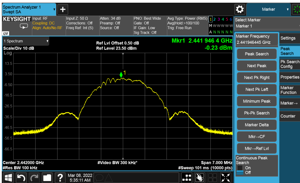
Figure 24: Maximum Power Spectral Density-2442 MHz at 2 Mbps
