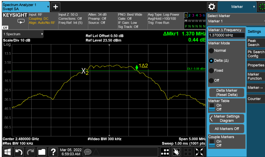
Figure 16: DTS Bandwidth 2480 MHz at 2 Mbps
