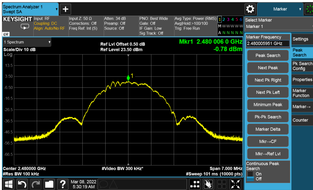
Figure 25: Maximum Power Spectral Density-2480 MHz at 2 Mbps
