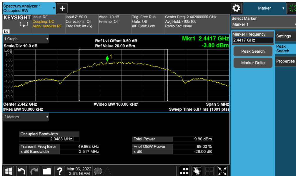
Figure 18: 99% Bandwidth 2442 MHz at 2 Mbps
