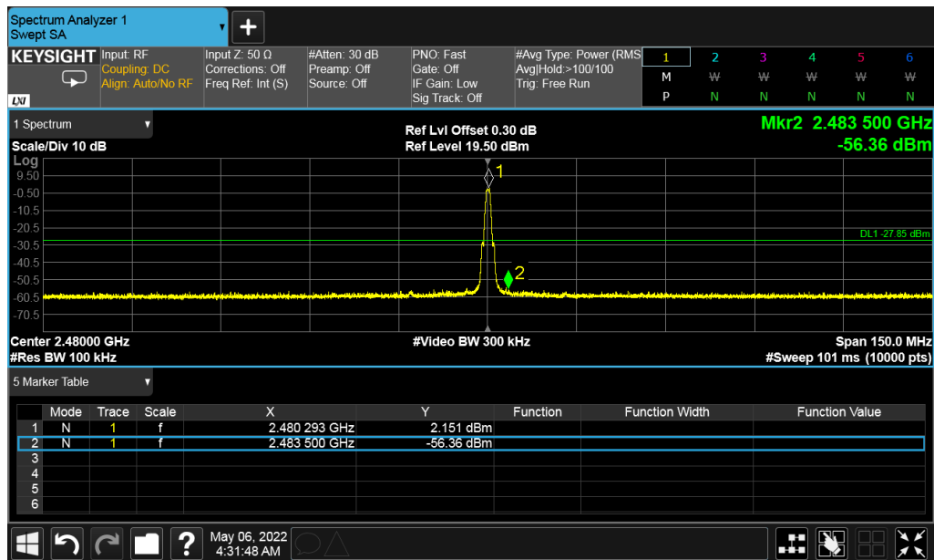
Figure 18: Conducted Band Edge - 2480 MHz
