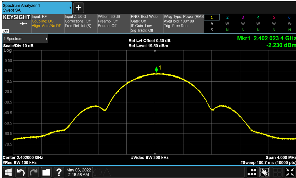
Figure 11: Maximum Power Spectral Density-2402 MHz
