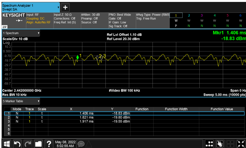
Figure 1: Duty Cycle at 1 Mbps
