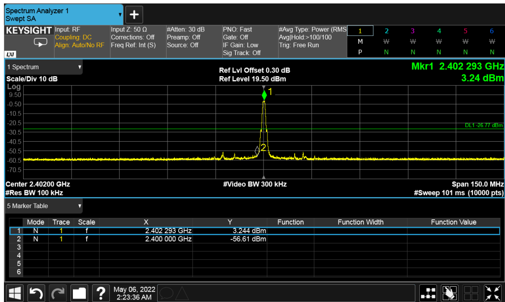
Figure 14: Conducted Band Edge - 2402 MHz at 1 Mbps
