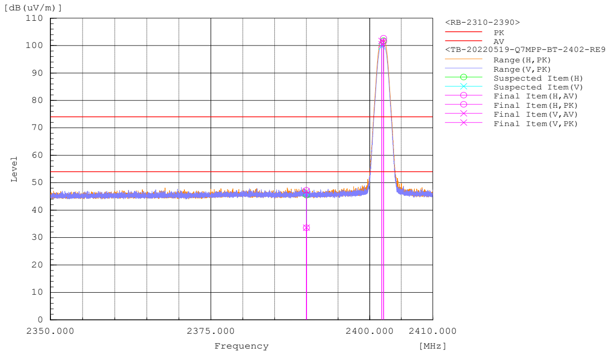
Figure 20: Band-edge-2402 MHz
