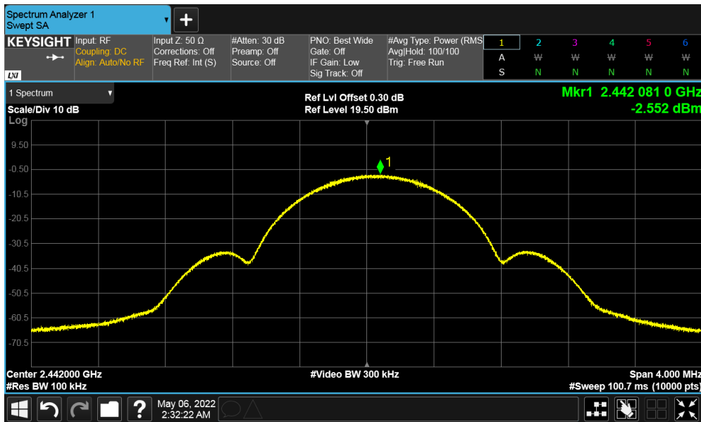
Figure 12: Maximum Power Spectral Density-2442 MHz
