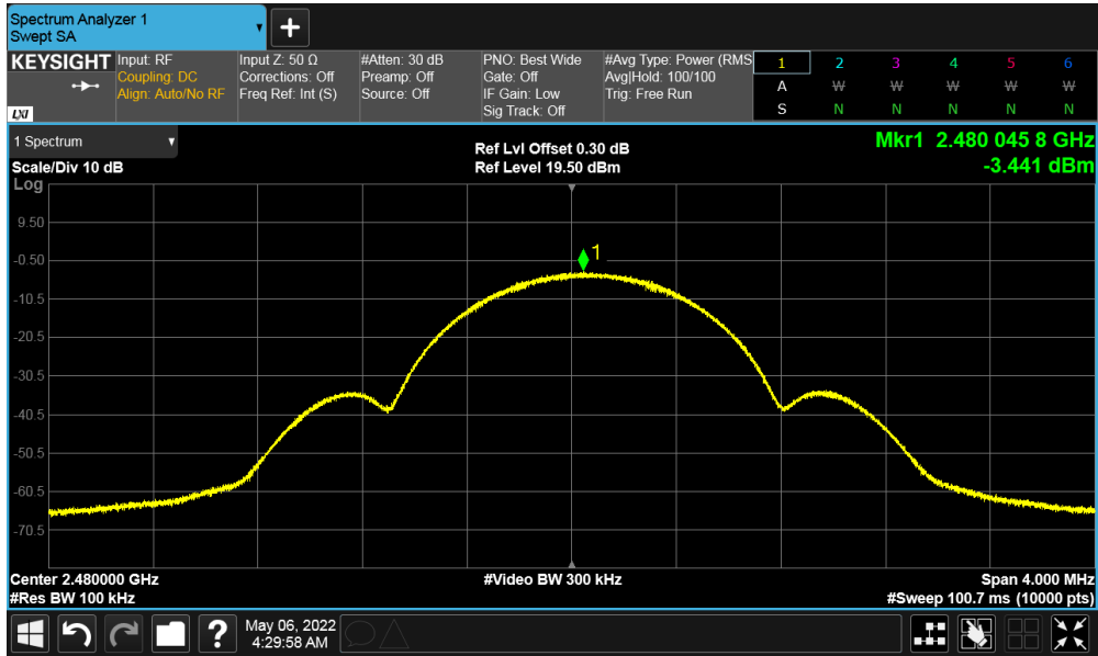
Figure 13: Maximum Power Spectral Density-2480 MHz
