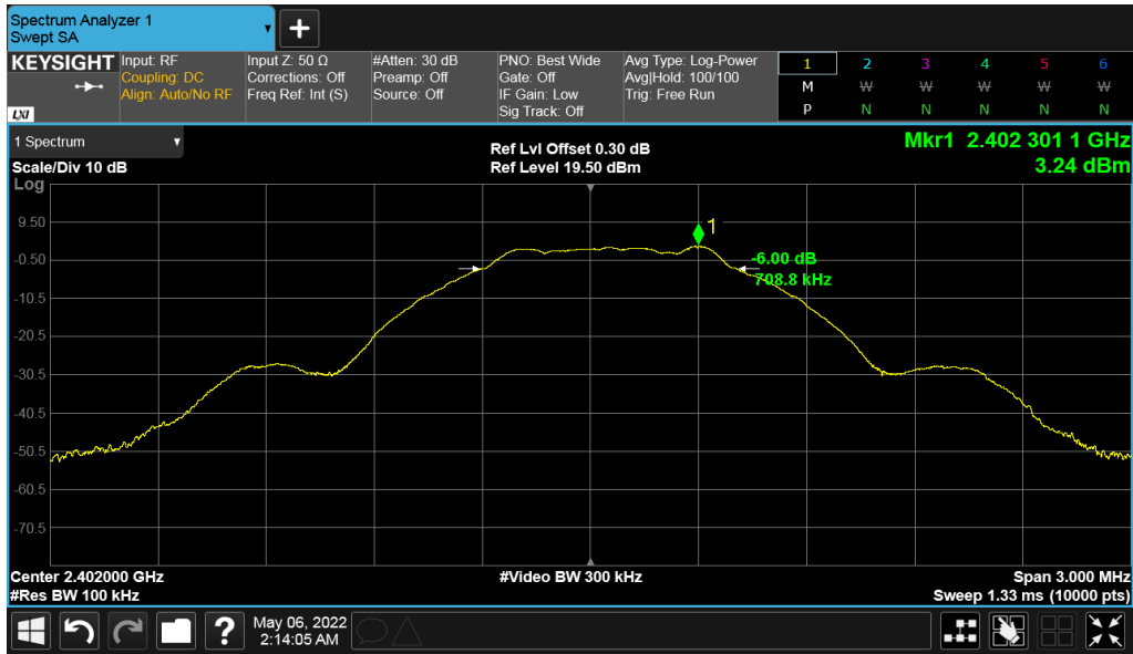
Figure 5: DTS Bandwidth 2402 MHz
