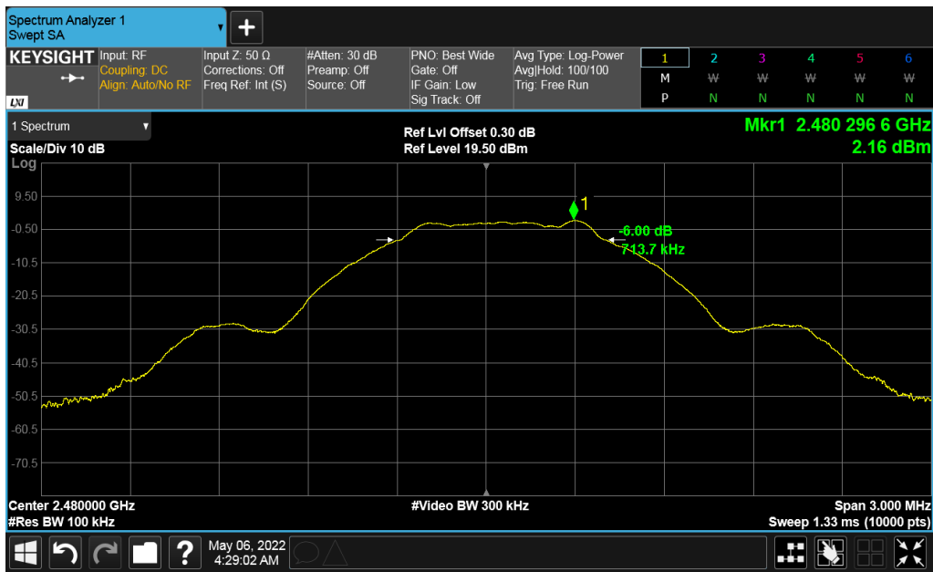
Figure 7: DTS Bandwidth 2480 MHz
