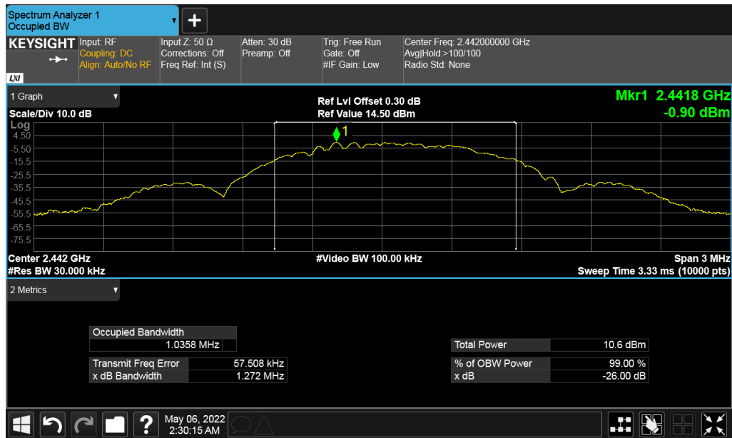
Figure 9: 99% Bandwidth 2442 MHz
