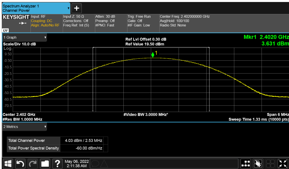
Figure 2: Maximum Conducted Output Power, 2402 MHz
