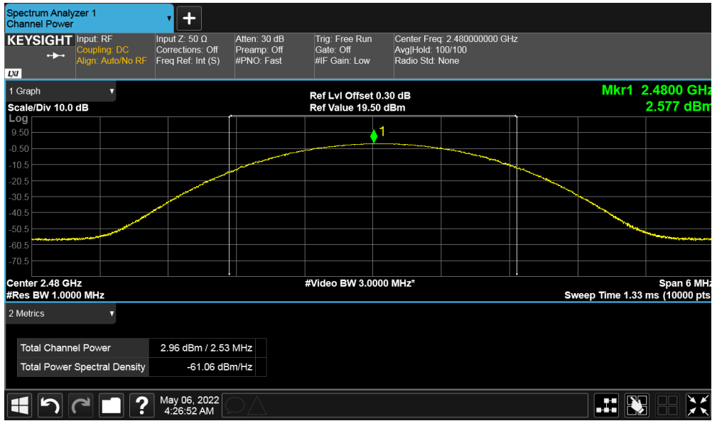
Figure 4: Maximum Conducted Output Power at 2480 MHz
