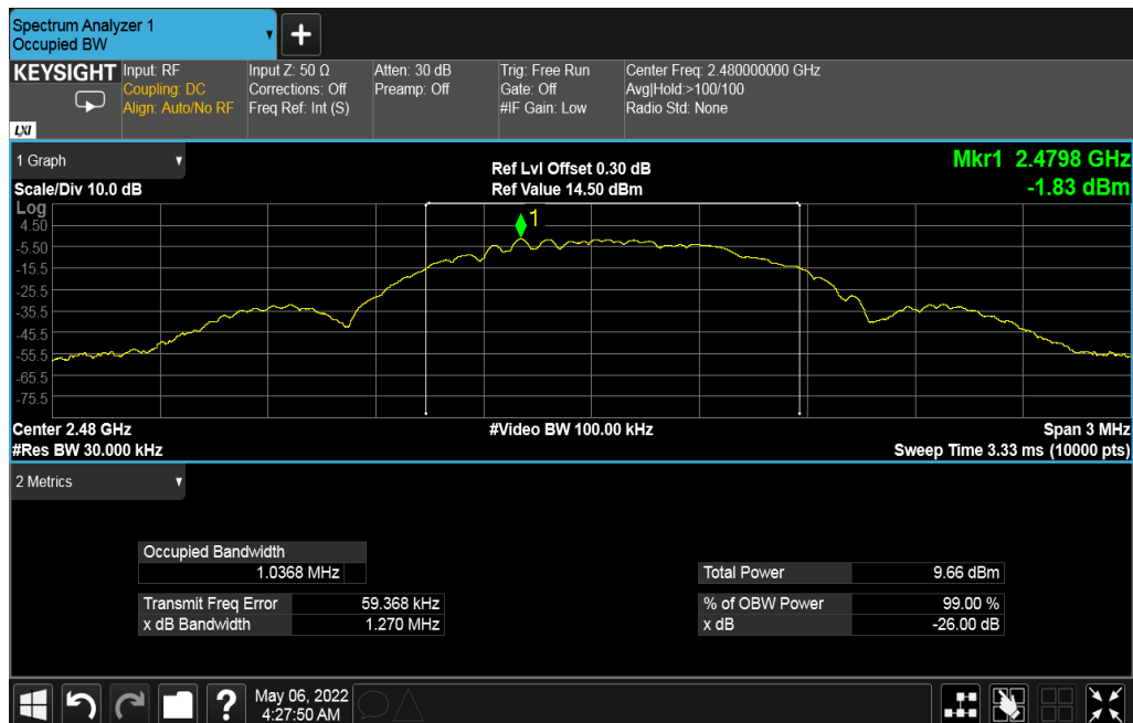
Figure 10: 99% Bandwidth 2480 MHz
