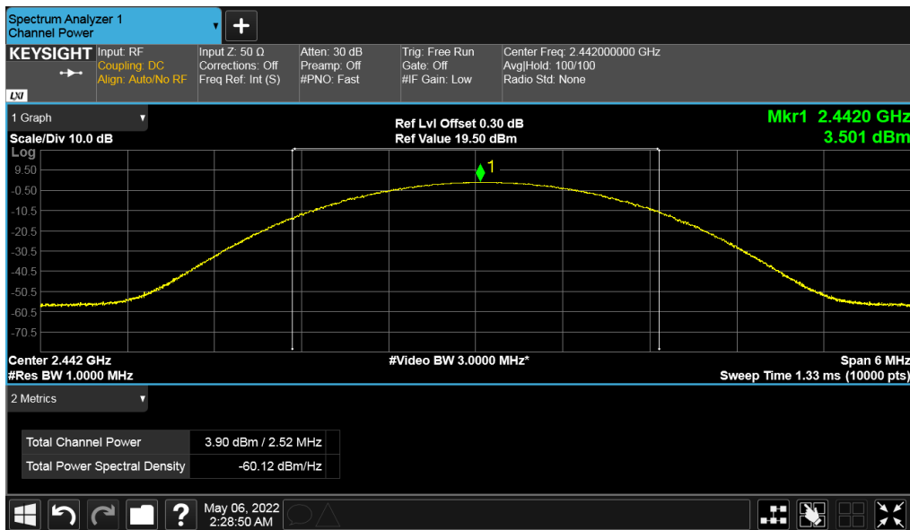
Figure 3: Maximum Conducted Output Power at 2442 MHz
