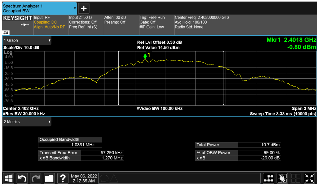
Figure 8: 99% Bandwidth 2402 MHz
