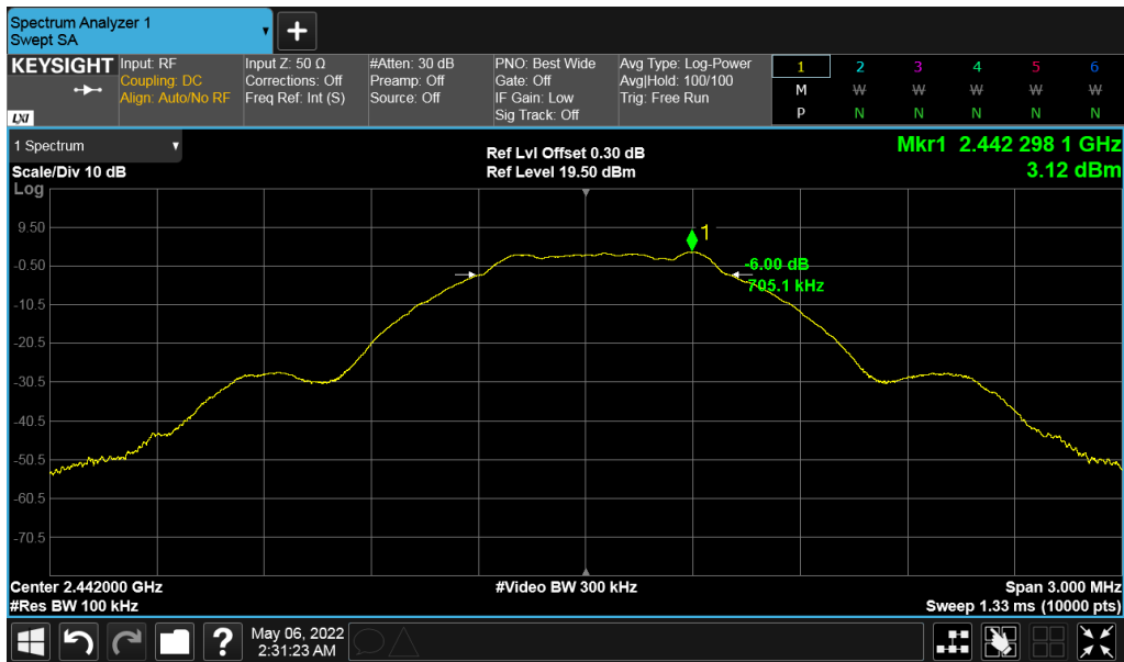
Figure 6: DTS Bandwidth 2442 MHz
