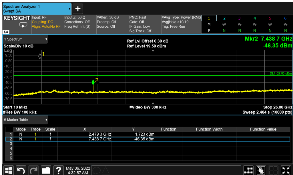
Figure 19: Out of band Emission - 2480 MHz
