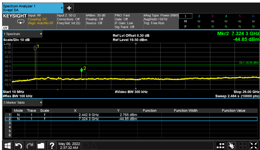
Figure 17: Out of band Emission - 2442 MHz at 1 Mbps
