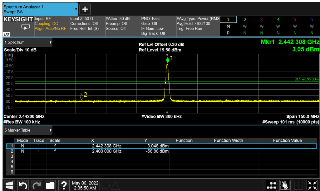
Figure 16: Conducted Band Edge - 2442 MHz at 1 Mbps
