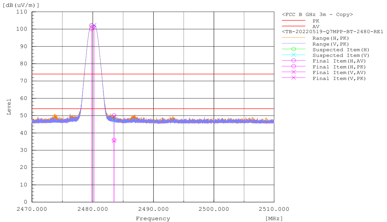
Figure 21: Band-edge-2480 MHz
