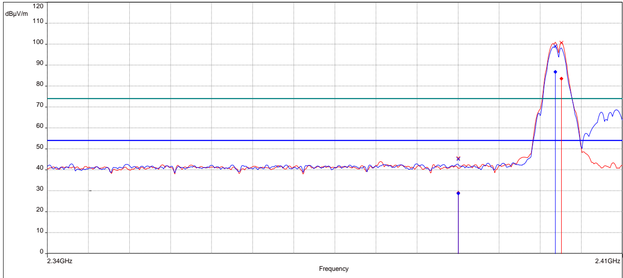
Figure 39: Band-edge-2402 MHz
