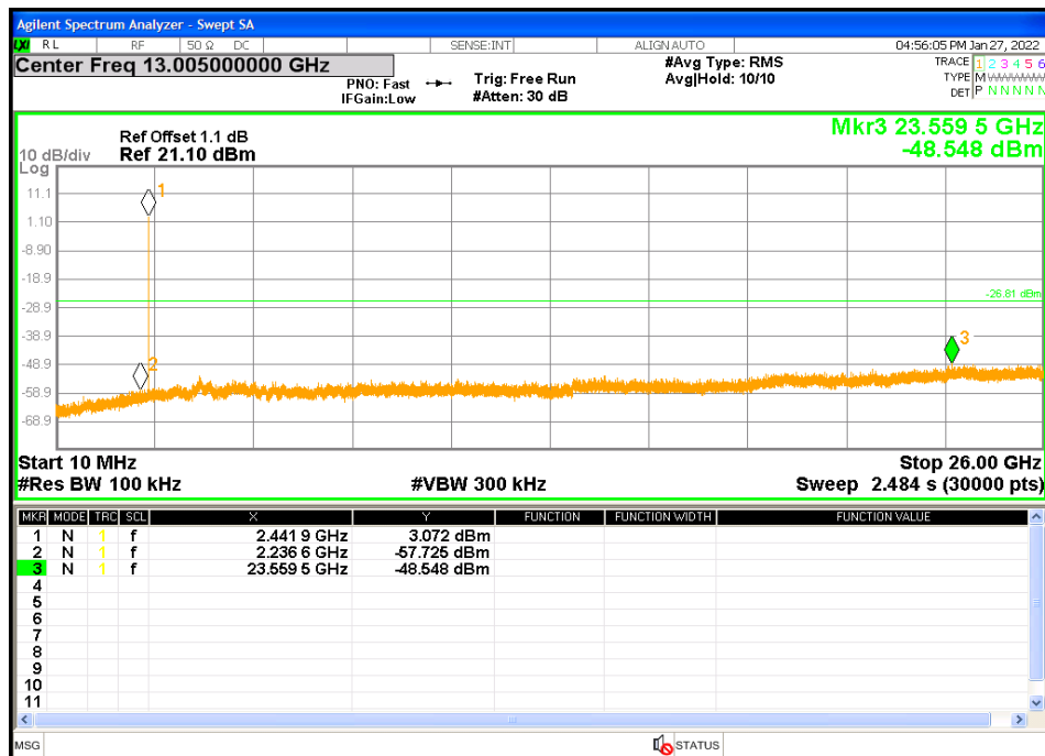
Figure 30: Out of band Emissions at 1 Mbps, 2442 MHz- Transmitter
