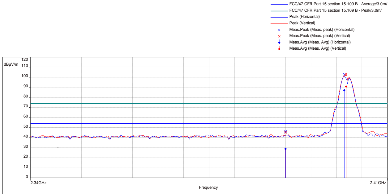
Figure 39: Band-edge-2402 MHz
