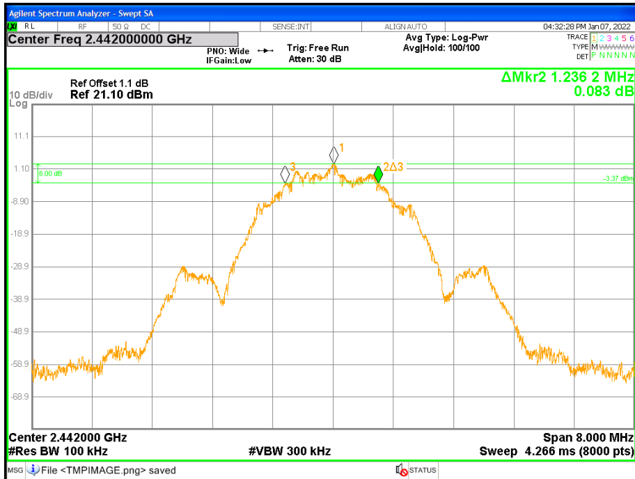
Figure 16: DTS Bandwidth-Headset at 2Mbps - 2442 MHz
