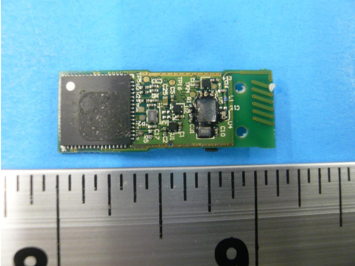
Figure 2: Internal Photo of SYN Pro Air TX - Bottom
