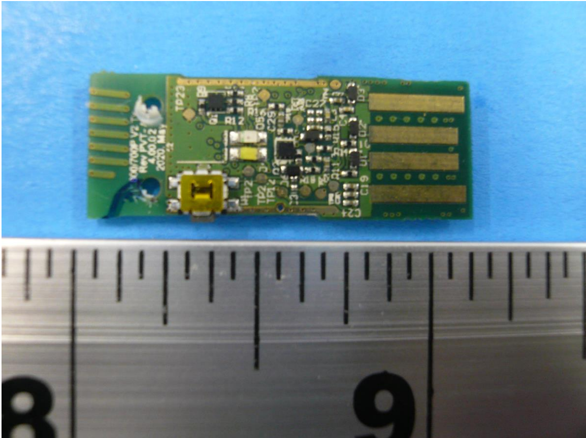
Figure 1: Internal Photo of SYN Pro Air TX - Top
