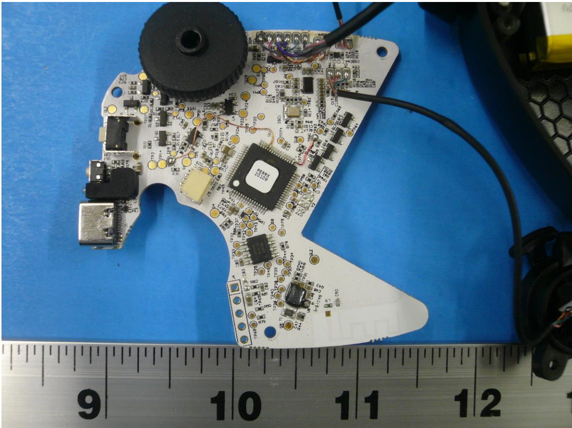
Figure 1: Internal Photo of SYN Pro Air RX – Left Ear PCB (Top)
