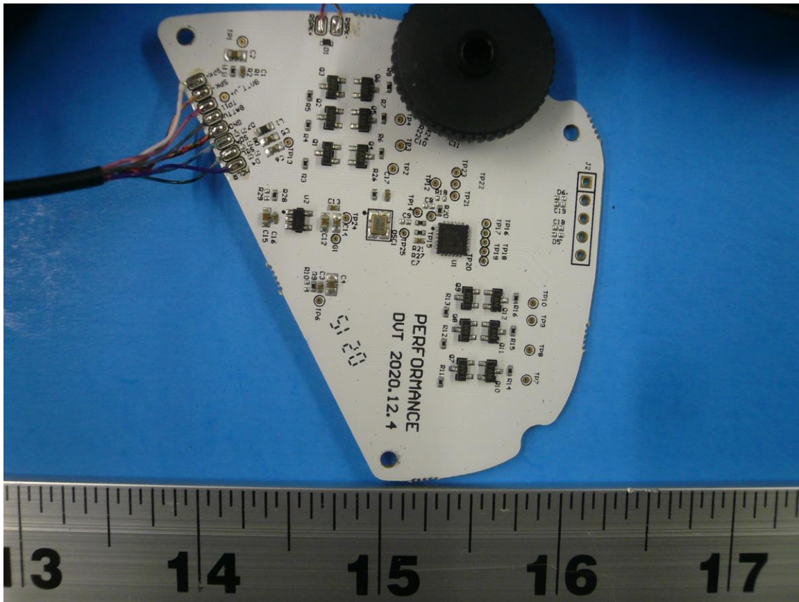
Figure 3: Internal Photo of SYN Pro Air RX – Right Ear (Top)
