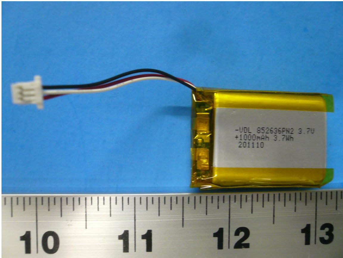
Figure 5: Internal Photo of SYN Pro Air RX – Battery (Top)
