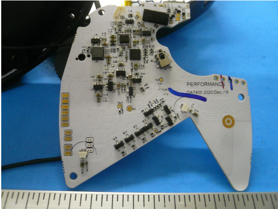
Figure 2: Internal Photo of SYN Pro Air RX – Left Ear PCB (Bottom)
