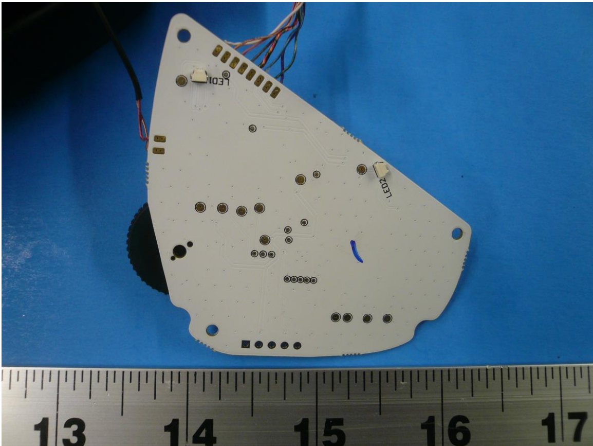
Figure 4: Internal Photo of SYN Pro Air RX – Right Ear (Bottom)
