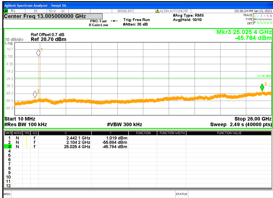
Figure 20: Out of band Emission at 2442 MHz-Headset
