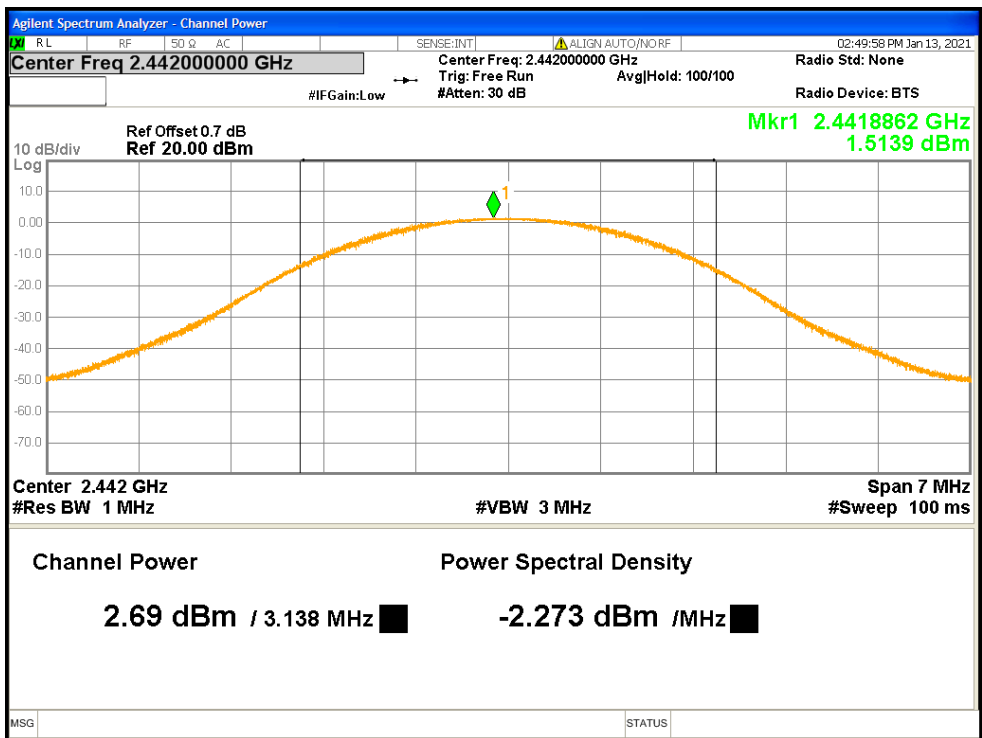
Figure 6: Maximum Conducted Output Power at 2442 MHz at 2Mbps - Headset
