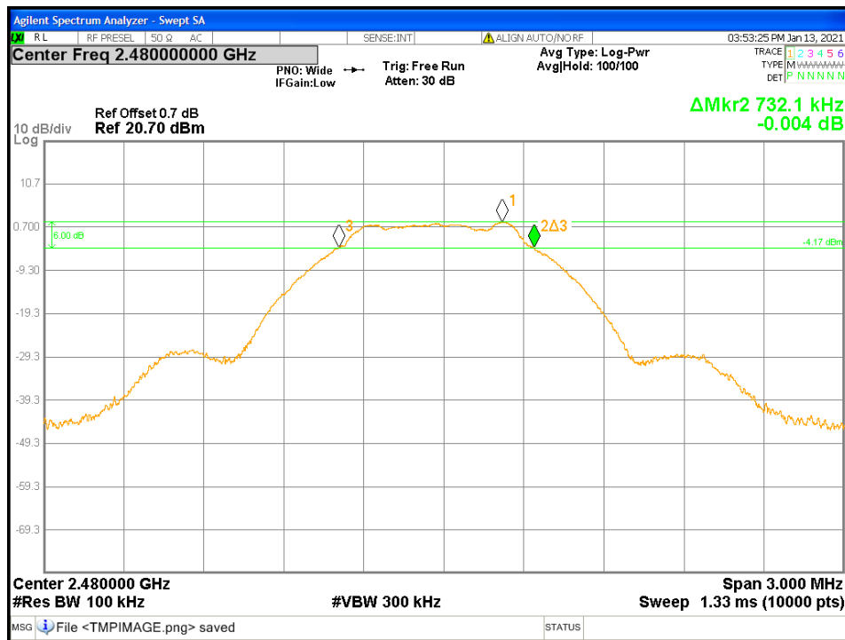
Figure 10: DTS Bandwidth-Headset -2480 MHz
