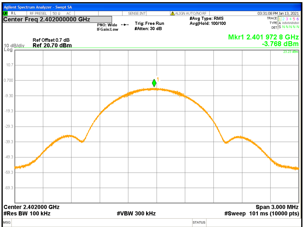
Figure 14: Maximum Power Spectral Density-2402 MHz-Headset
