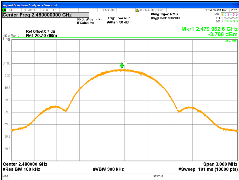
Figure 16: Maximum Power Spectral Density-2480 MHz-Headset
