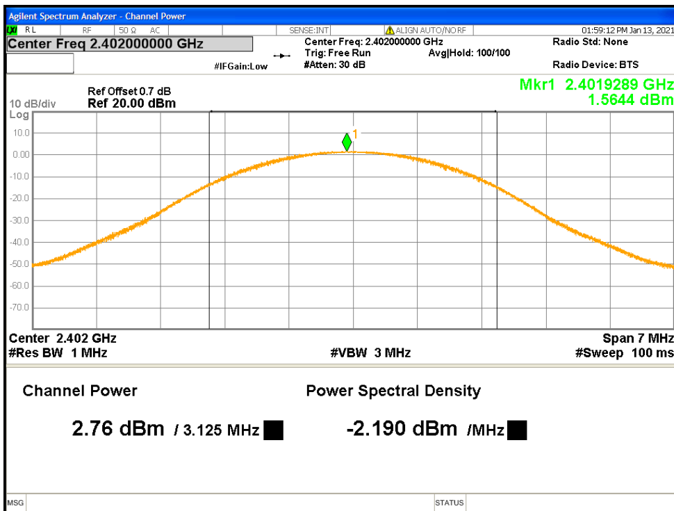
Figure 5: Maximum Conducted Output Power at 2402 MHz at 2Mbps - Headset
