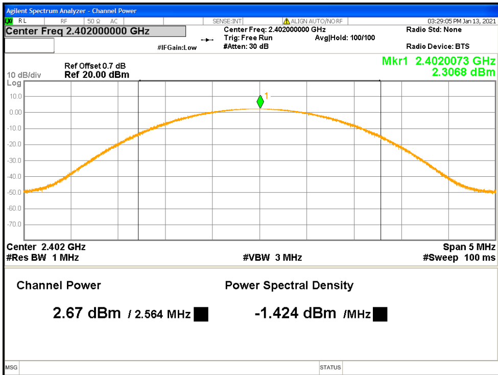
Figure 2: Maximum Transmitted Power, 2402 MHz at 1Mbps - Headset
