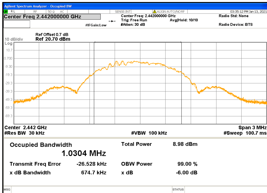
Figure 12: 99% Bandwidth-Headset -2442 MHz
