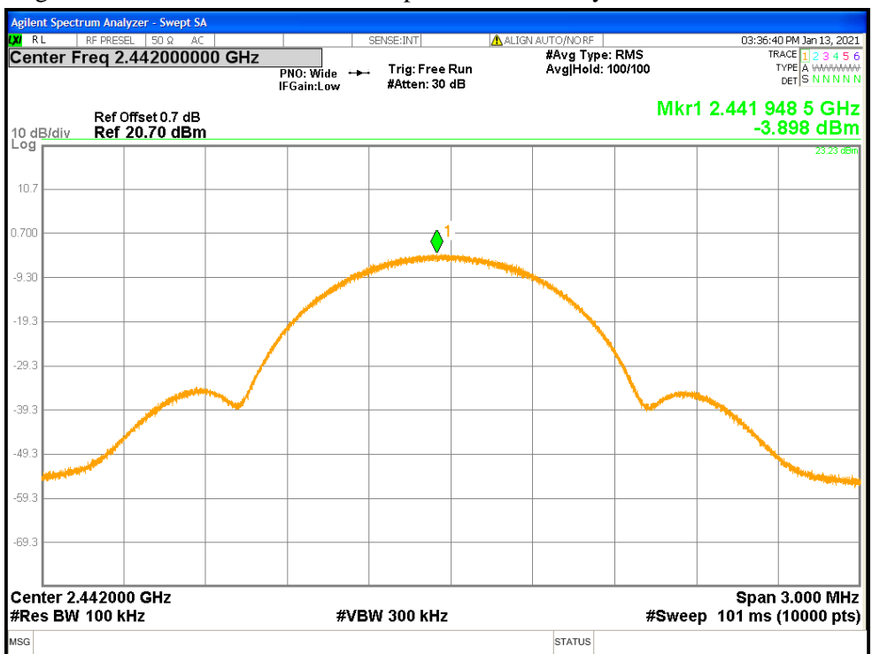
Figure 15: Maximum Power Spectral Density-2442 MHz-Headset
