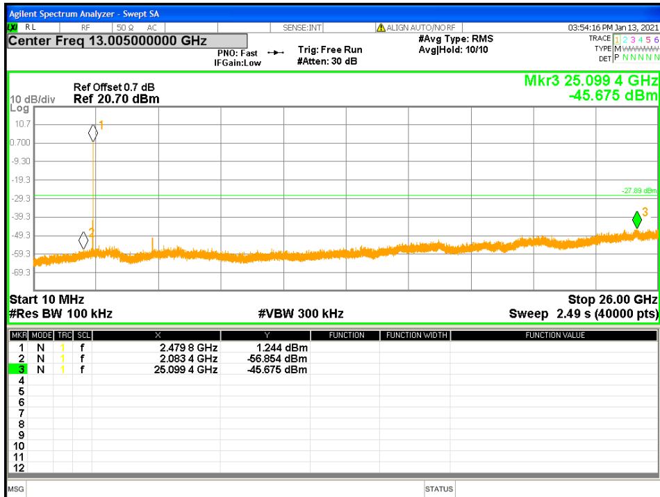
Figure 22: Out of band Emission at 2480 MHz-Headset
