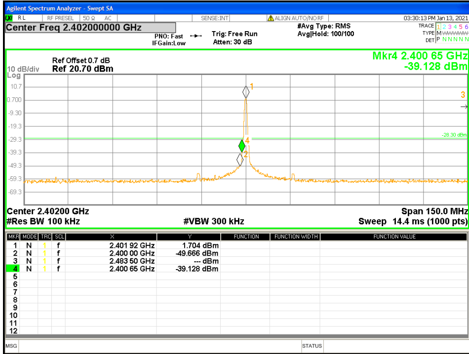
Figure 17: Conducted Band Edge at 2402 MHz-Headset
