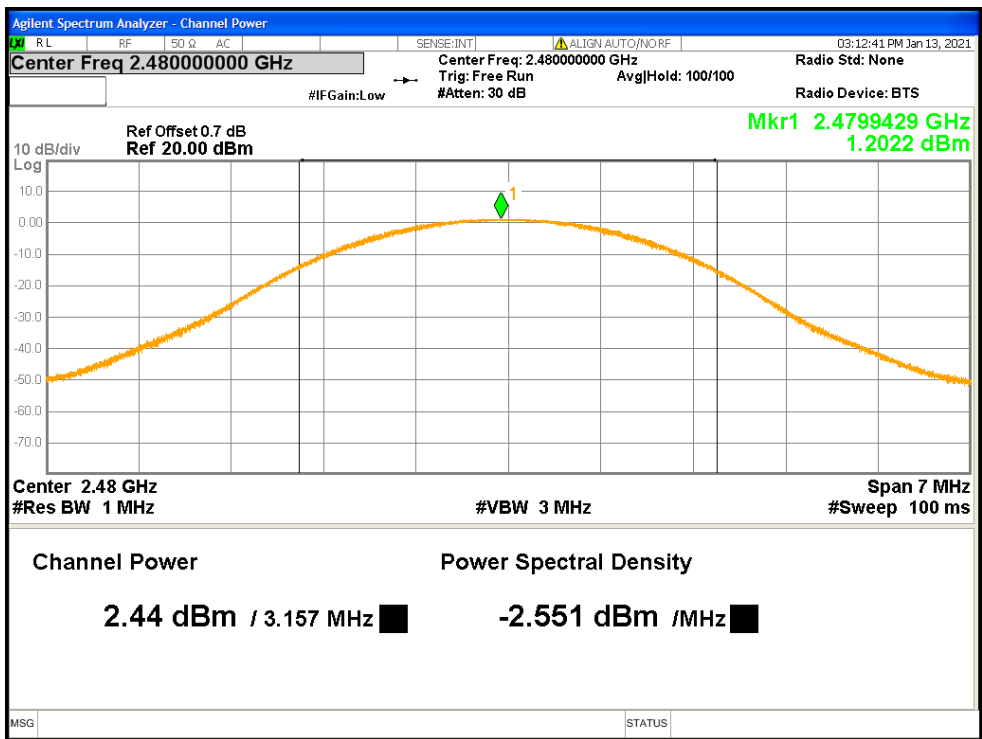
Figure 7: Maximum Conducted Output Power at 2480 MHz at 2Mbps - Headset
