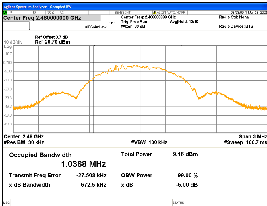
Figure 13: 99% Bandwidth-Headset -2480 MHz
