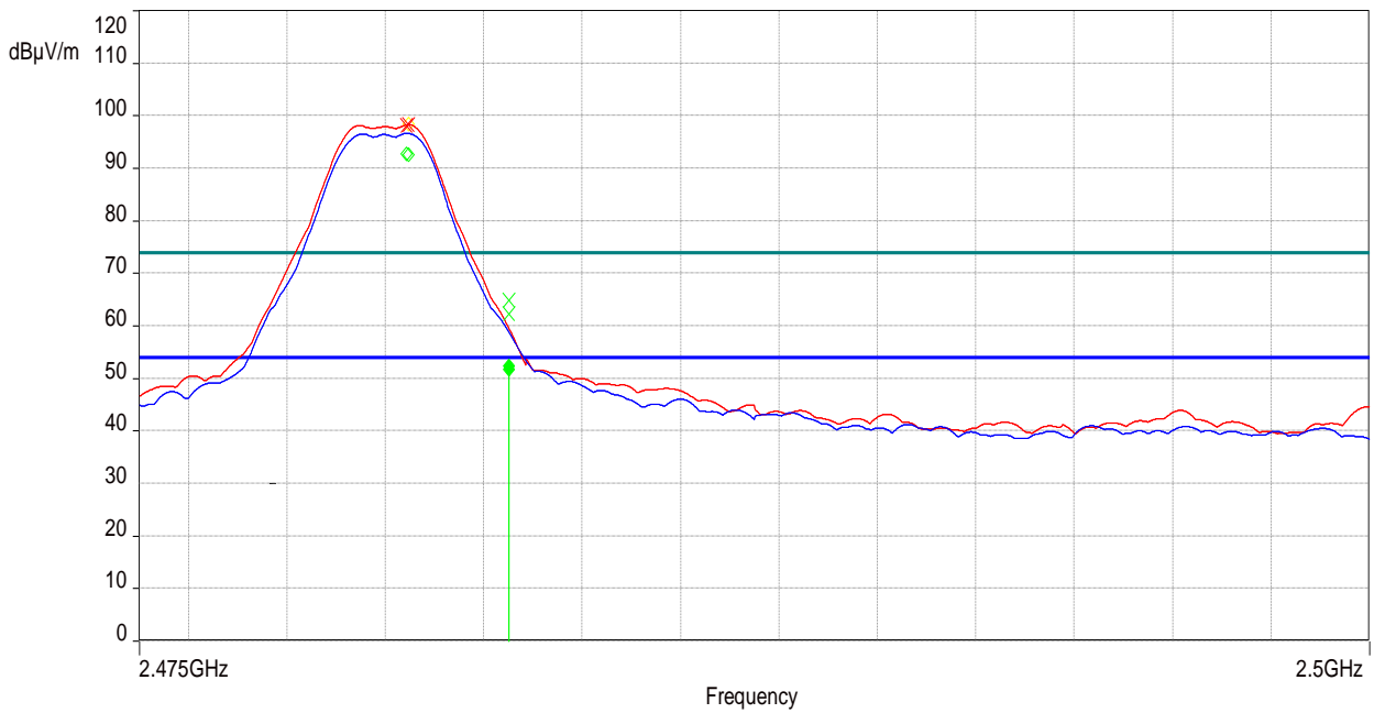
Figure 24: Band-edge-2480 MHz
