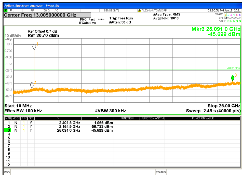
Figure 18: Out of band Emission at 2402 MHz-Headset
