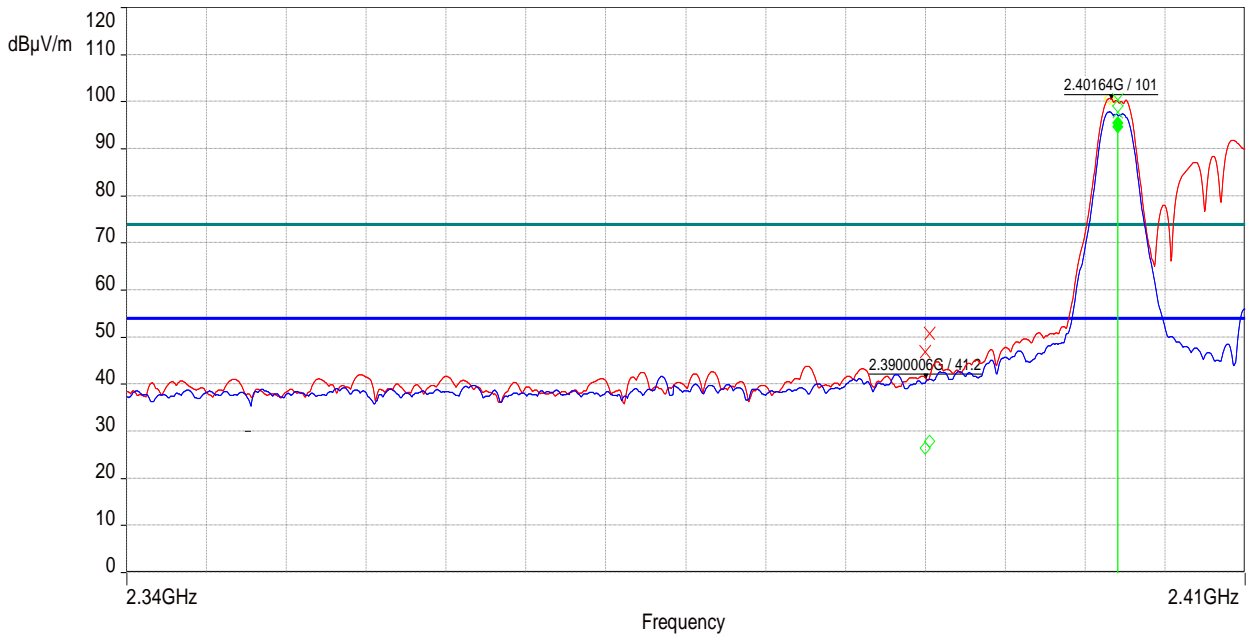
Figure 23: Band-edge-2402 MHz
