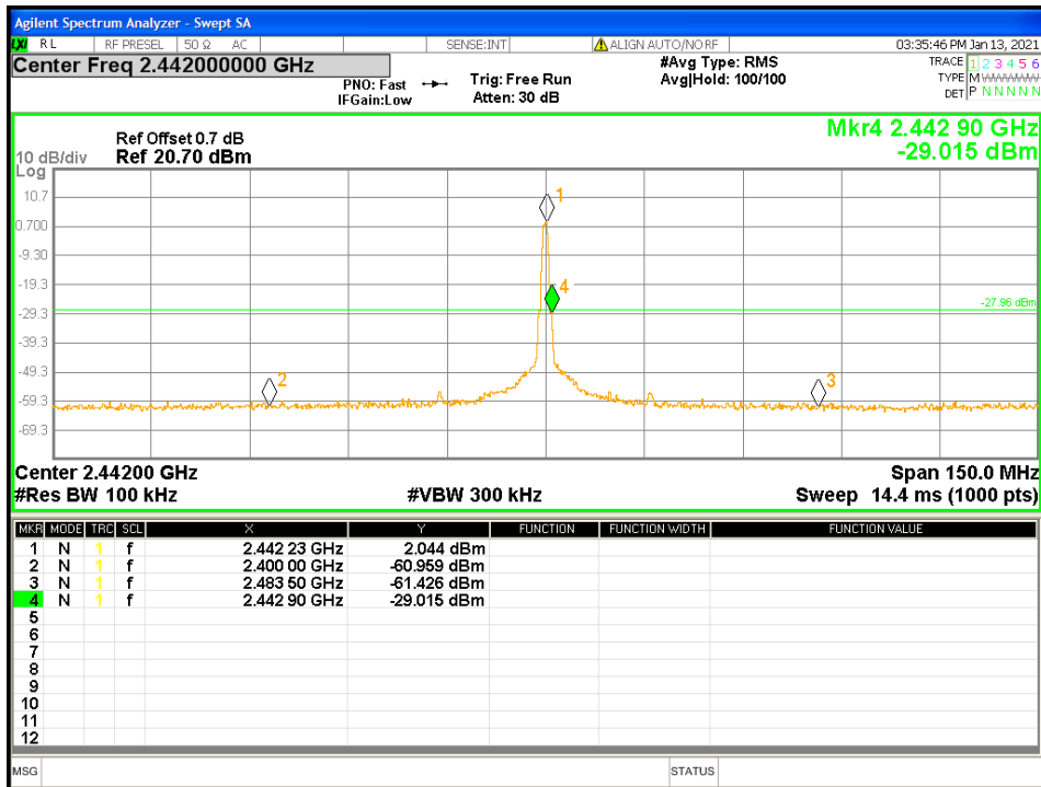
Figure 19: Conducted Band Edge at 2442 MHz-Headset
