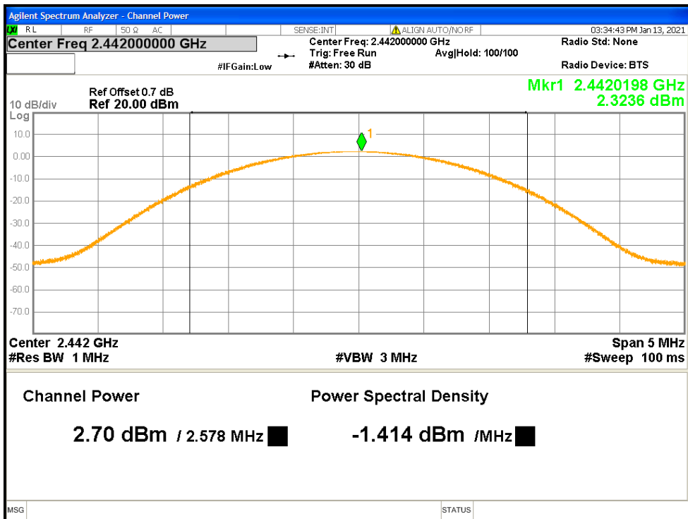
Figure 3: Maximum Conducted Output Power at 2442 MHz at 1Mbps - Headset
