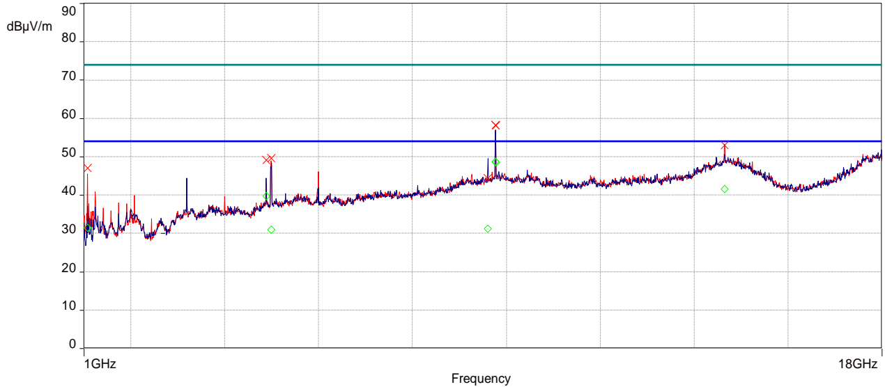
Above 1 GHz Plots for Transmit Mode at 2442 MHz
