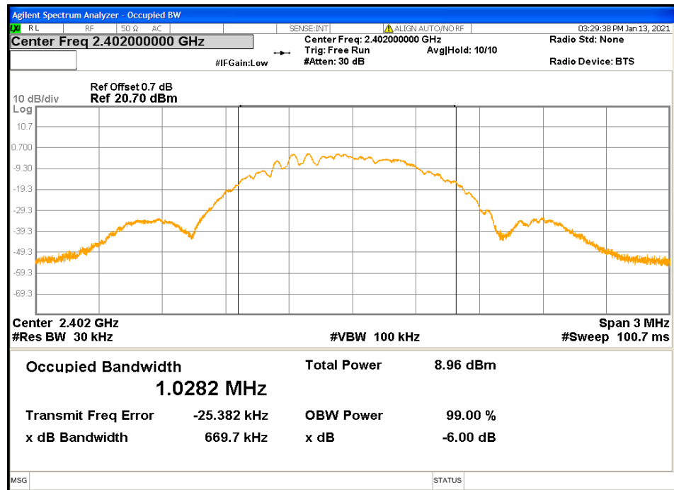
Figure 11: 99% Bandwidth-Headset -2402 MHz
