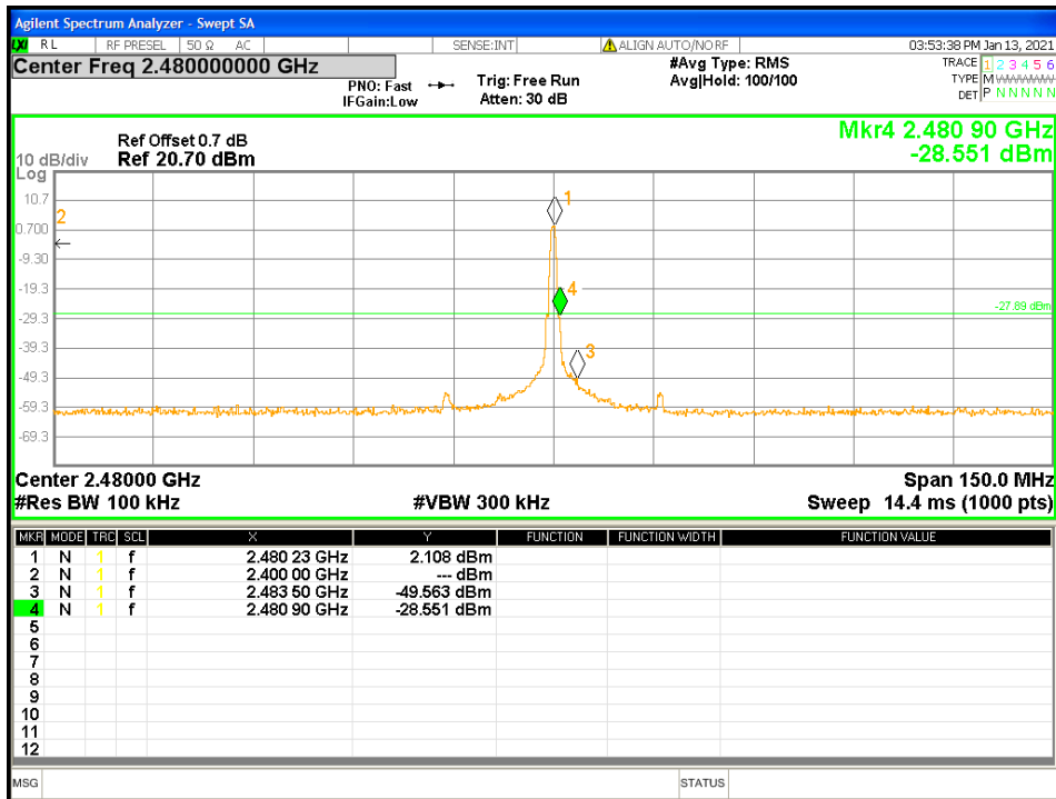
Figure 21: Conducted Band Edge at 2480 MHz-Headset
