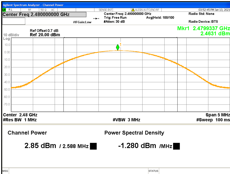
Figure 4: Maximum Conducted Output Power at 2480 MHz at 1Mbps - Headset
