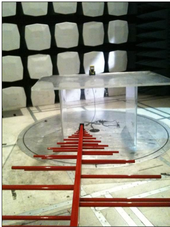
Photograph 3. Radiated Emission, Test Setup, Programming Mode, 2
