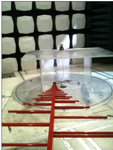
Photograph 5. Radiated Spurious Emissions, Test Setup, 2
