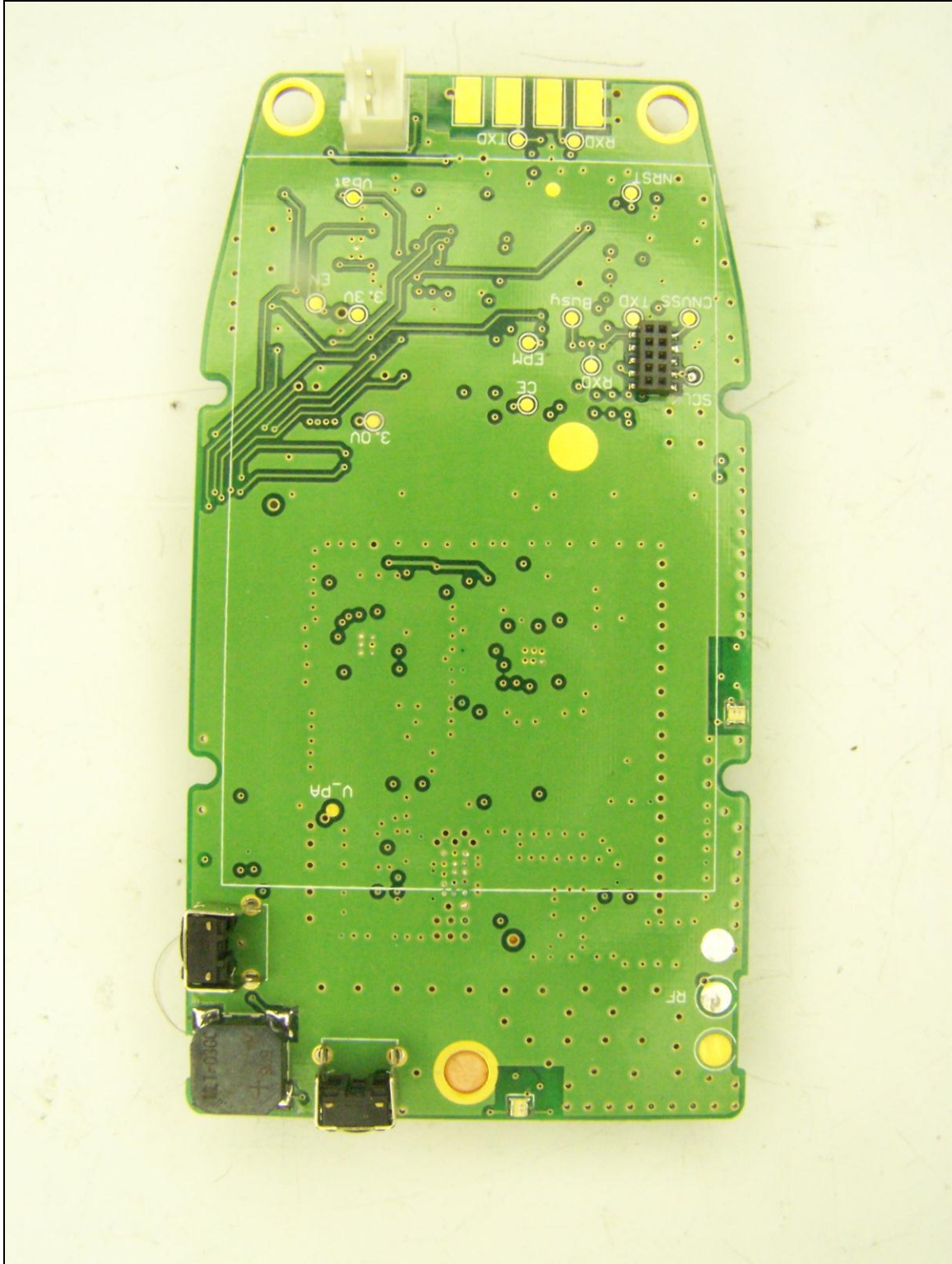
Photograph 3. Board Reverse
