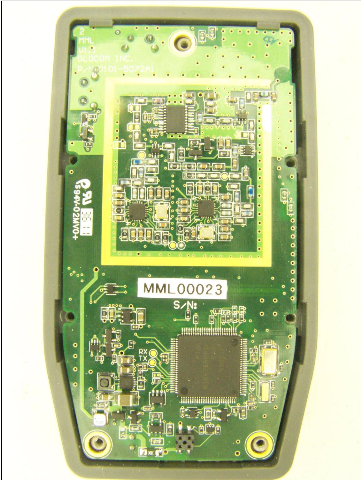
Photograph 6. Internal Full Board View
