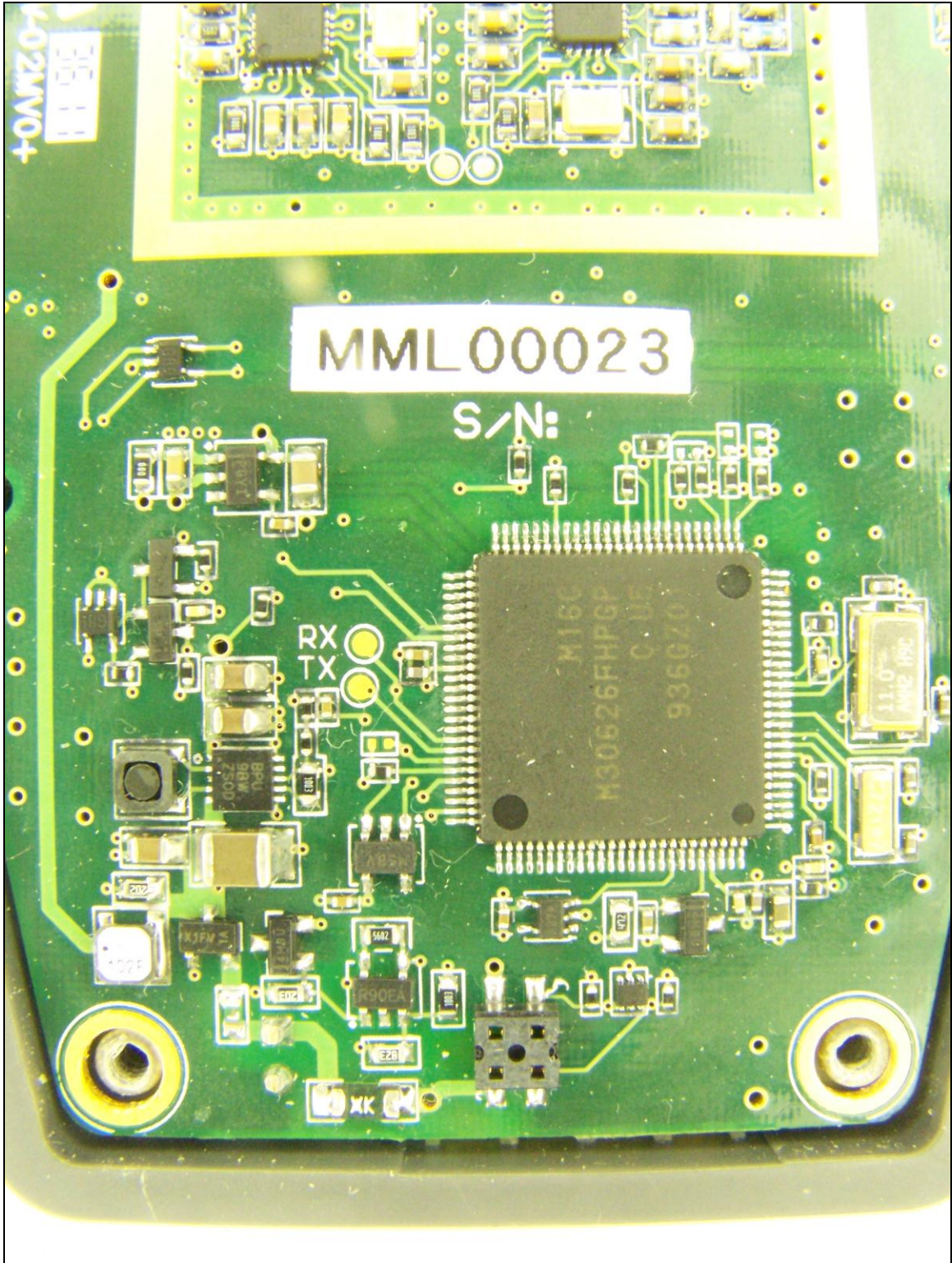
Photograph 5. Internal Components 2
