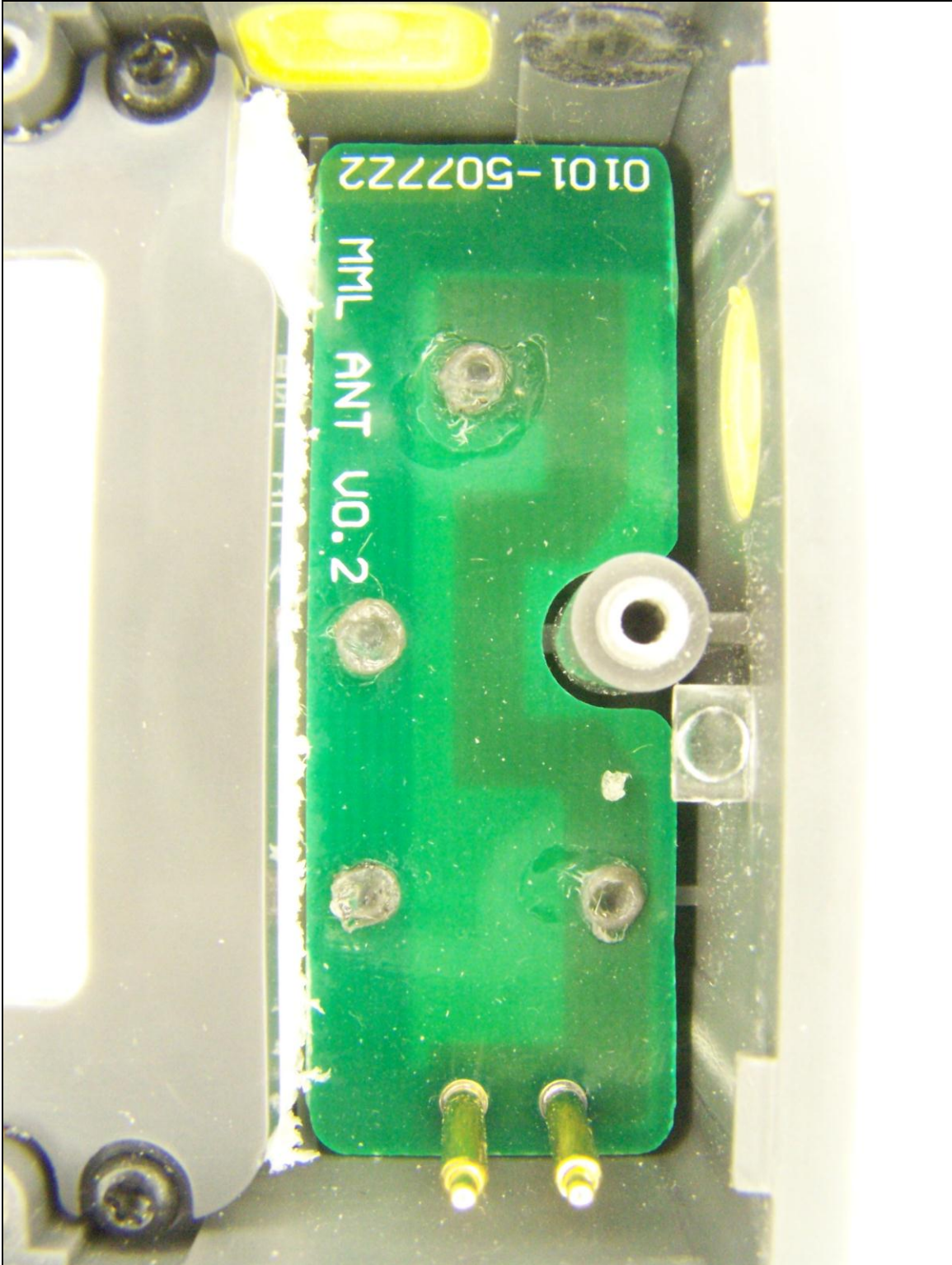
Photograph 1. Antenna
