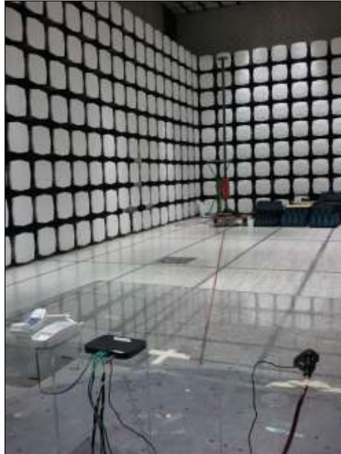
Photograph 3. Radiated Emission, Test Setup, 30 MHz – 1 GHz, Schmidt
