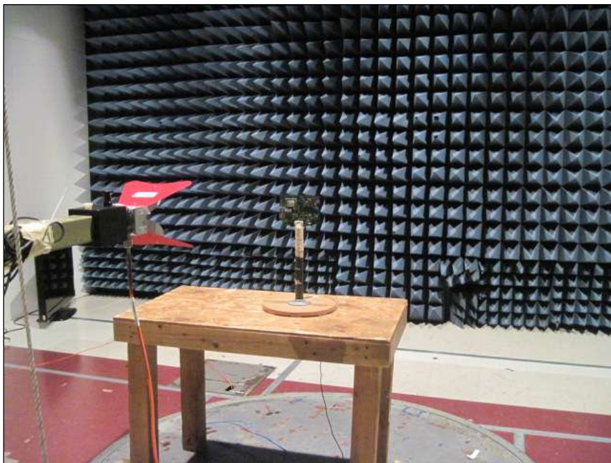
Photograph 10. Radiated Spurious Emissions, 1 GHz – 18 GHz
