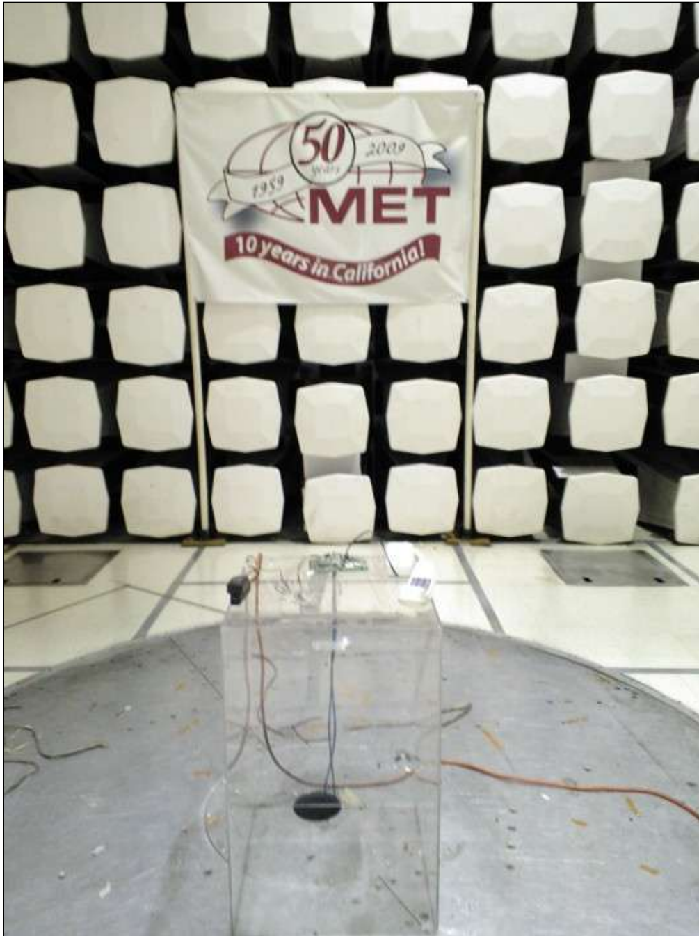
Photograph 7. Radiated Emission, Test Setup
