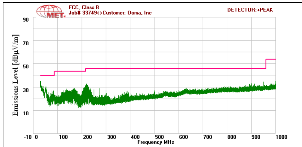
Plot 8. Radiated Spurious Emissions, Low Channel, 30 MHz – 1 GHz
