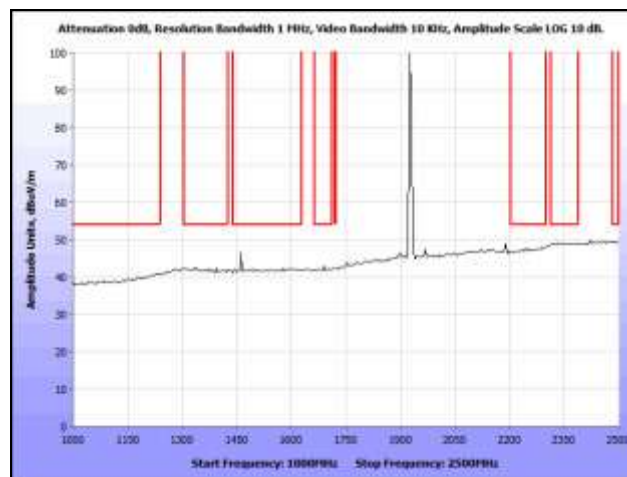
Plot 16. Radiated Spurious Emissions, Mid Channel, 1 GHz – 2.5 GHz, Average
