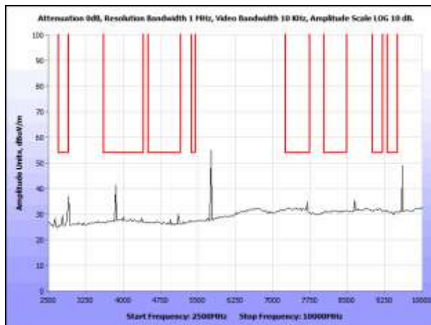
Plot 11. Radiated Spurious Emissions, Low Channel, 2.5 GHz – 10 GHz, Average
