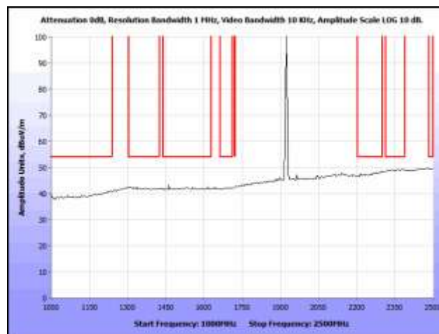
Plot 9. Radiated Spurious Emissions, Low Channel, 1 GHz – 2.5 GHz, Average
