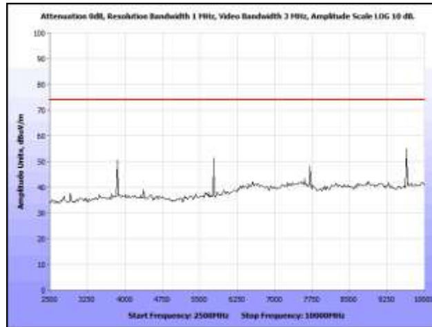
Plot 26. Radiated Spurious Emissions, High Channel, 2.5 GHz – 10 GHz, Peak
