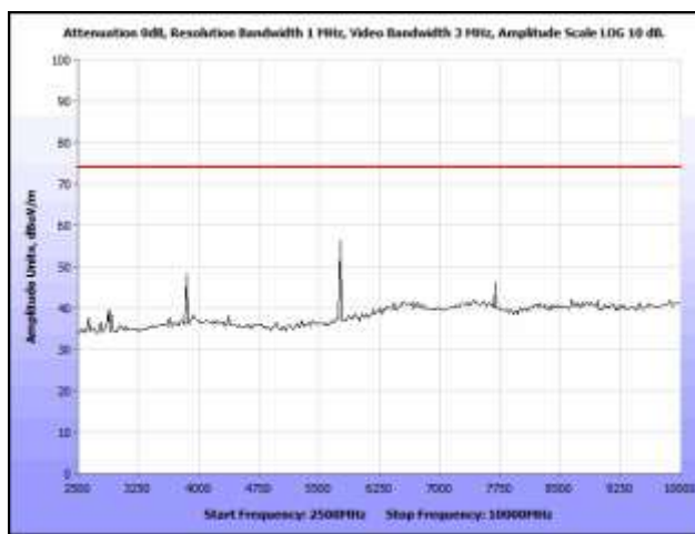
Plot 12. Radiated Spurious Emissions, Low Channel, 2.5 GHz – 10 GHz, Peak
