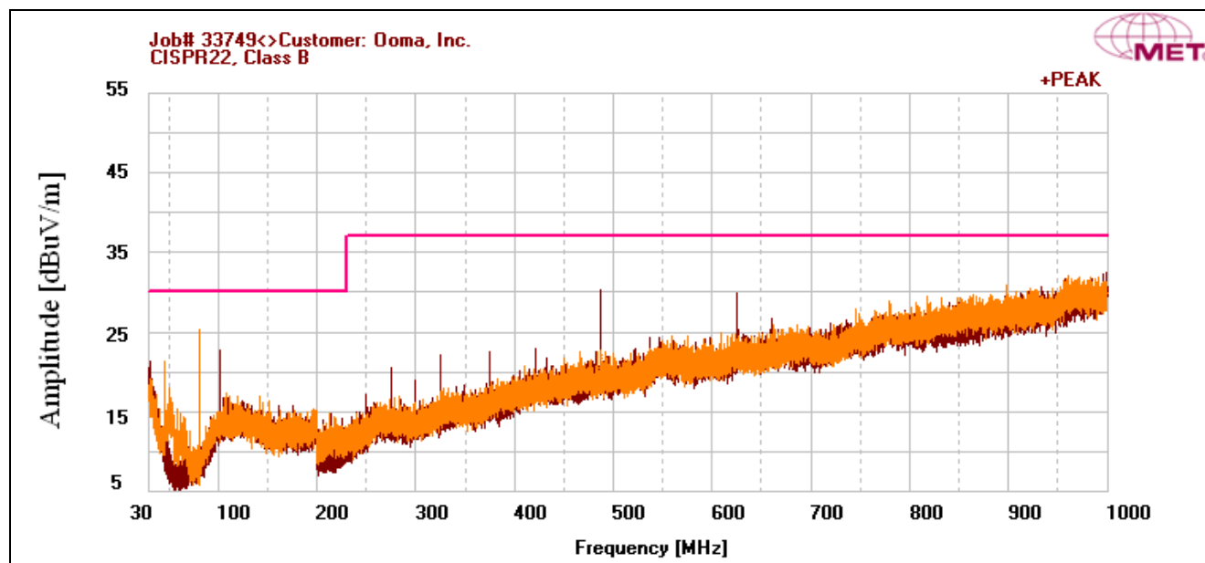
Plot 5. Radiated Emissions Pre-Scan, 30 MHz – 1 GHz, ICES-003 Limits
