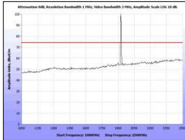
Plot 17. Radiated Spurious Emissions, Mid Channel, 1 GHz – 2.5 GHz, Peak
