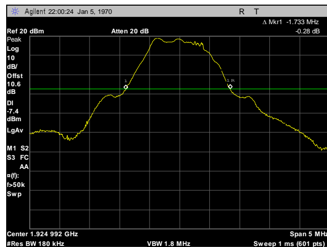
Plot 30. Occupied Bandwidth, Mid Channel
