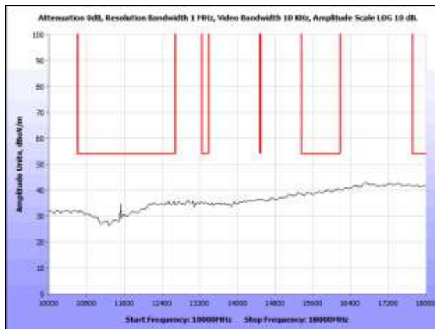
Plot 13. Radiated Spurious Emissions, Low Channel, 10 GHz – 18 GHz, Average
