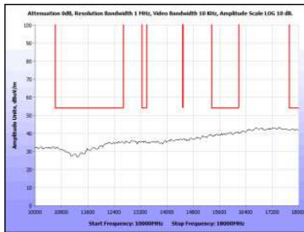
Plot 27. Radiated Spurious Emissions, High Channel, 10 GHz – 18 GHz, Average
