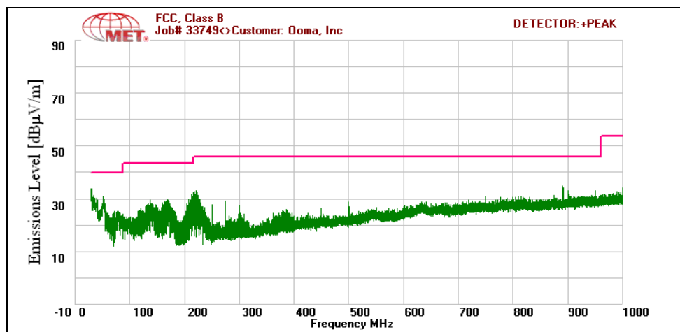
Plot 22. Radiated Spurious Emissions, High Channel, 30 MHz – 1 GHz
