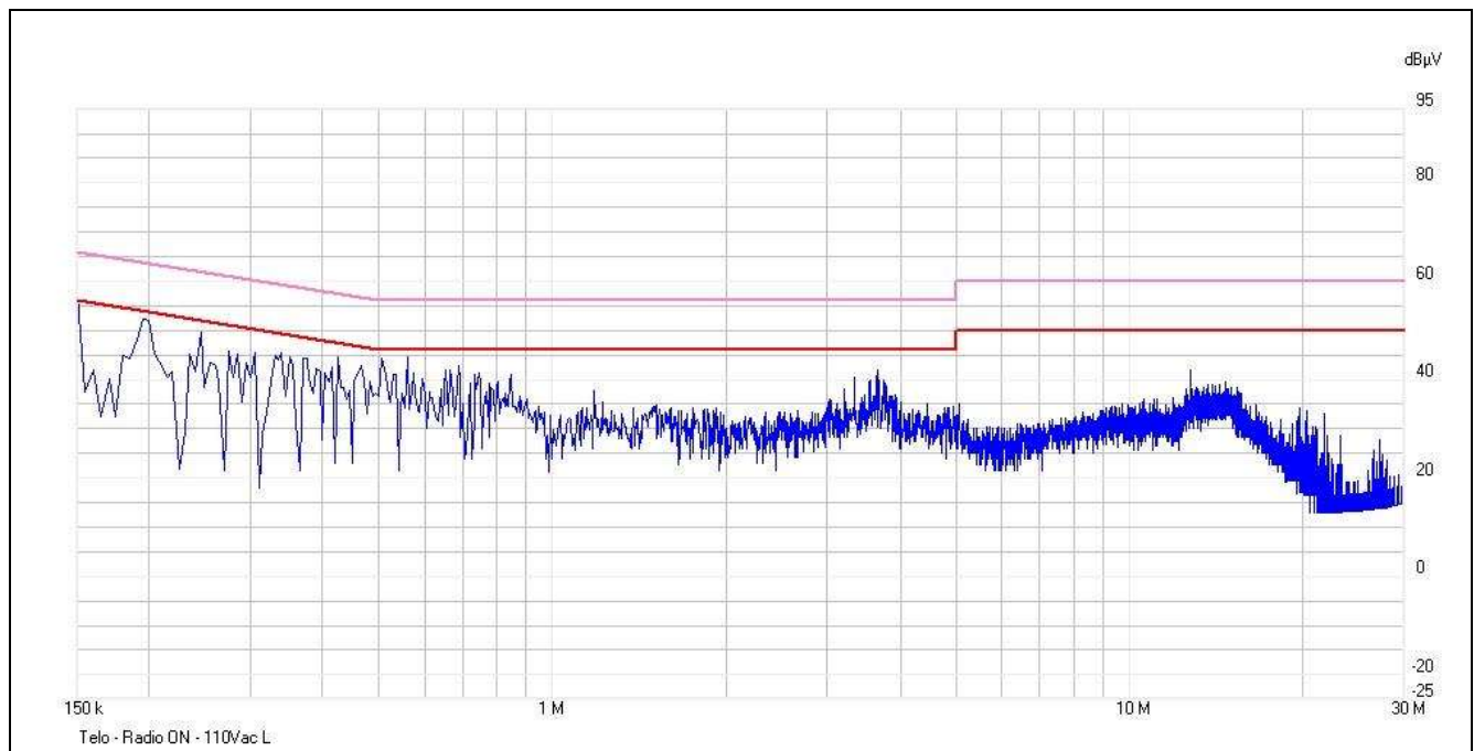
Plot 6. Conducted Emissions, 15.207(a), Phase Line
