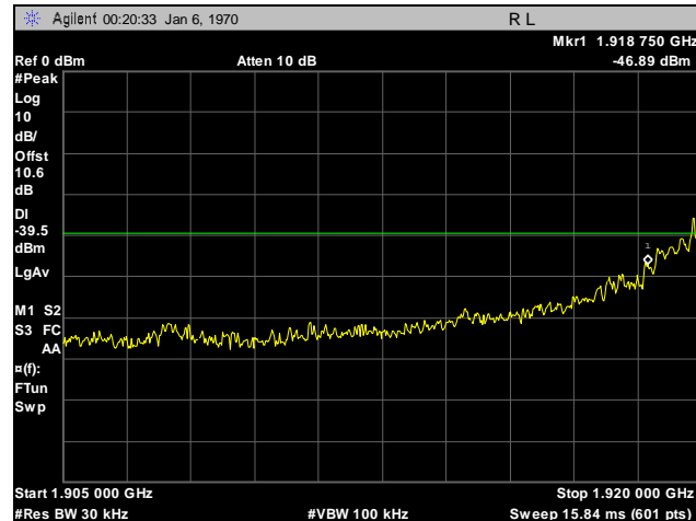
Plot 41. Conducted Spurious Emission, Out-of-Band, Low Channel
