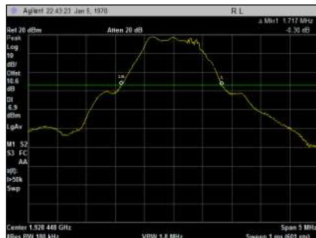
Plot 31. Occupied Bandwidth, High Channel
