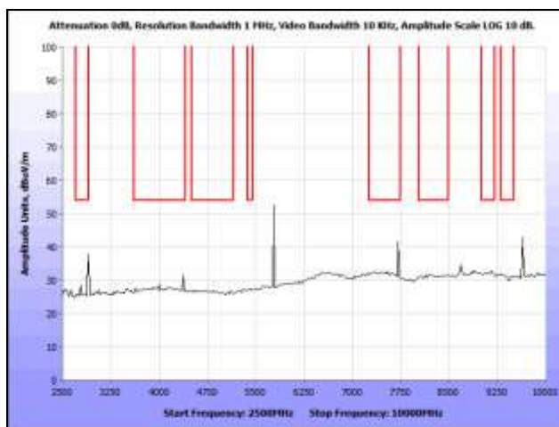
Plot 25. Radiated Spurious Emissions, High Channel, 2.5 GHz – 10 GHz, Average
