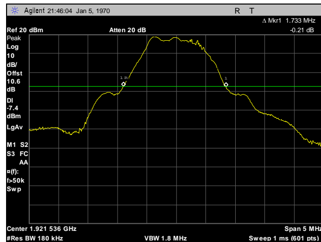
Plot 29. Occupied Bandwidth, Low Channel
