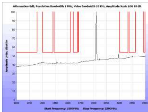
Plot 23. Radiated Spurious Emissions, High Channel, 1 GHz – 2.5 GHz, Average
