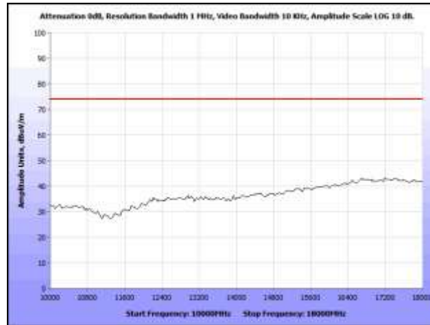
Plot 20. Radiated Spurious Emissions, Mid Channel, 10 GHz – 18 GHz, Average
