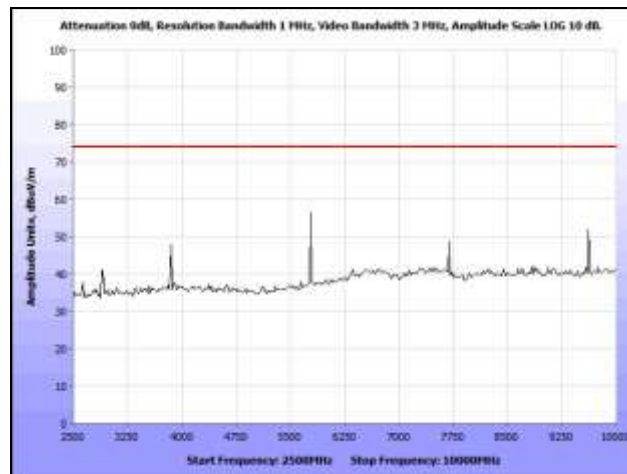
Plot 19. Radiated Spurious Emissions, Mid Channel, 2.5 GHz – 10 GHz, Peak
