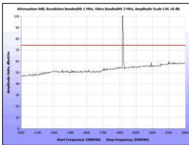
Plot 24. Radiated Spurious Emissions, High Channel, 1 GHz – 2.5 GHz, Peak
