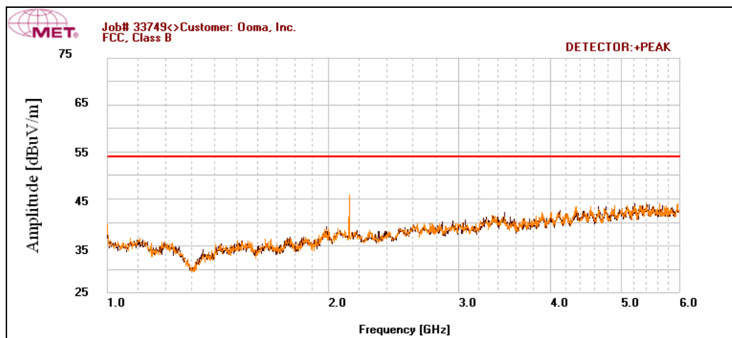
Plot 4. Radiated Emissions Pre-Scan, 1 GHz – 6 GHz, FCC Limits
