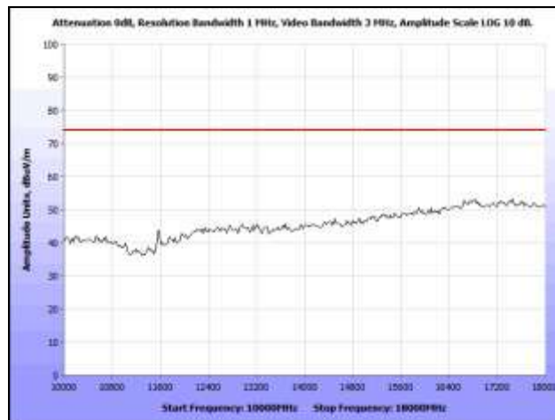
Plot 28. Radiated Spurious Emissions, High Channel, 10 GHz – 18 GHz, Peak
