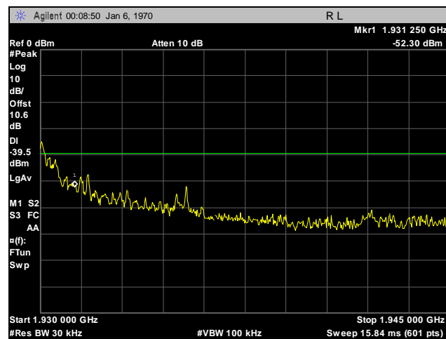
Plot 42. Conducted Spurious Emission, Out-of-Band, High Channel
