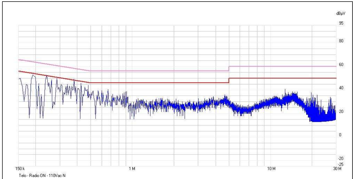
Plot 7. Conducted Emissions, 15.207(a), Neutral Line
