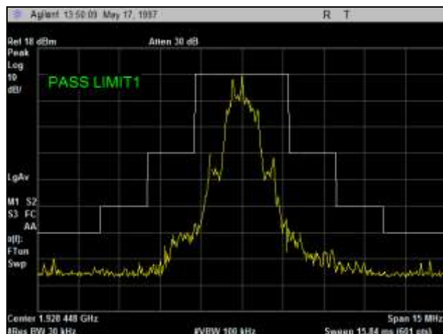
Plot 40. Conducted Spurious Emission, In-Band, High Channel
