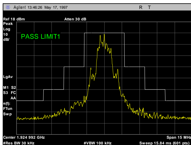
Plot 39. Conducted Spurious Emission, In-Band, Mid Channel
