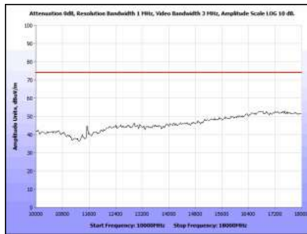
Plot 21. Radiated Spurious Emissions, Mid Channel, 10 GHz – 18 GHz, Peak
