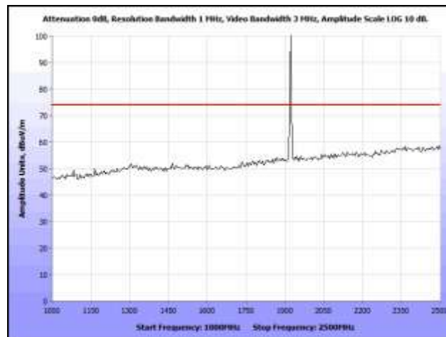
Plot 10. Radiated Spurious Emissions, Low Channel, 1 GHz – 2.5 GHz, Peak
