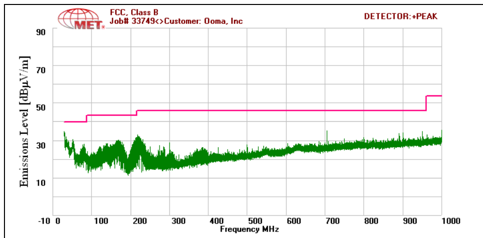
Plot 15. Radiated Spurious Emissions, Mid Channel, 30 MHz – 1 GHz
