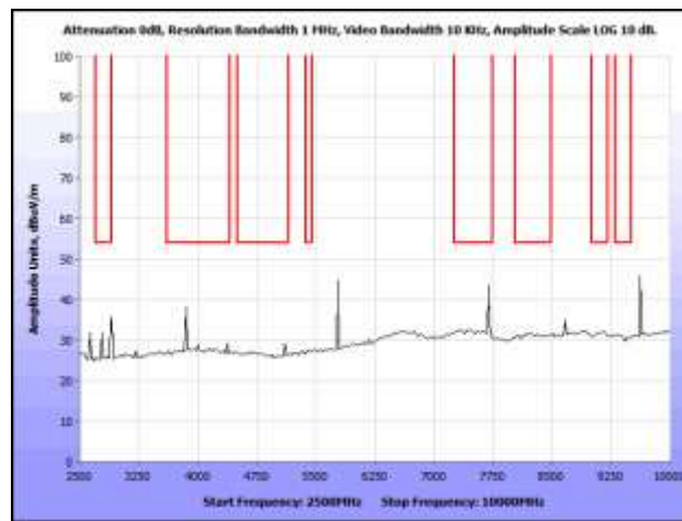
Plot 18. Radiated Spurious Emissions, Mid Channel, 2.5 GHz – 10 GHz, Average
