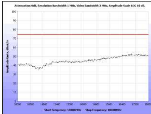
Plot 14. Radiated Spurious Emissions, Low Channel, 10 GHz – 18 GHz, Peak
