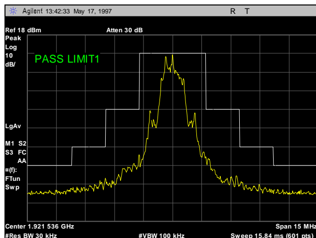
Plot 38. Conducted Spurious Emission, In-Band, Low Channel
