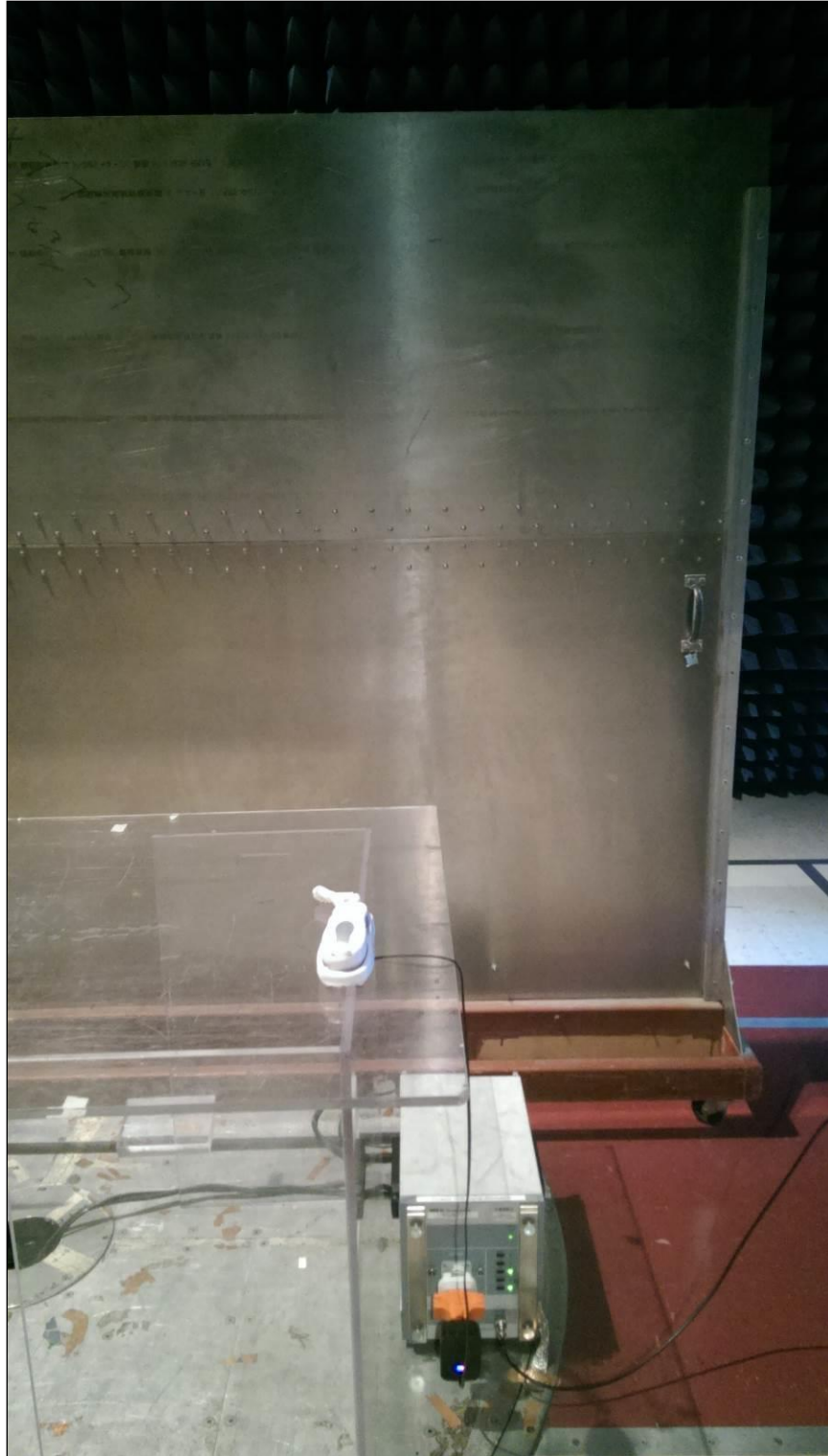
Photograph 1. Conducted Emissions, Test Setup
