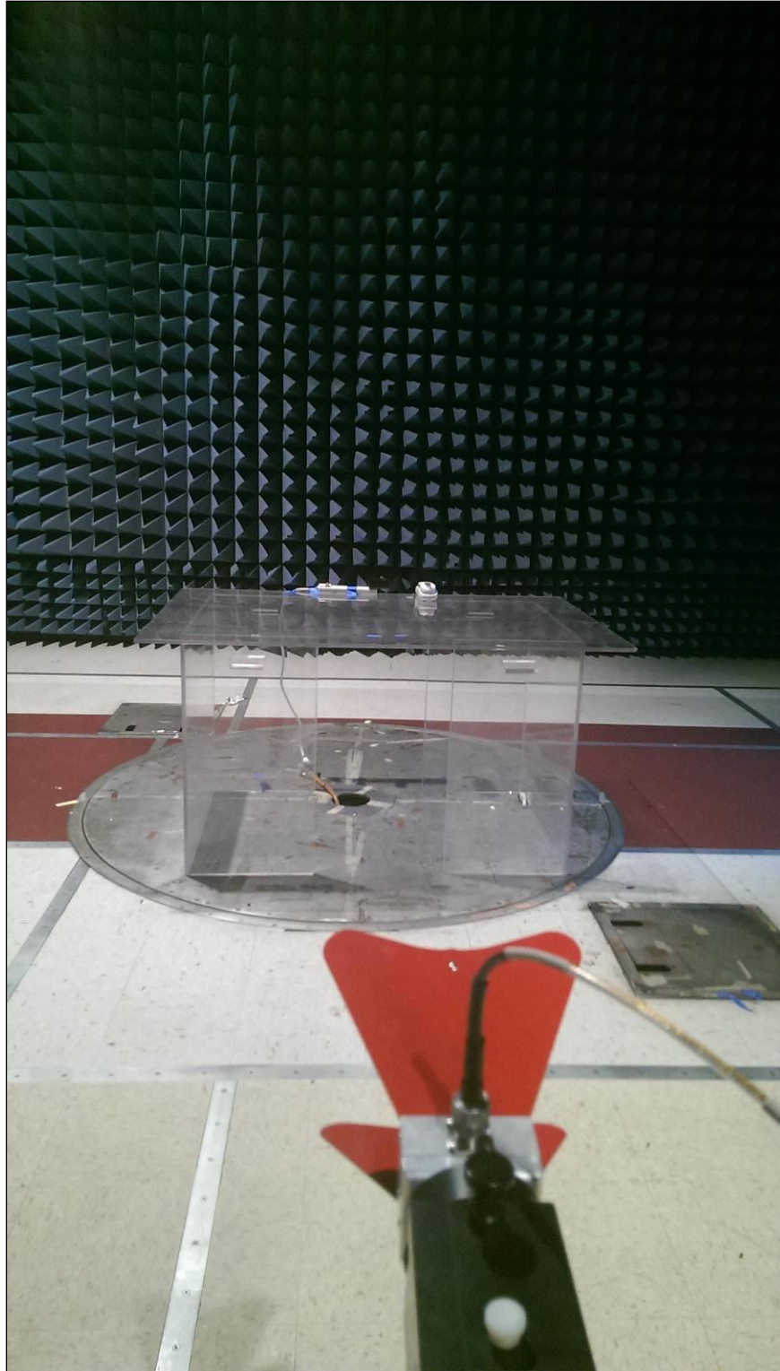
Photograph 3. Radiated Emission, Test Setup, Horn Setup
