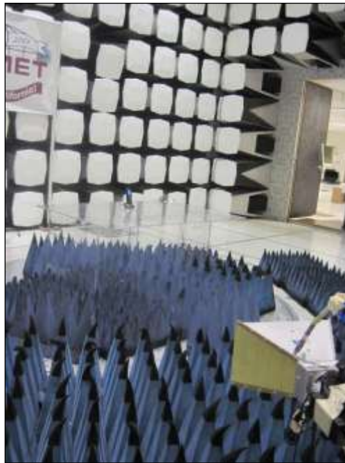
Photograph 4. Radiated Emissions, Test Setup, 1 GHz – 18 GHz
