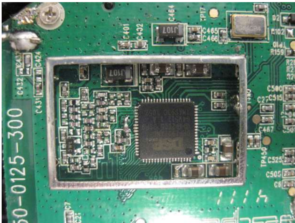
Photograph 3. RF Cover
