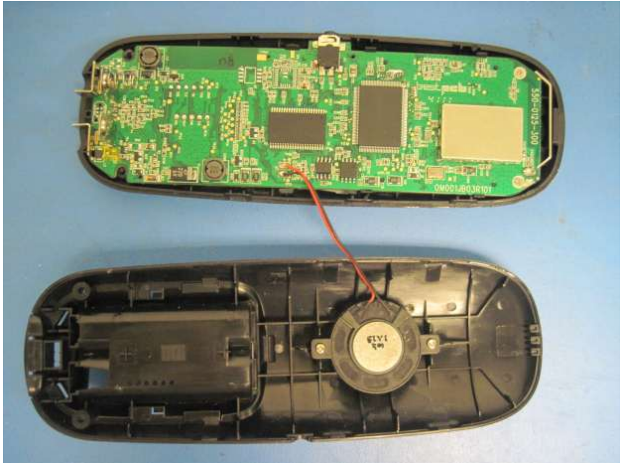
Photograph 4. EUT Open
