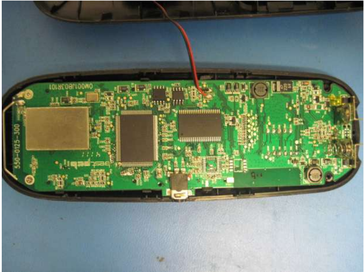
Photograph 1. Board Back
