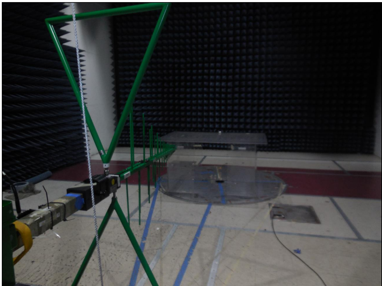
Photograph 1. Radiated Emissions, 30 MHz – 1 GHz, Test Setup
