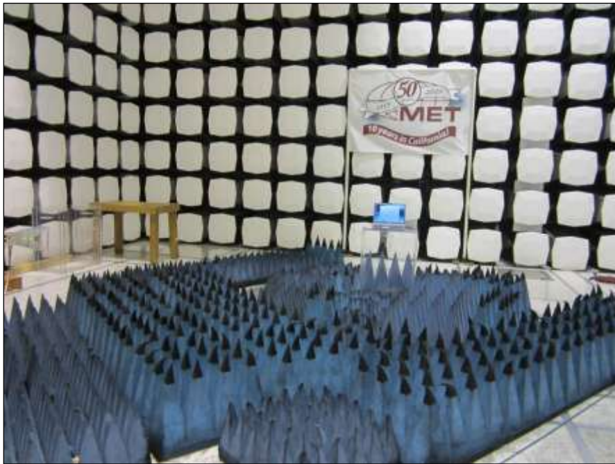
Photograph 3. Radiated Emissions, Test Setup, 1 GHz – 6 GHz
