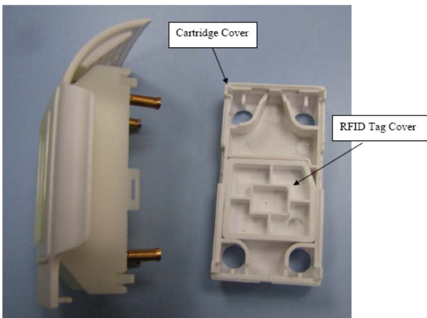
Picture – 2 Cartridge (opened cover)
