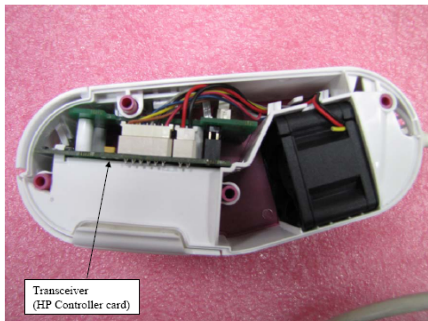
Picture 5 – Handpiece (Transceiver location)
