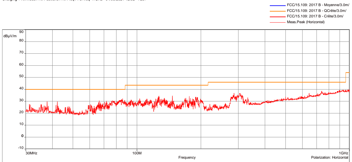
Charging + Rx mode / All Positions / All Freq / For freq <1GHz - 04/09/2021 12:02 - 7267
