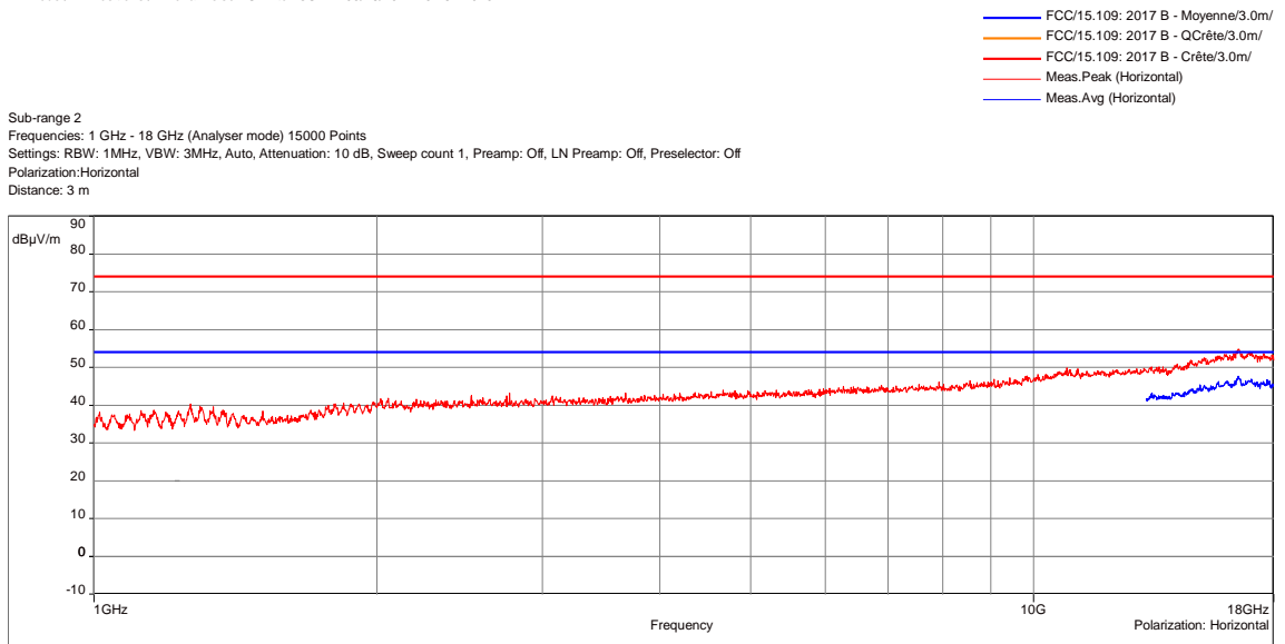
Rx mode / All Positions / All channels / 1GHz to 18GHz - 03/26/2021 13:26 - 7073
