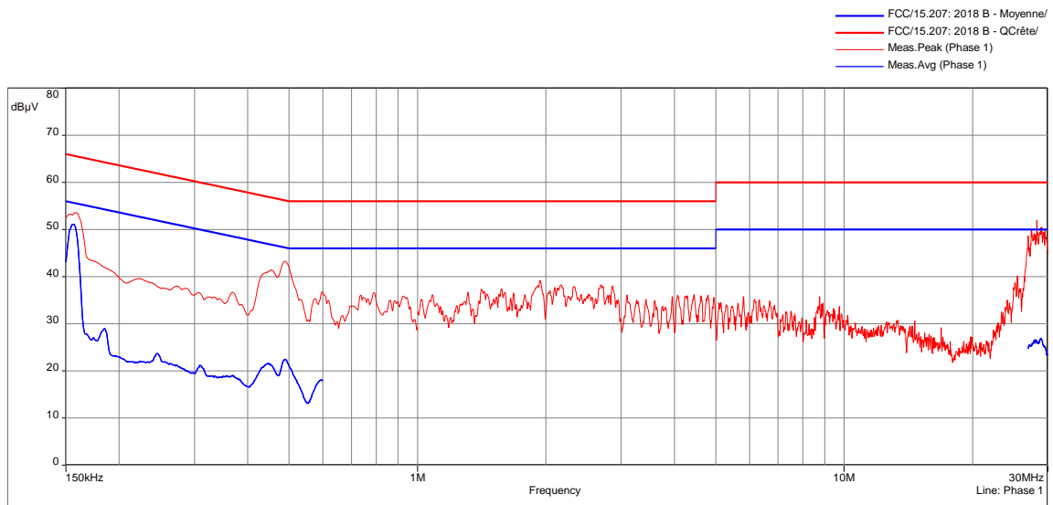
120Vac/60Hz power supply / Charging mode - 05/05/2021 09:44 - 7580
