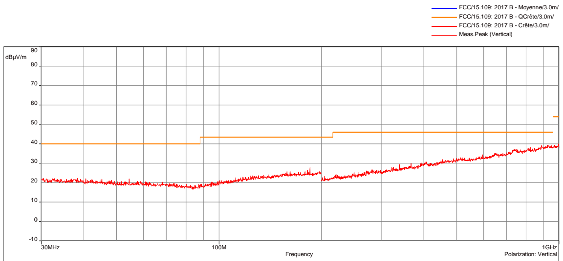
Rx mode / All Positions / All Freq / For freq <1GHz - 04/09/2021 10:56 - 7266
