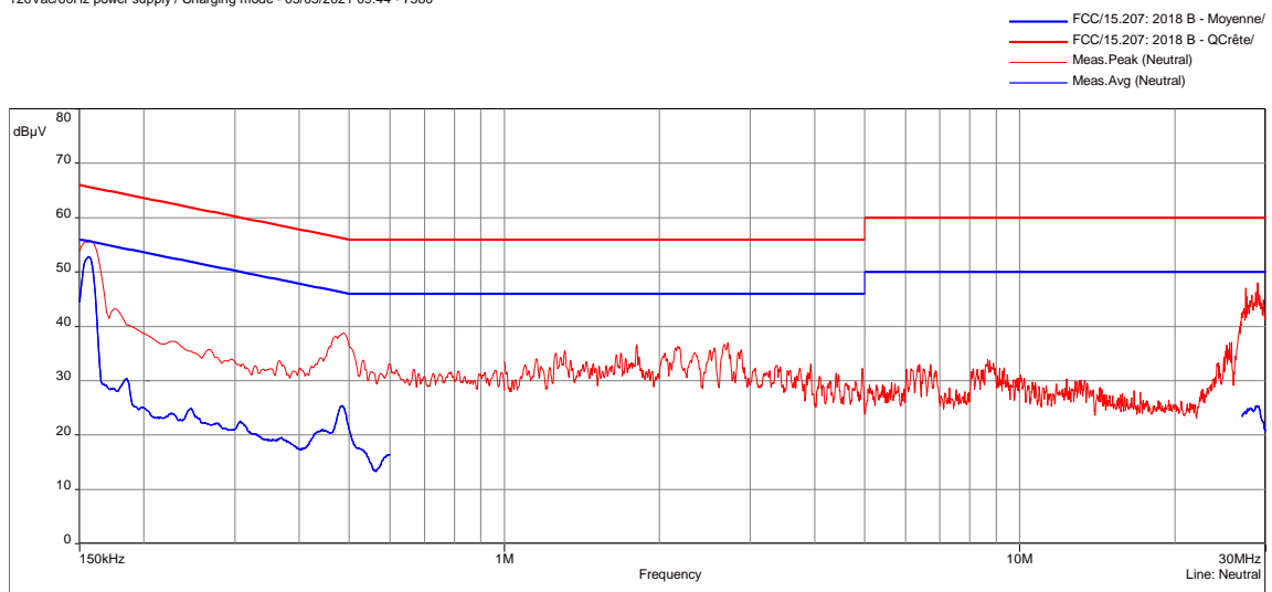
120Vac/60Hz power supply / Charging mode - 05/05/2021 09:44 - 7580
