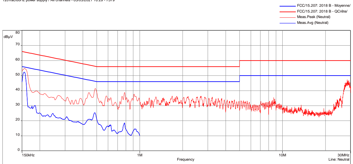
120Vac/60Hz power supply / All channels - 05/05/2021 10:29 - 7579
